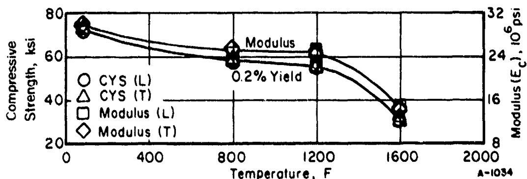
FIGURE 53. EFFECT OF TEMPERATURE ON THE COMPRESSIVE PROPERTIES OF INCONEL 625 SHEET
