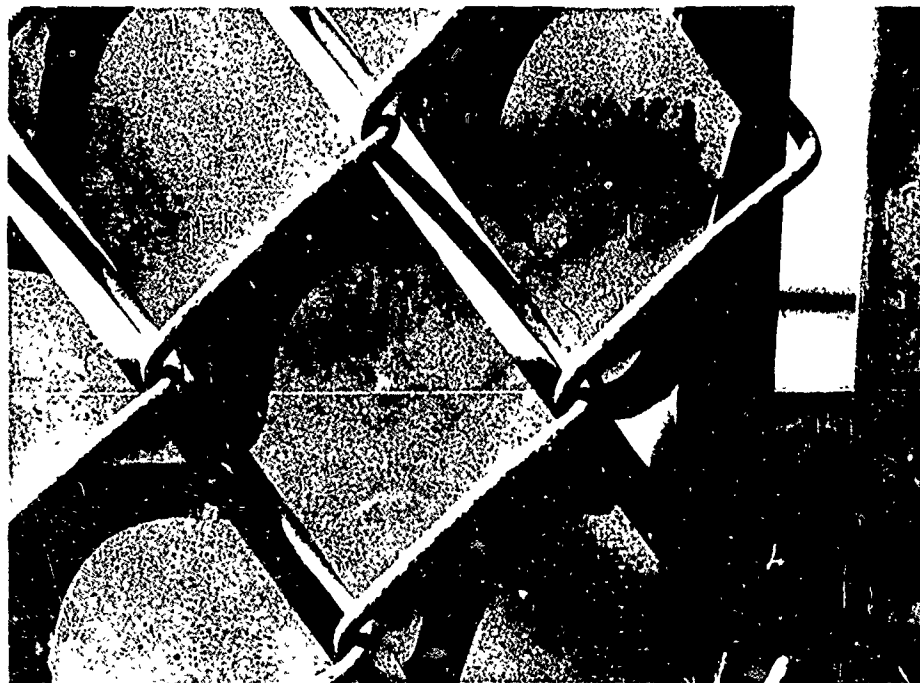
Figure 15. Newly installed anodized aluminum slats on zinc-coated wire.
