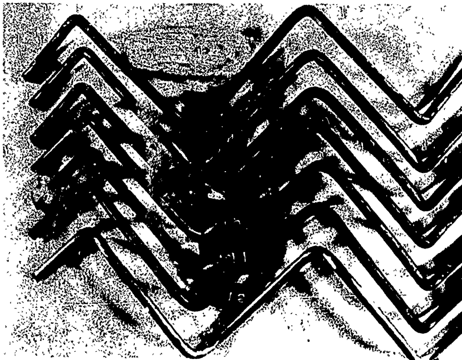
Figure 36. System 15. Corrosion product removed after 2 to 4 months of salt-spray test.
