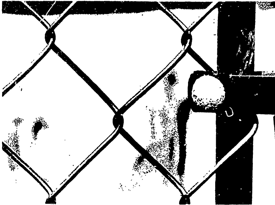
Figure 14. System 9. Stainless steel after 3 years of exposure.
