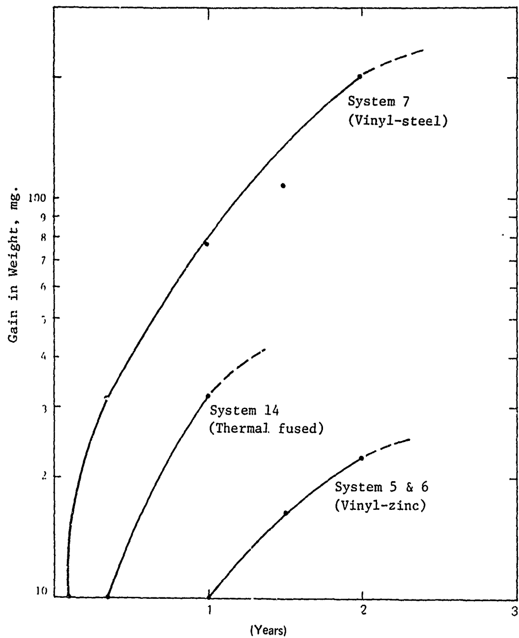
Figure 33. Corrosion patterns of vinyl-coated fence wires in atmosphere.
