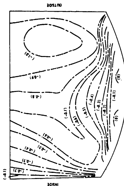
\mu = 0.3 E_1 = 5.0 \times 10^6 \text{ psi} Model G26
