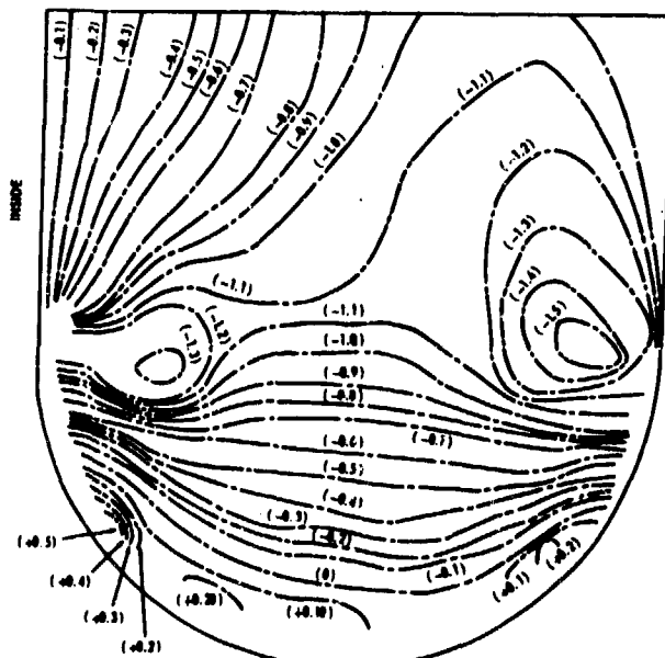
P_1 = 0.3 E_1 = 5 \times 10^6 \text{ psi} Model G37
