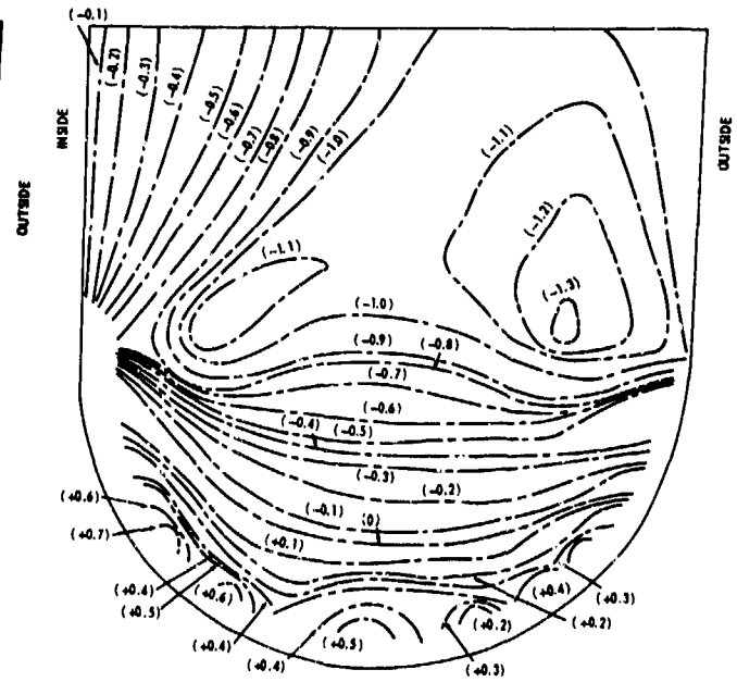
P_1 = 0.3 E_1 = 50.0 \times 10^6 \text{ psi} Model G36
