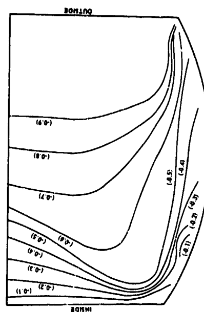
E_1 = 5 \times 10^6 \mu = 0.3 \nu_1 = 0.04 Model G28
