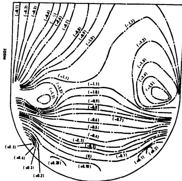
P_1 = 0.3 E_1 = 5 \times 10^6 \text{ psi} Model G35
