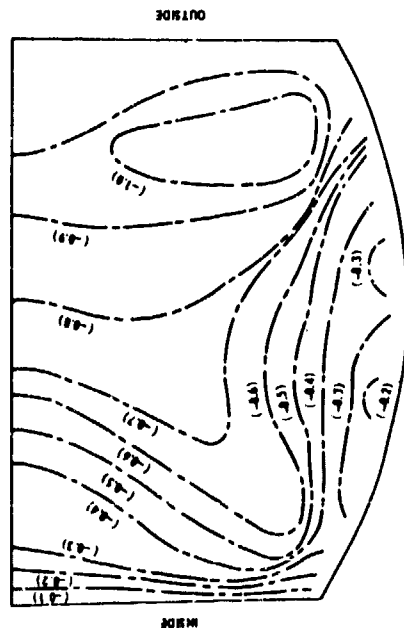
\mu = 0.3 E_1 = 5.11 \times 10^6 \text{ psi} Model G25
