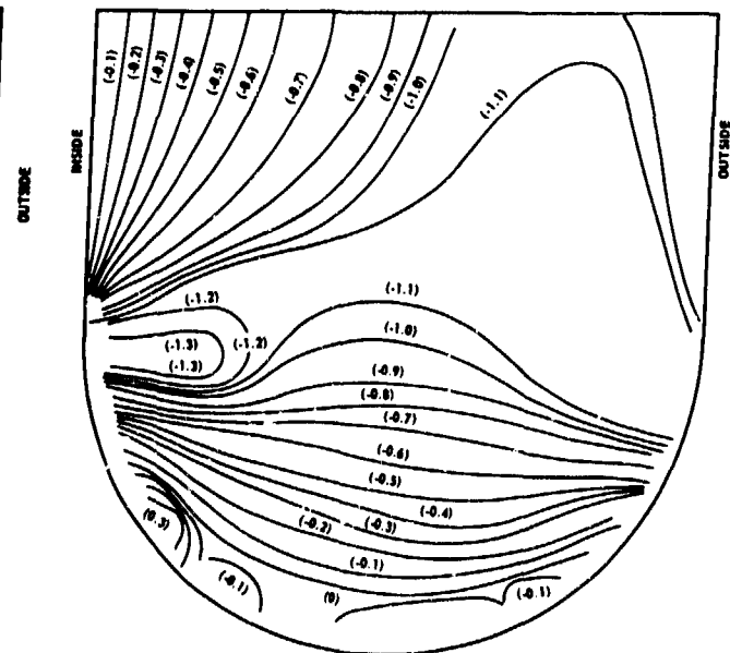
E_1 = 5 \times 10^6 P_1 = 0.3 h_1 = 0.040 Model G38
