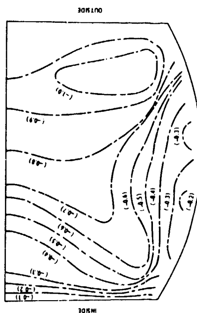
\mu = 0.3 E_1 = 5.11 \times 10^6 \text{ psi} Model G27
