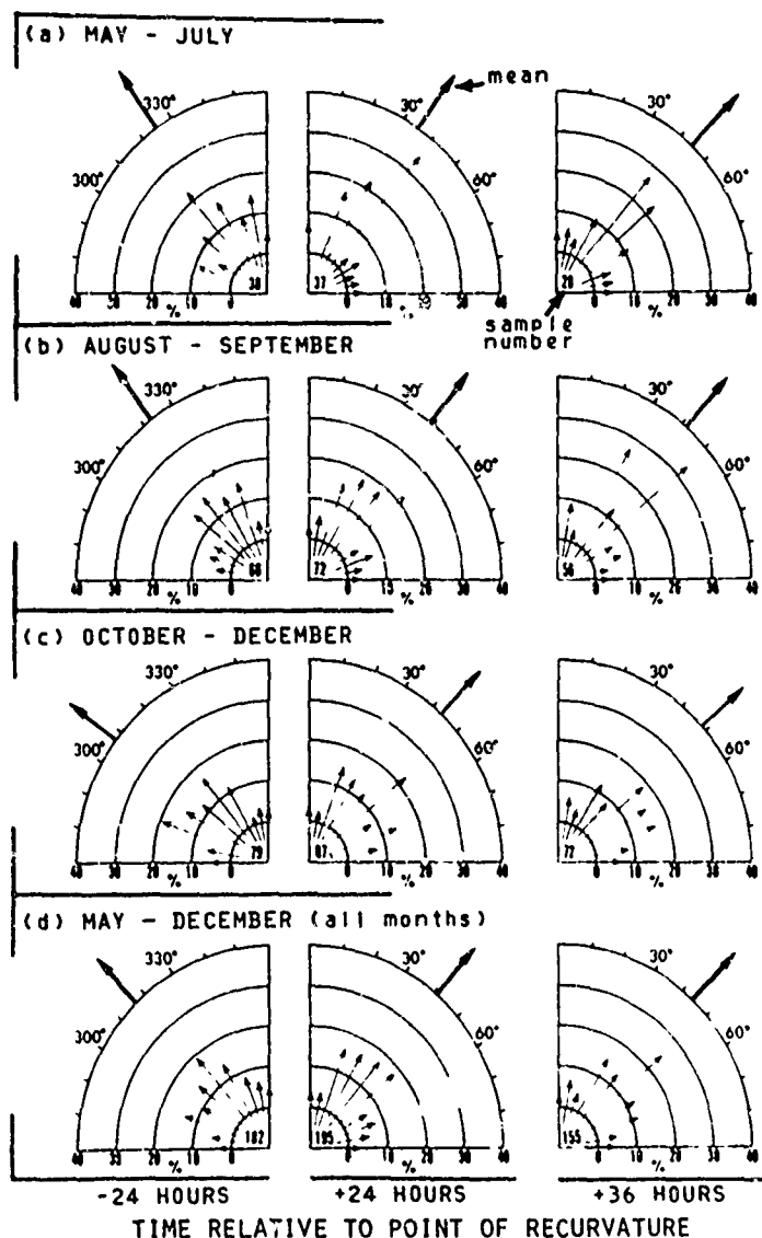
Figure 8. Percentage frequency distribution of direction of movement at specified times relative to point of recurvature for tropical storms and typhoons from 1945-1969 for the periods: (a) May-July; (b) August-September; (c) October-December; and (d) May-December (all months). The sample number of "recurvers" is given at the center of the quadrants. The cumulative percentage may not necessarily add up to 100% because a small percentage may fall outside the given quadrants. Mean directions are indicated by arrows at outer boundaries of the quadrants.
