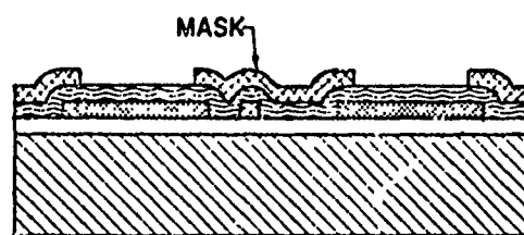
⑧ MASK FOR ETCHING THROUGH \text{SiO}_2
