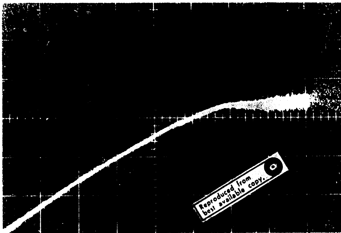
Figure III-5 Typical I-V characteristic showing flat current saturation and incoherent noise above threshold value. Diode 222-4. Horizontal scale 5 V./division, vertical scale 10 mA/division.
