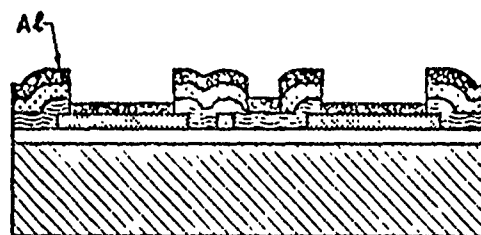
⑪ EVAPORATE INSULATED GATE METAL
