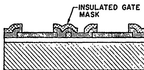
⑩ MASK FOR INSULATED GATE
