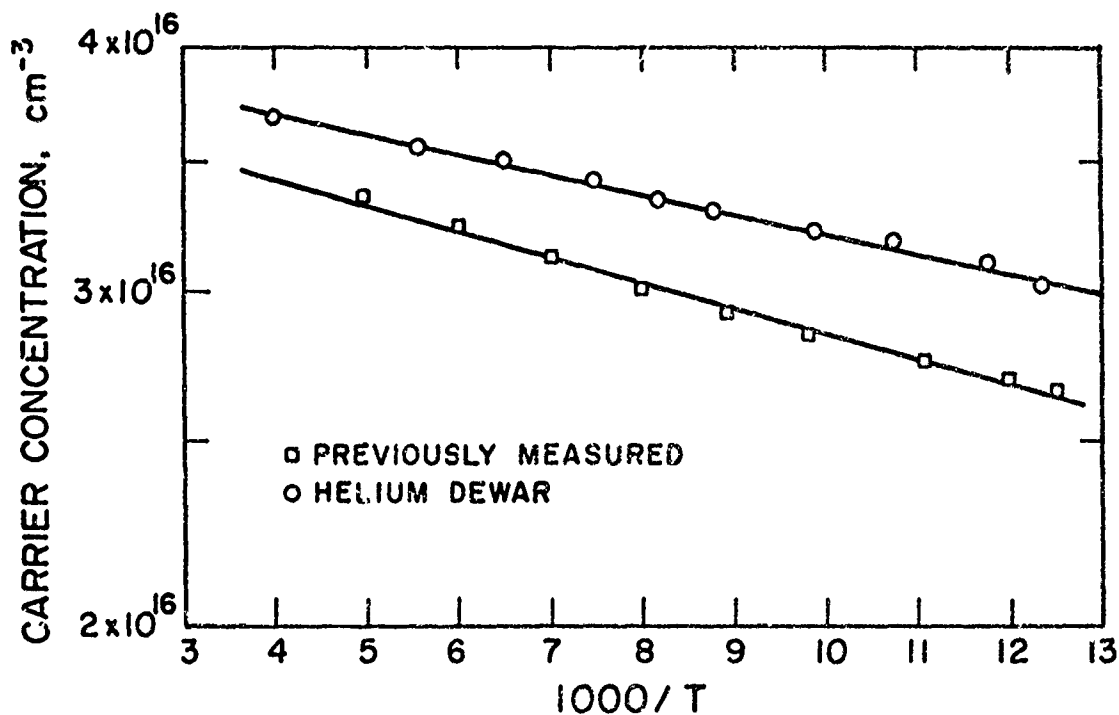
Figure V-1. Temperature dependence of the carrier concentration in n-type GaAs as measured in a Helium dewar. Comparison with previous measurements shows a large discrepancy.
