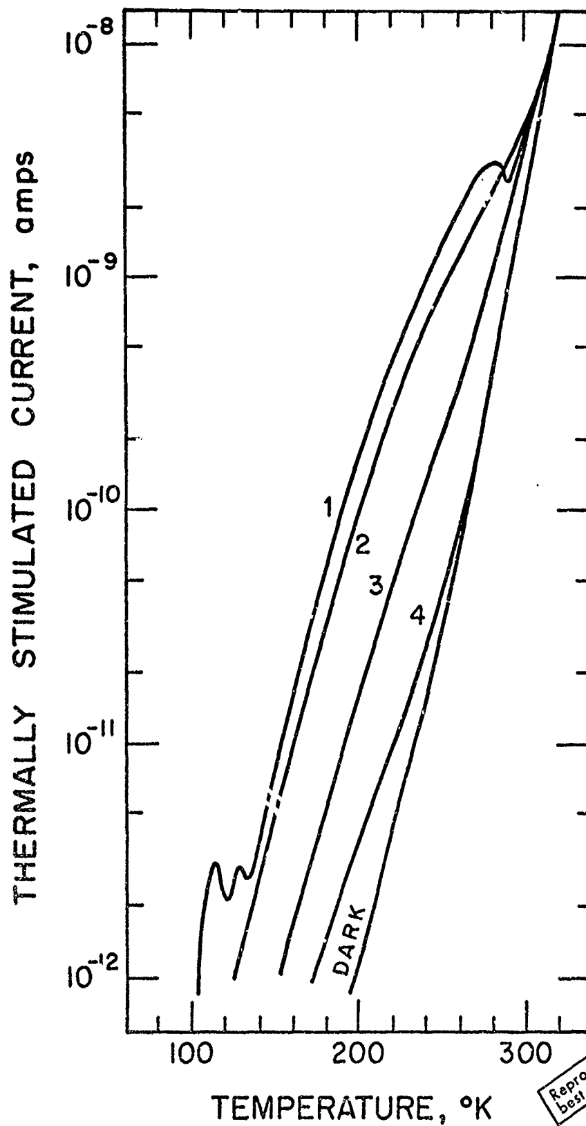
Figure V-8. Thermally stimulated current curves for deformed GaAs:Cr after the following photoexcitations: (1) white light, f = 1.0 ; (2) white light, f = 0.14 ; (3) white light, f = 0.013 ; (4) 0.85-eV radiation for 30 min. followed by 1.08-eV
