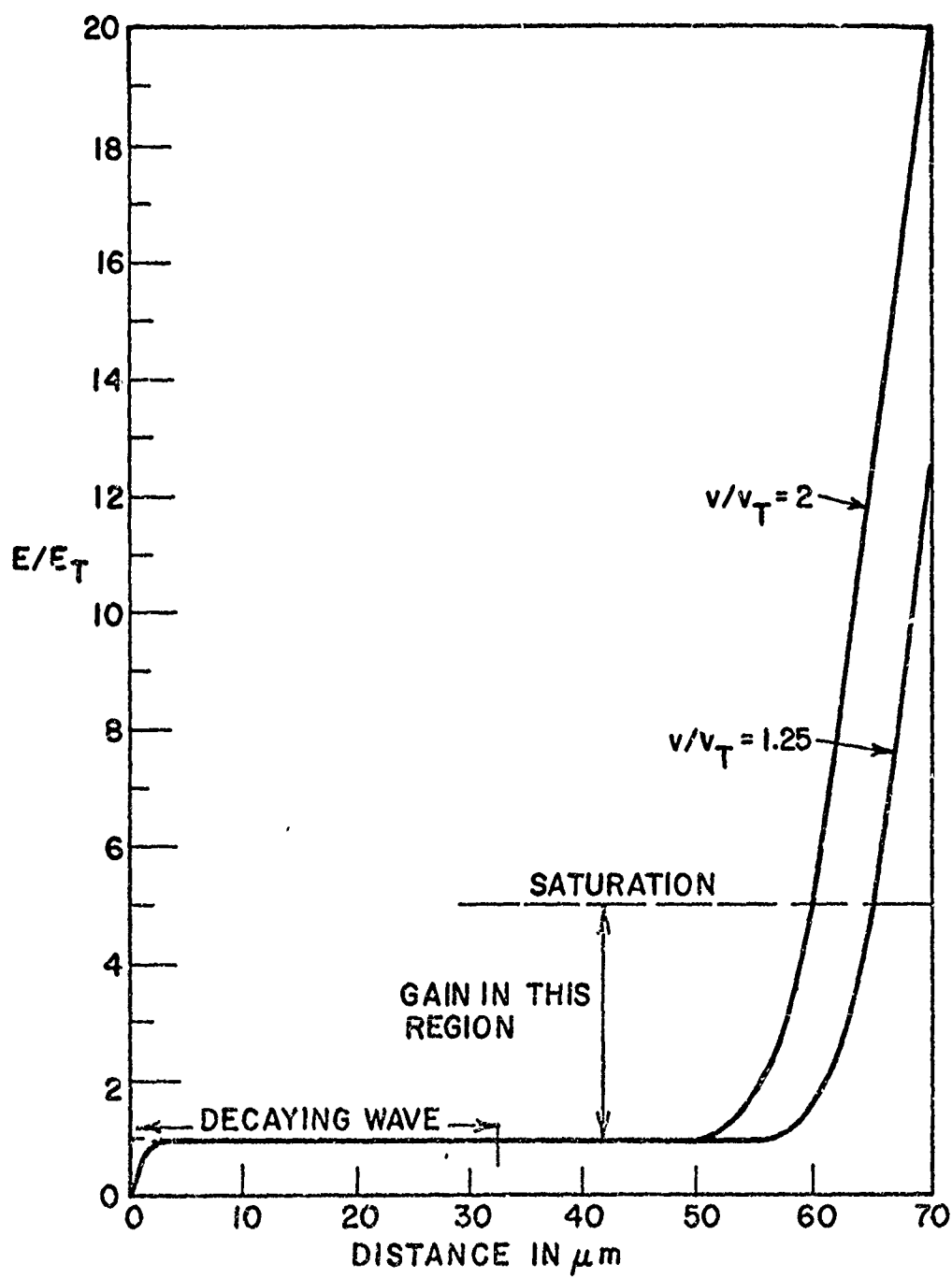
Figure III-1 A plot of the dc field distribution in a 70 \mu diode.
