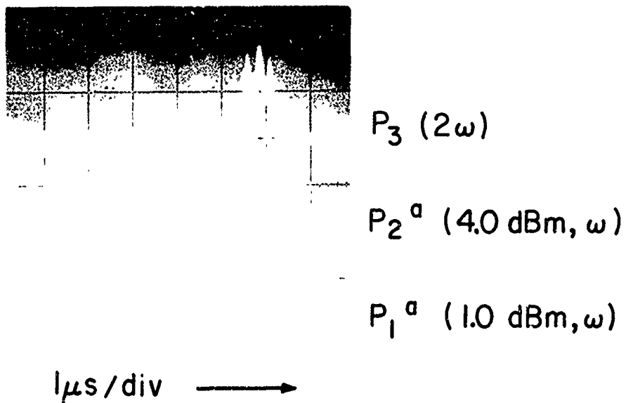
Figure III-16 Convolution property shown for pulse inputs at a carrier frequency of 176 MHz.
