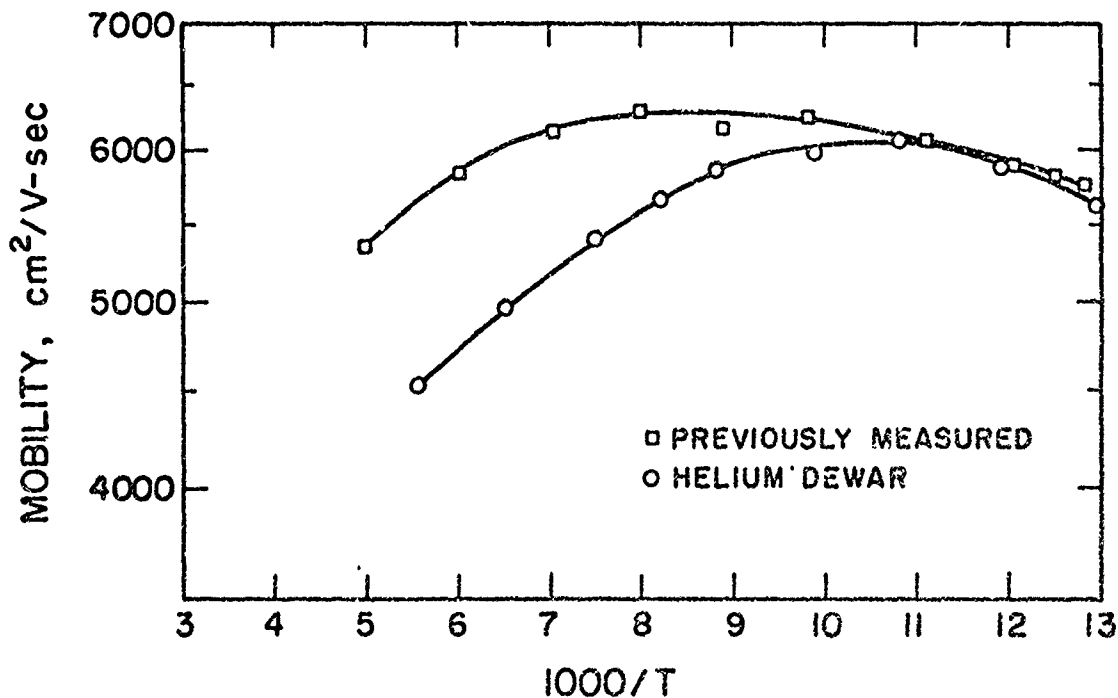
Figure V-2. Temperature dependence of the carrier mobility in n-type GaAs as measured in a Helium dewar. Comparison with previous measurements shows a large discrepancy.
