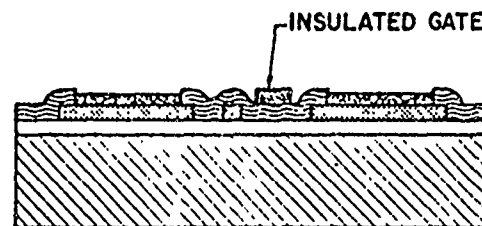
⑫ LIFT INSULATED GATE MASK
