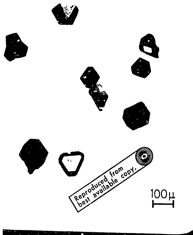
Figure II-9 Growth No. 335 shows randomly oriented GaAs hillocks rigidly attached to a (1102) Al 2 O 3 substrate.
