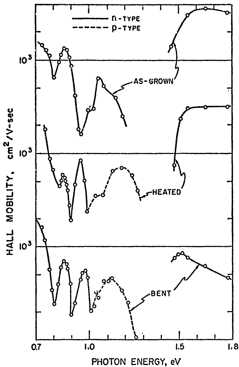
Figure V-4. Variation of photo-Hall mobility with exciting photon energy for GaAs:Cr as-grown, after heating for 1 hour at 580°C, and after deformation at 580°C. Measurements at 80°K.
