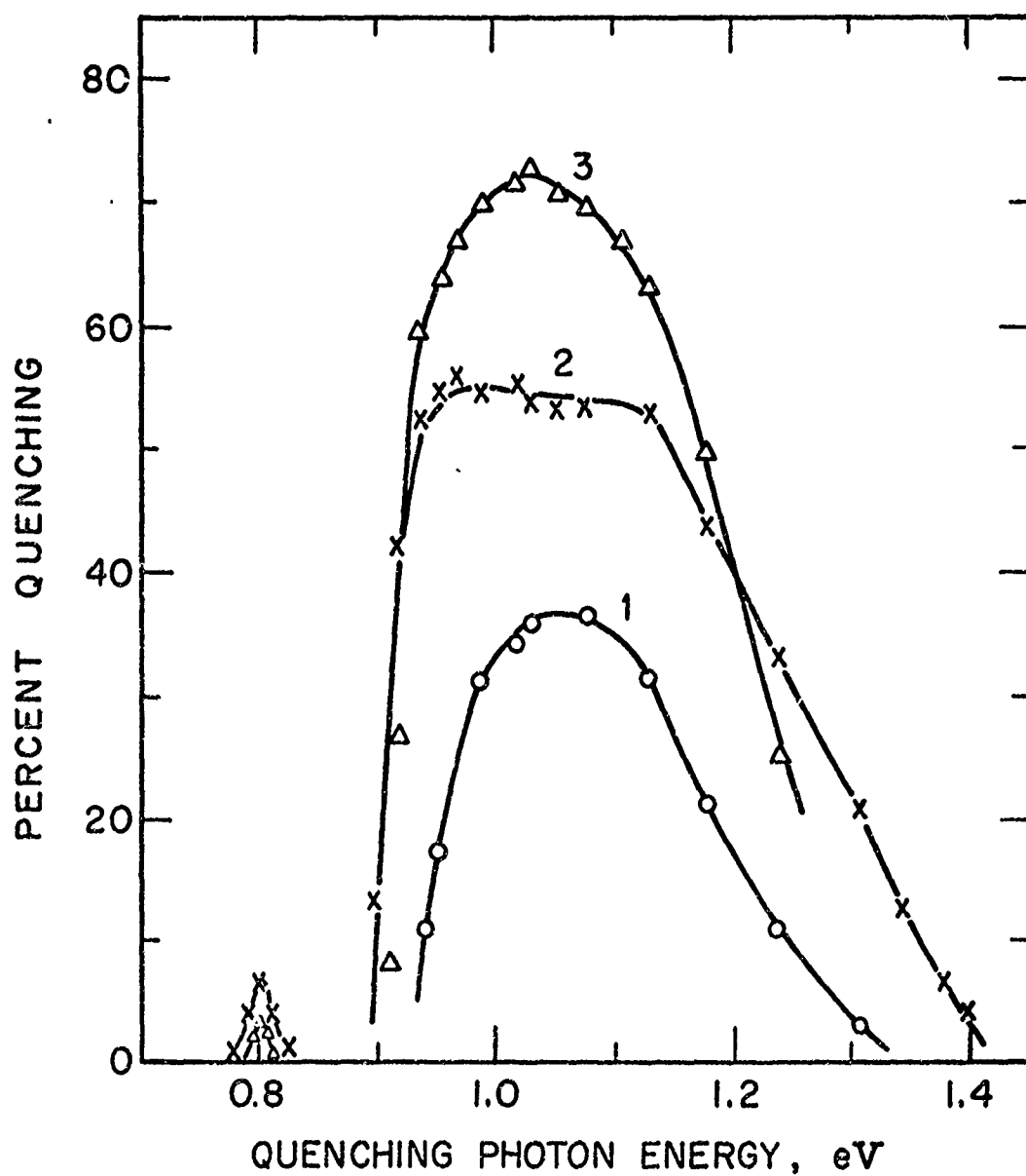
Figure V-6. Optical quenching of photoconductivity spectra at 80°K for GaAs:Cr (1) as-grown, (2) after heating for 1 hour at 580°C, and (3) after deformation at 580°C.
