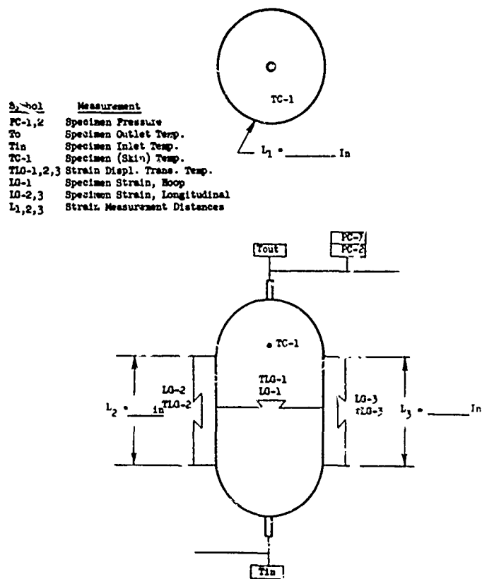
FIG. F-1 LOCATION OF INSTRUMENTATION ON TEST VESSEL
