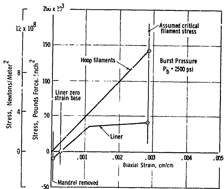
FIG. C-1 THORNE 50 PRESSURE VESSEL STRESS-STRAIN RELATIONSHIPS HOOP DIRECTION OF CYLINDER, 22°C (75°F)
