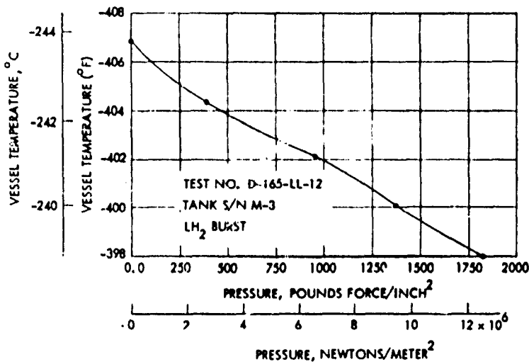
FIG. F-3 PRESSURE VS TEMPERATURE - LIQUID NITROGEN TEST
