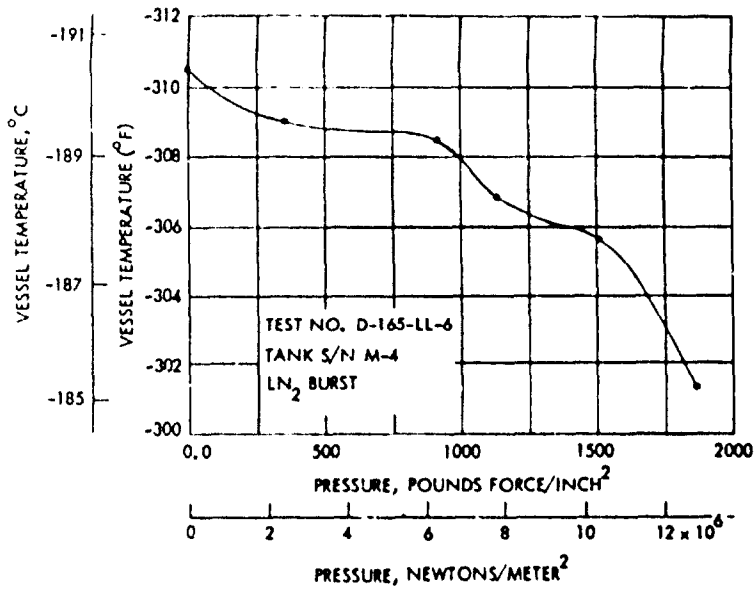
FIG. F-2 PRESSURE VS TEMPERATURE - LIQUID NITROGEN TEST
