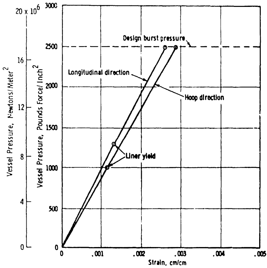
FIG. C-3 THORNIEL 50 VESSEL PRESSURE - STRAIN RELATIONSHIPS
