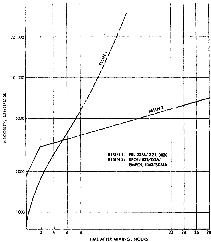
FIG. 24 VISCOSITY OF RESIN/HARDENER SYSTEMS MEASURED AT 22°C
