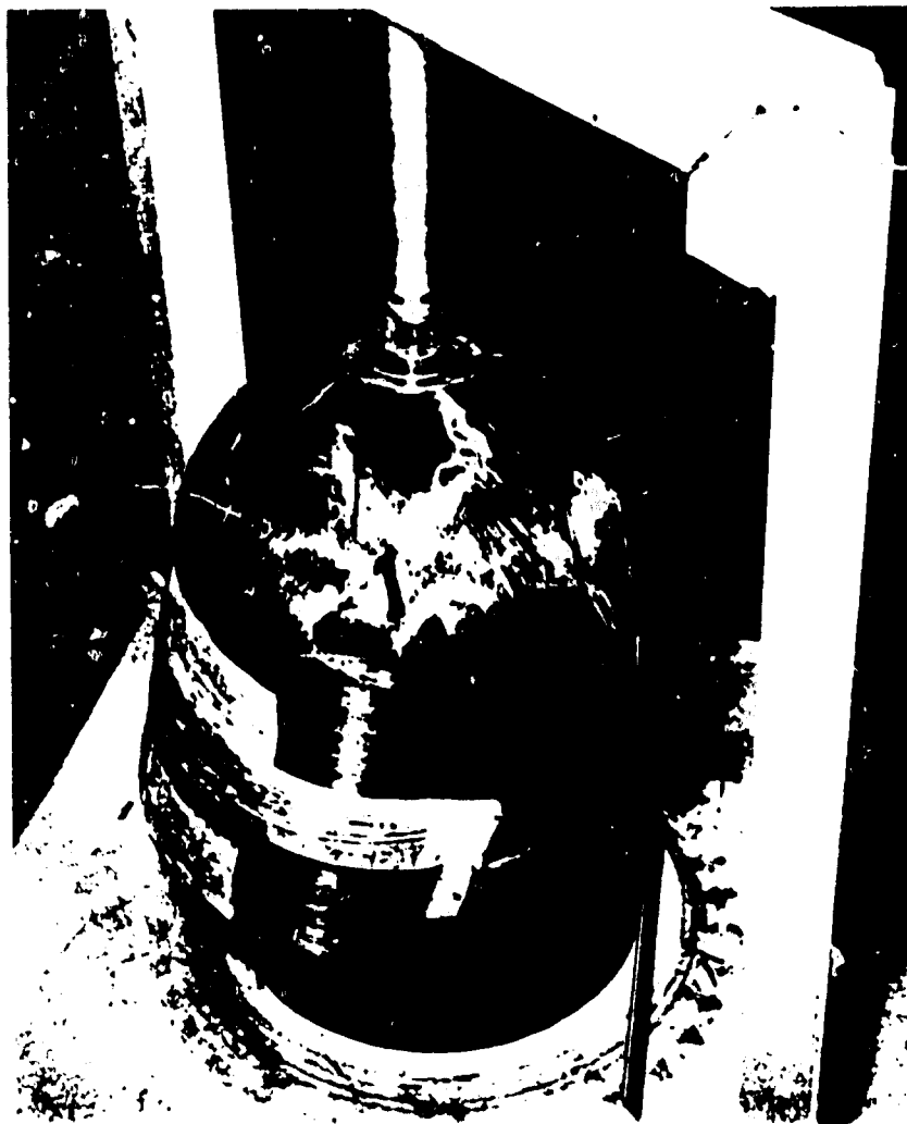
FIG. 25 POST TEST PHOTOGRAPH TANK T-1
