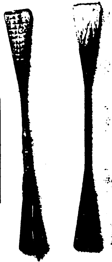
(B) TENSILE BARS FOR MODULUS AND STRENGTH. BAR ON LEFT HAS ELECTRIC STRAIN GAGE BONDED ON.
