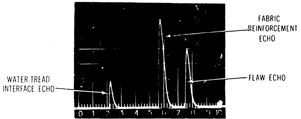
Fig 7a TRACE PRODUCED WITH SUPPRESSION AND SWEPT GAIN
