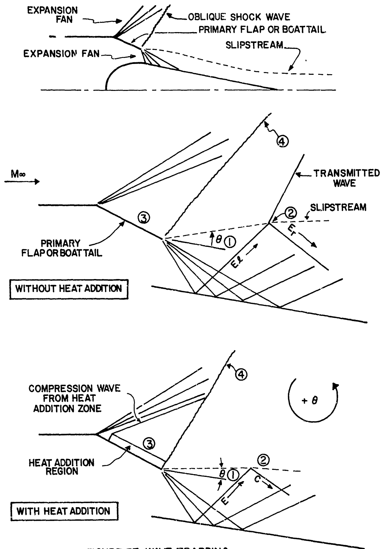
FIGURE 37. WAVE TRAPPING.
