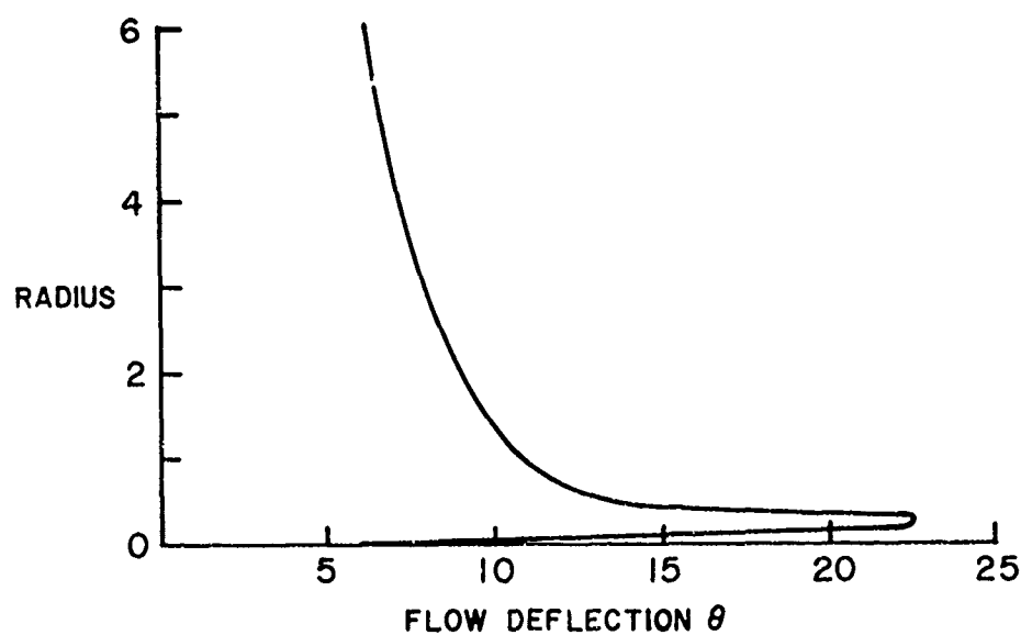
(B) FLOW DEFLECTION AS A FUNCTION OF RADIUS
