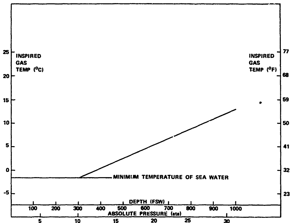
Figure 1. Minimum Allowable Inspired Gas Temperatures at Depth for Mk 10-Mod 4 Closed Circuit Mixed Gas Underwater Breathing Apparatus, from Material Certification Procedures and Criteria Manual for Deep Submergence Systems, NAVSHIPS 0090-028-2010
