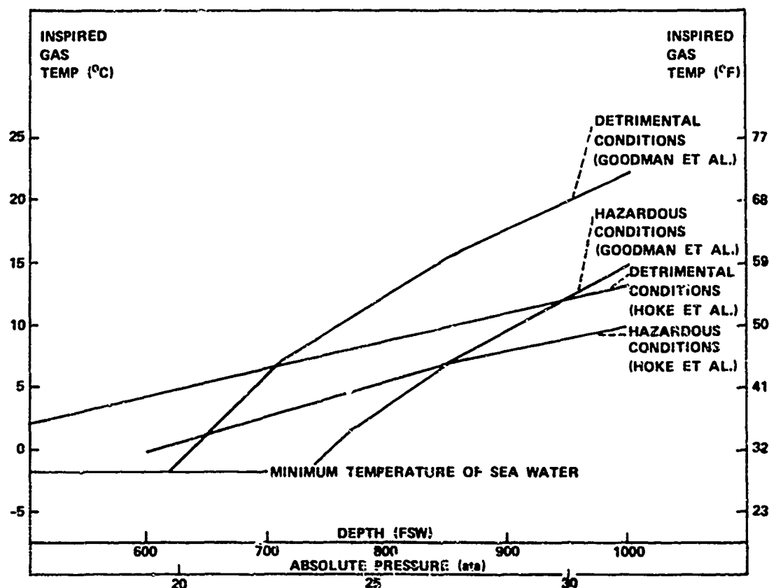
Figure 2. Inspired Gas Temperatures at Depth Resulting in Respiratory Heat Loss Causing Detrimental and Hazardous Conditions, from calculations by Hoke et al 2 and Goodman et al 3
