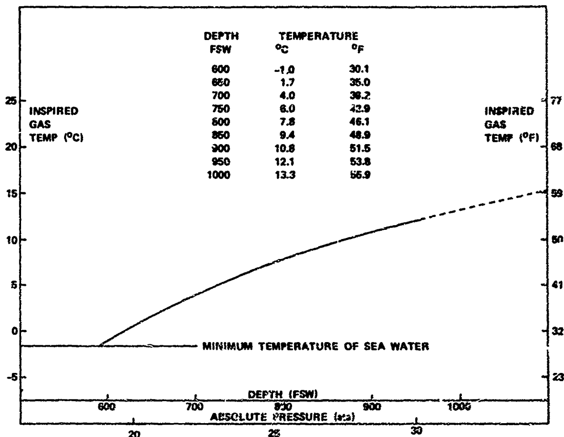
Figure 5. Minimum Safe Inspired Gas Temperature Limits
