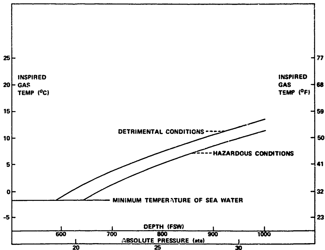
Figure 4. Inspired Gas Temperatures at Depth Resulting in Respiratory Heat Loss Causing Detrimental and Hazardous Diving Conditions, as calculated from experimental data of Goodman et al 3
