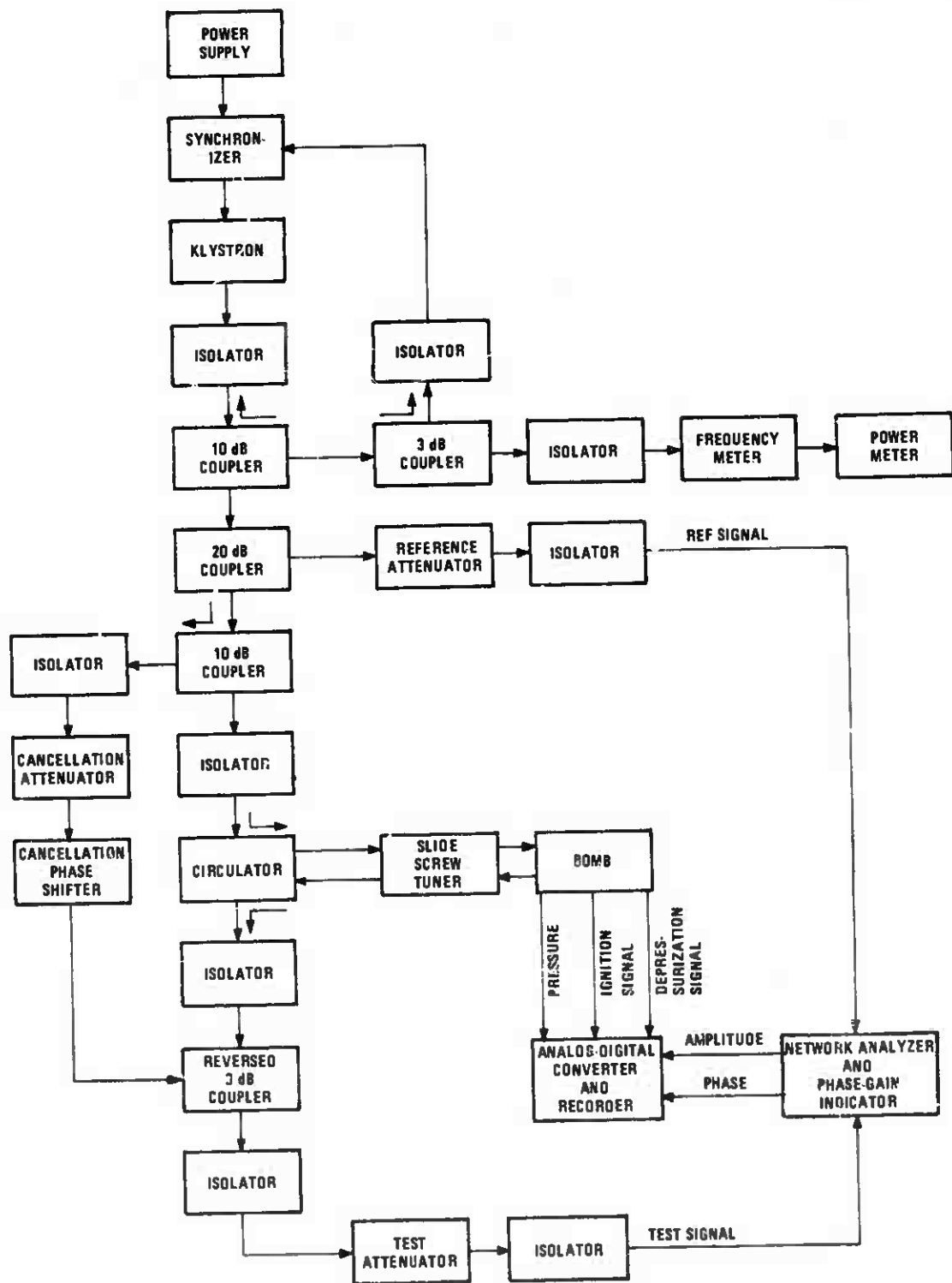
Figure 15. System Block Diagram.
