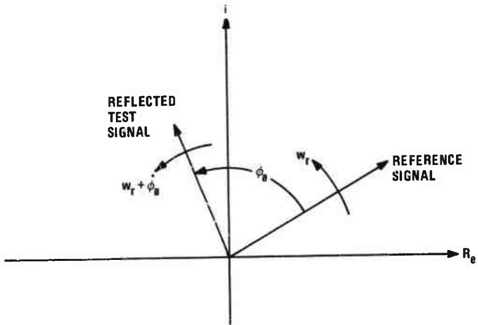
Figure 12. Phaser Diagram.
