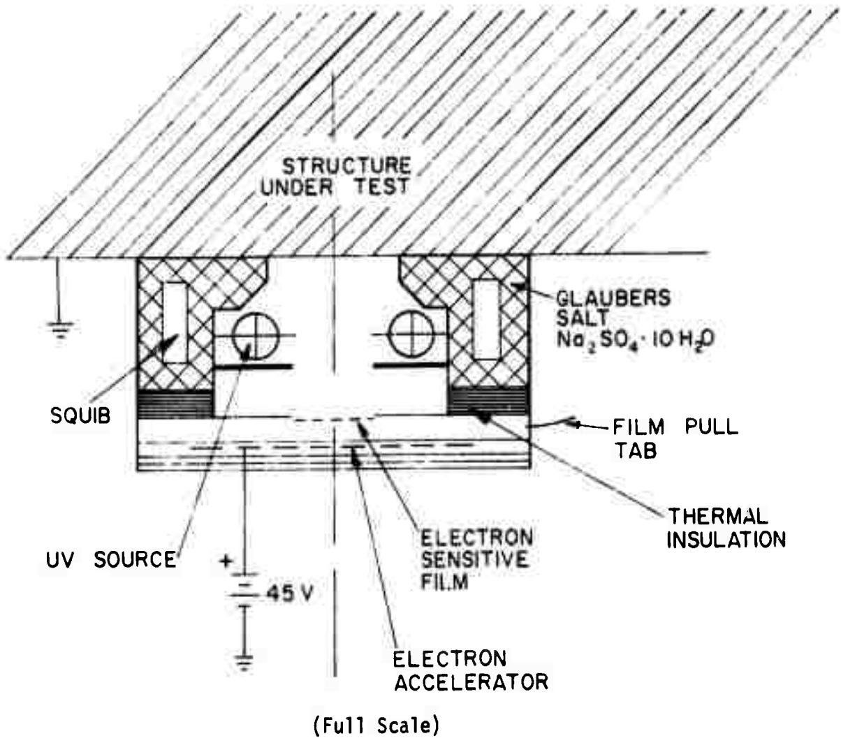
Figure 16. Placket Detector.
