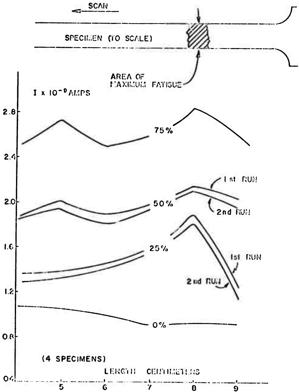
Figure 15. Exo-electron Current vs. Length and Fatigue Level (7075-T6 aluminum).
