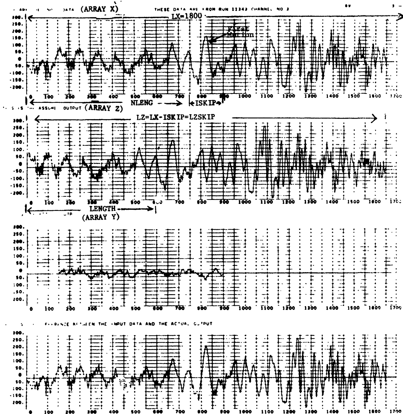
Figure 3a. Application of Program MAXLKH to Infrasonic Record 11343 Channel 3.
