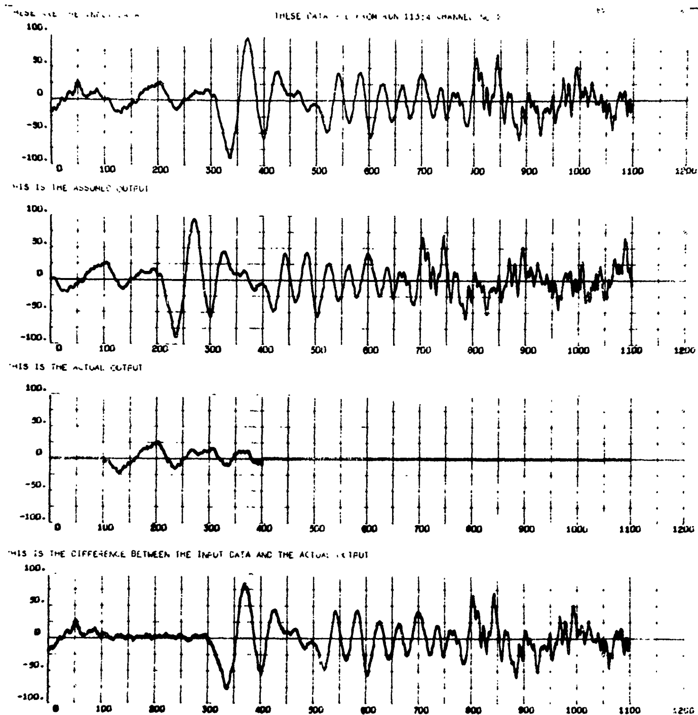
Figure 4a. Application of Program MAXLKH to Infrasonic Record 11354; Channel 1.
