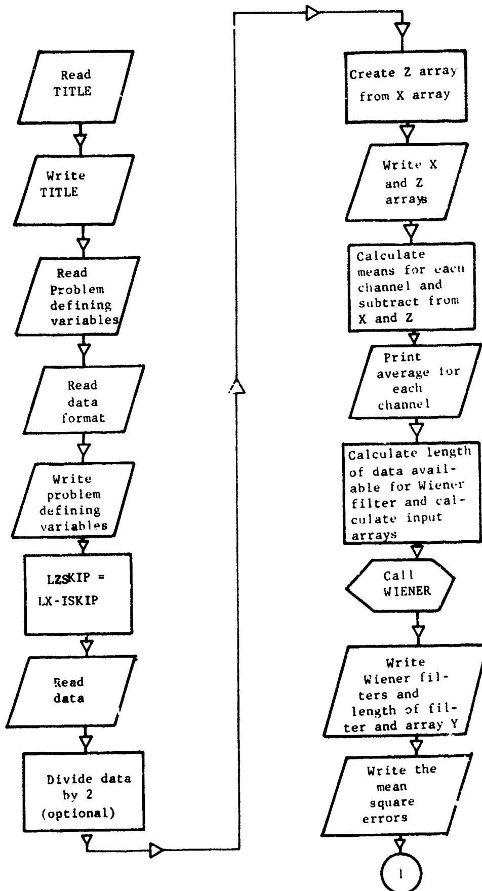
Figure 2. Flow Chart of MAXLKH
