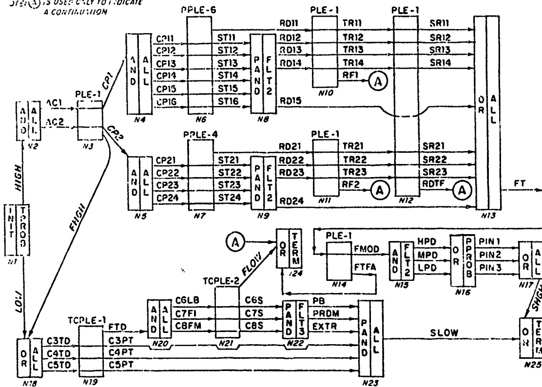
HELICOPTER EXAMPLE Figure 3
