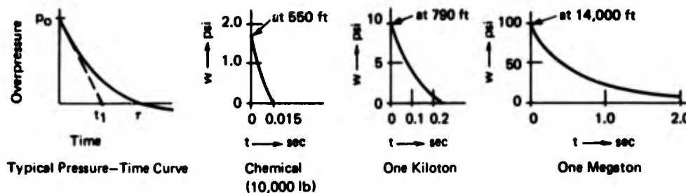
Figure 3.1. Pressure-time signatures of typical explosions.
