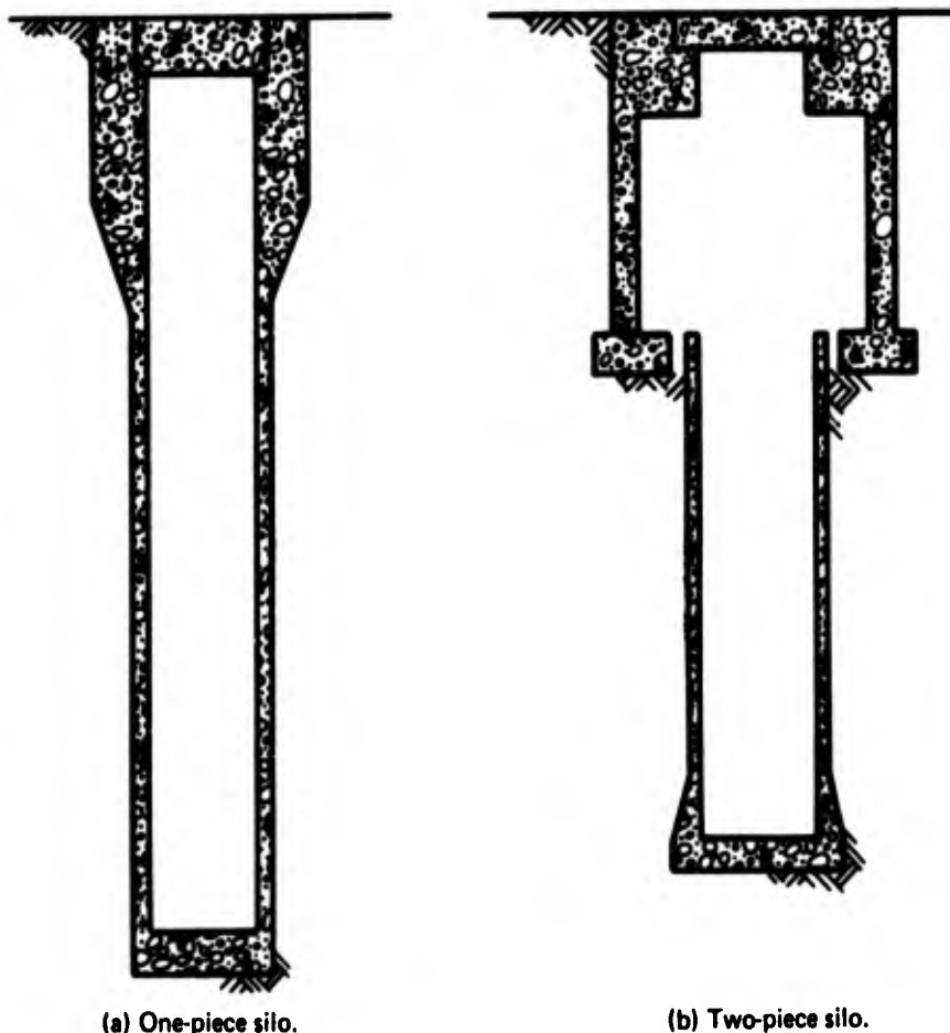
Figure 5.8. Typical silo configurations.
