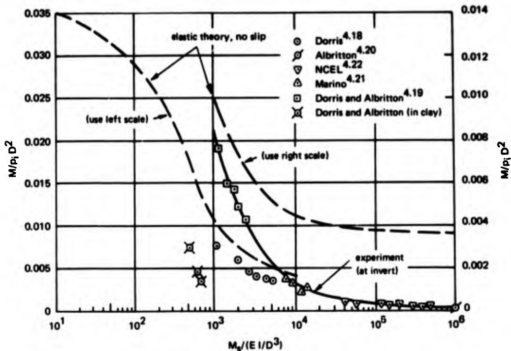
Figure 4.6. Moments in buried cylinders.
