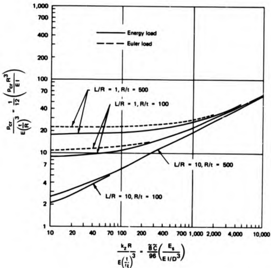
Figure 4.7. Critical pressures for cylinders with elastic support.
