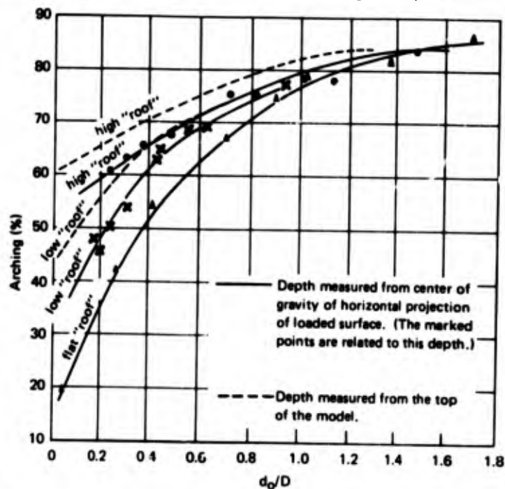
Figure 5.12. Arching versus depth and shape. (From Reference 5.36)
