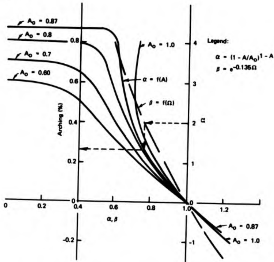
Figure 3.8. Plot for determining the arching over structures in granular soils.
