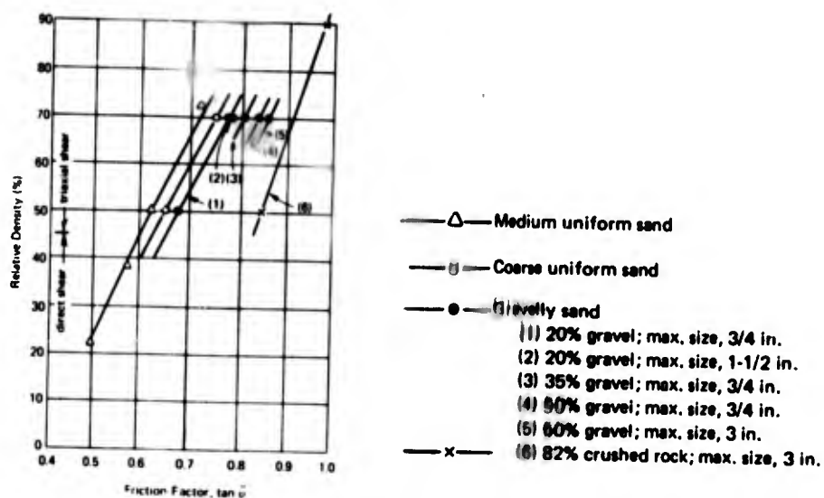
Figure 2.1. Effect of relative density on the friction factor for coarse-grained soils. (From Reference 2.17)
