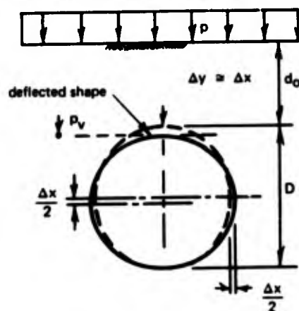
Figure 4.2. Deflected shape of horizontal cylinder.
