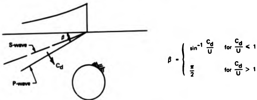
Figure 3.2. Air-blast induced P and S waves.
