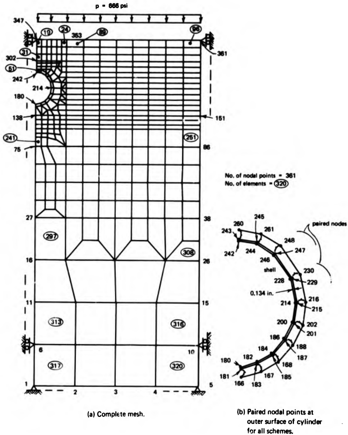
Figure 4.10. Finite element mesh for buried cylinder.
