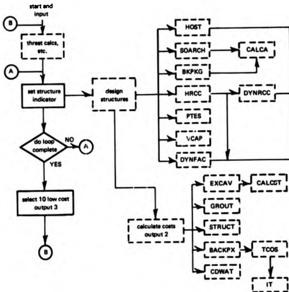
Figure 6.5. Flow diagram for structural design calculations.
