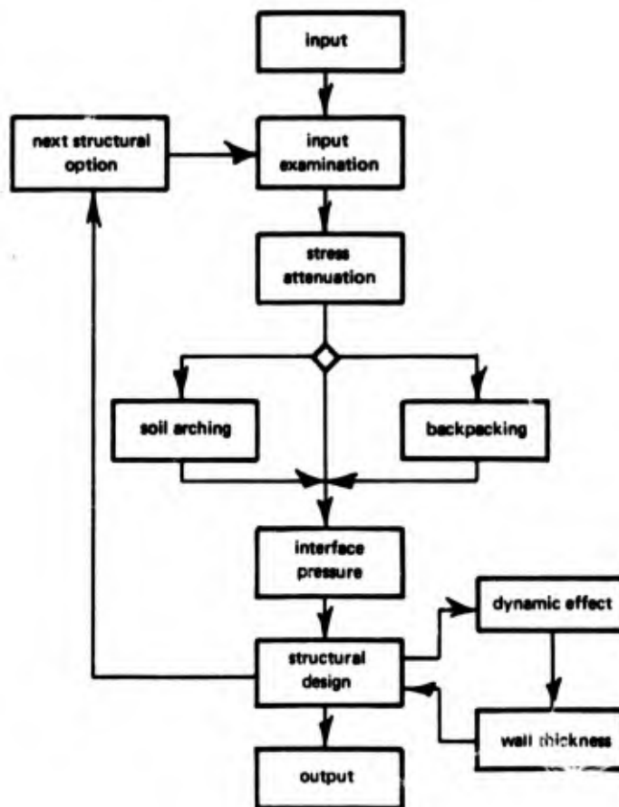
Figure 6.1. General flow diagram.
