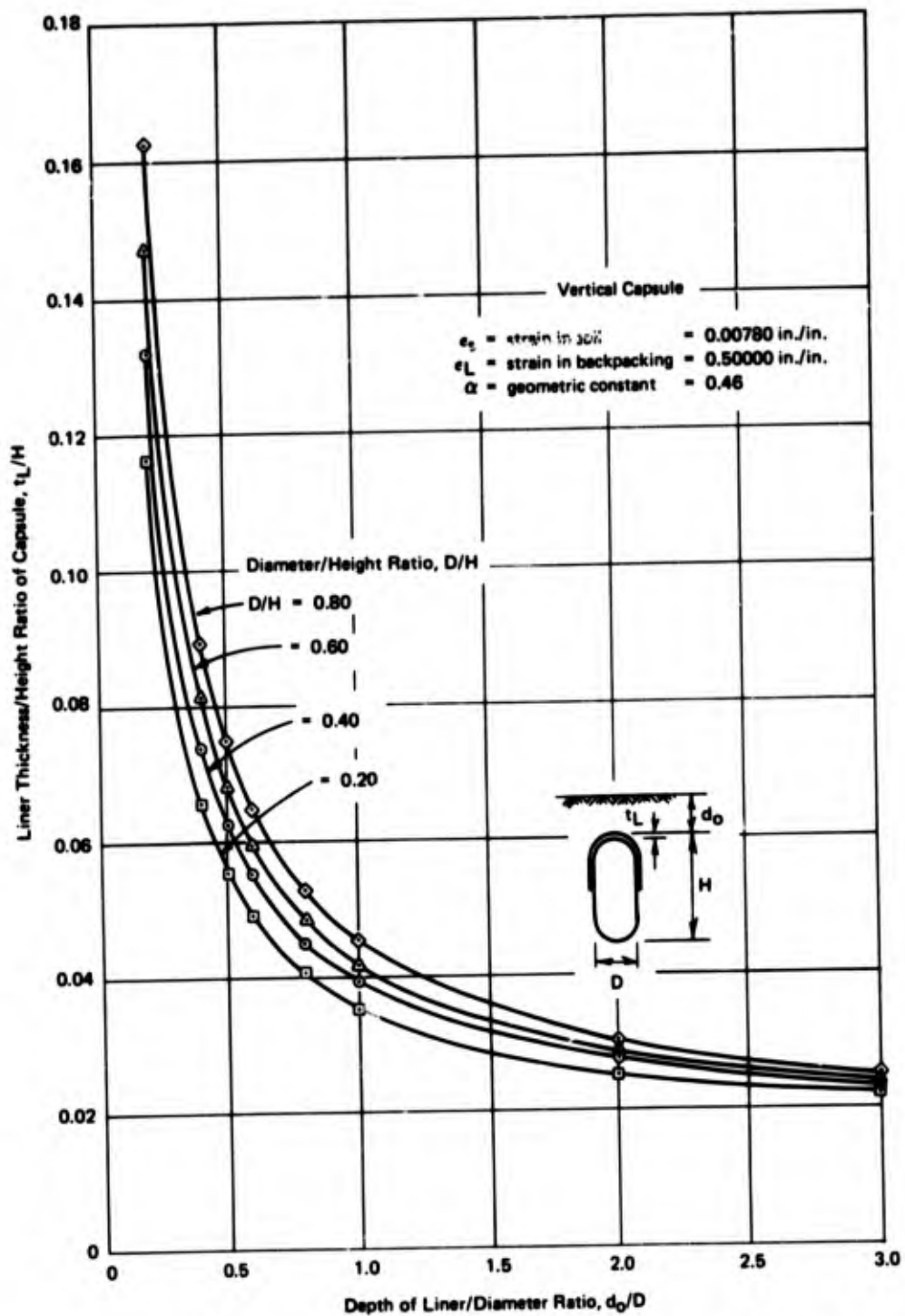
Figure 5.7. Thickness of liner and depth of cover for maximum arching over capsule. (Prepared by S. K. Takahashi of the NCEL staff.)
