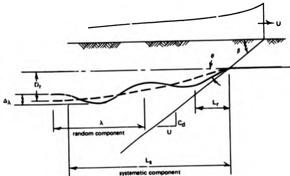
Figure 5.1. Deflection of a buried cable subjected to a blast wave.
