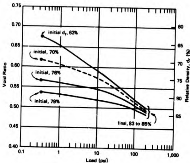
Figure 2.2. Compressibility characteristics of a fine, uniform sand in relation to placement relative density. (From Reference 2.17).
