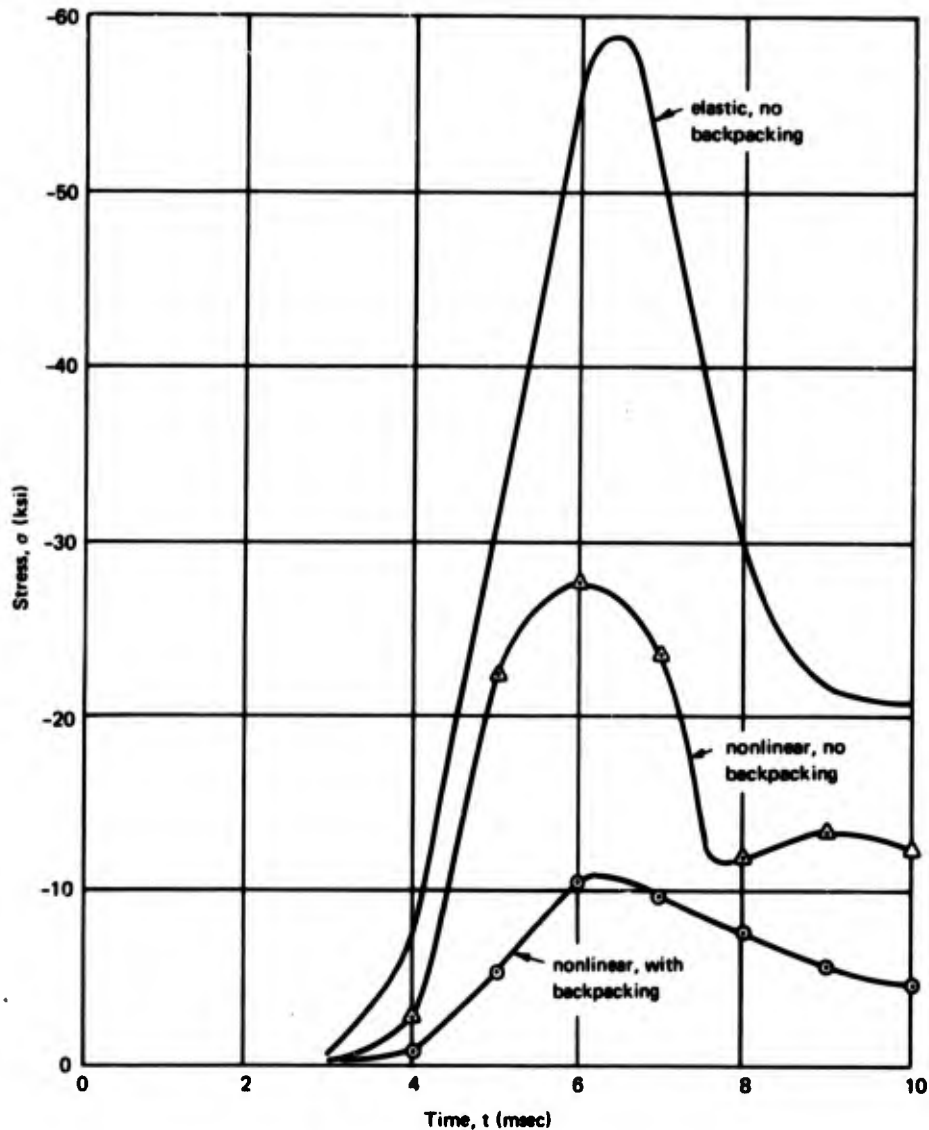
Figure 4.18. Minimum stress at springline of buried cylinder (configuration 4).
