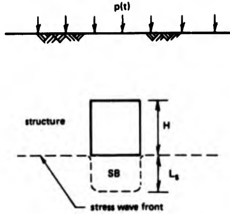
Figure 3.5. Distortion of stress front below a stiff structure.
