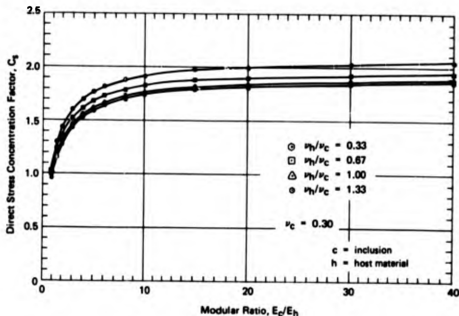
Figure 5.13. Direct stress concentration factor, C_s .
