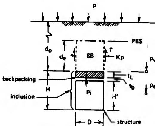
Figure 3.9. Inclusion in soil field.
