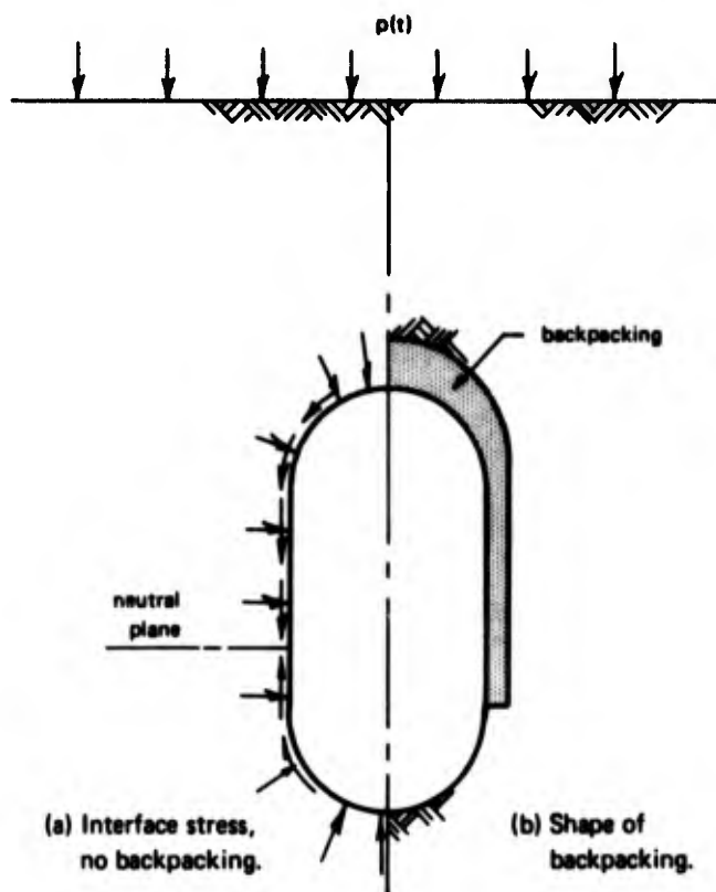
Figure 5.6. Vertical capsule sections.
