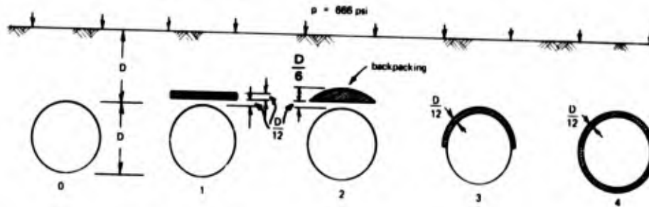
Figure 4.9. Backpacking configurations for buried cylinders.
