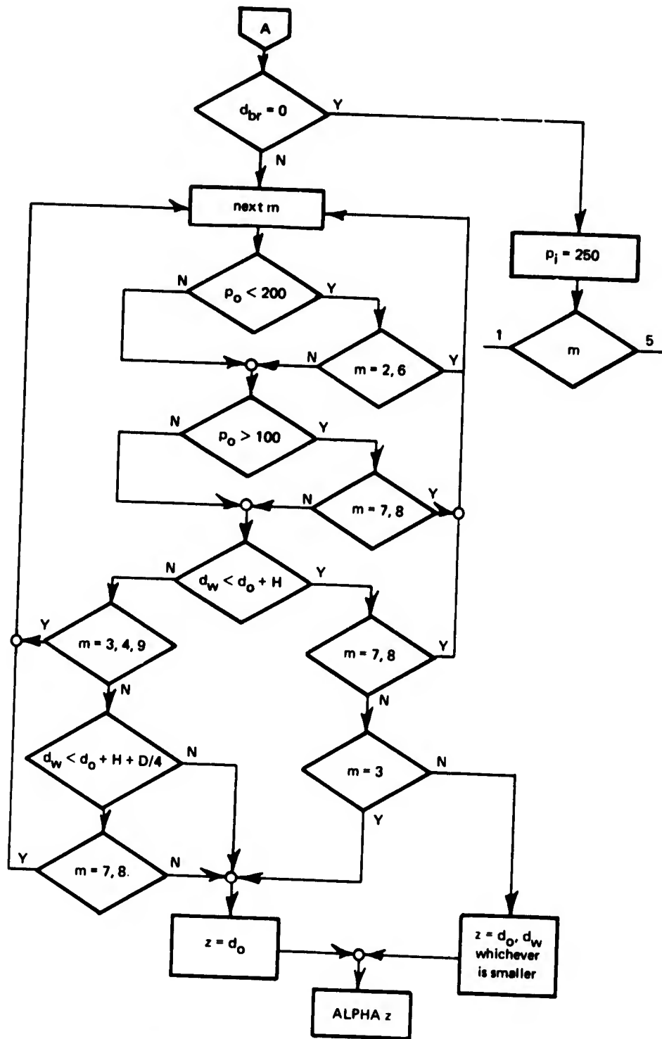
Figure 6.4. Qualification process for structure.
