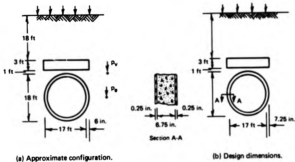
Figure 4.8. Example of a buried cylinder design.
