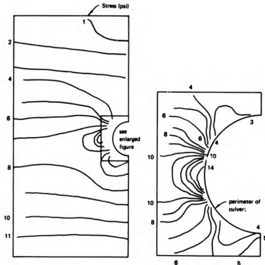
Figure 4.23. Horizontal soil stress contours (Y-Z plane).
