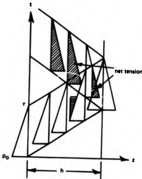
Figure 3.7. Stress wave diagram.
