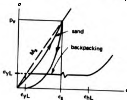
Figure 3.10. Stress-strain diagrams.
