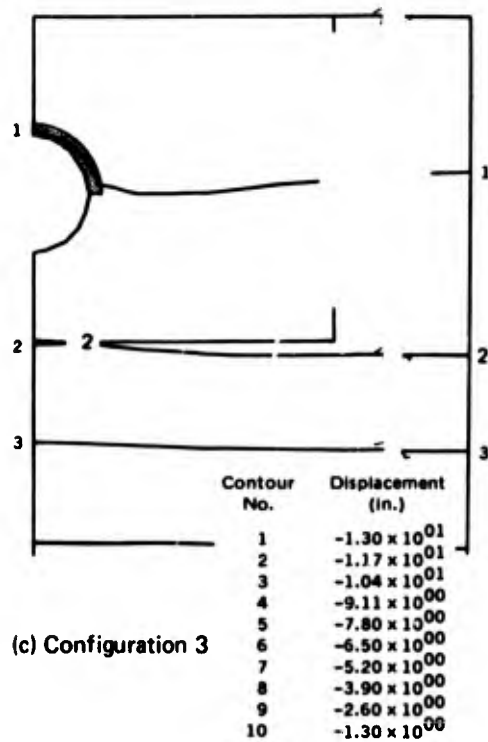
Figure 4.12. Static vertical displacement contours.
