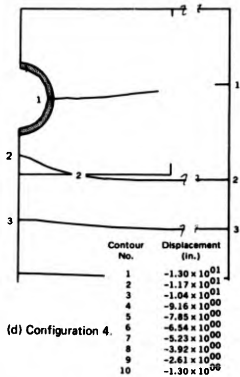
Figure 4.12. Static vertical displacement contours.
