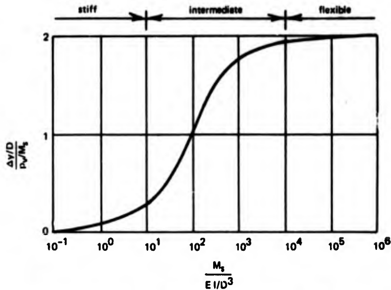
Figure 4.3. Vertical diametral deflection of a cylinder under static loading.
