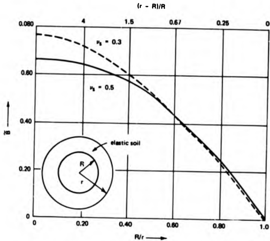
Figure 4.4. Modulus of soil support for elastic ring. (From Reference 4.14)
