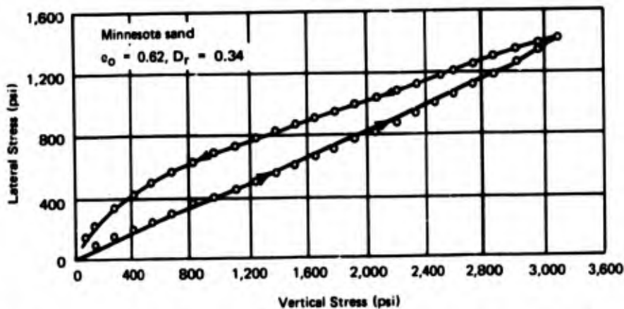
Figure 2.4. Lateral stress during one-dimensional compression. (From Reference 2.28)
