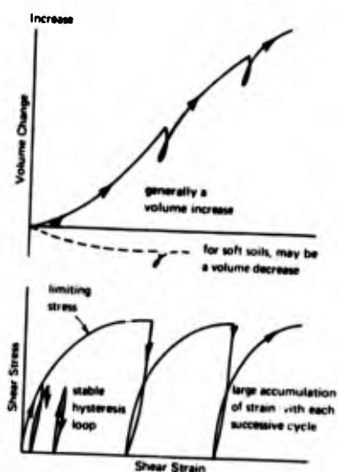
Figure 2.7. Typical stress-strain and volume change curves in shear. (From Reference 2.1)
