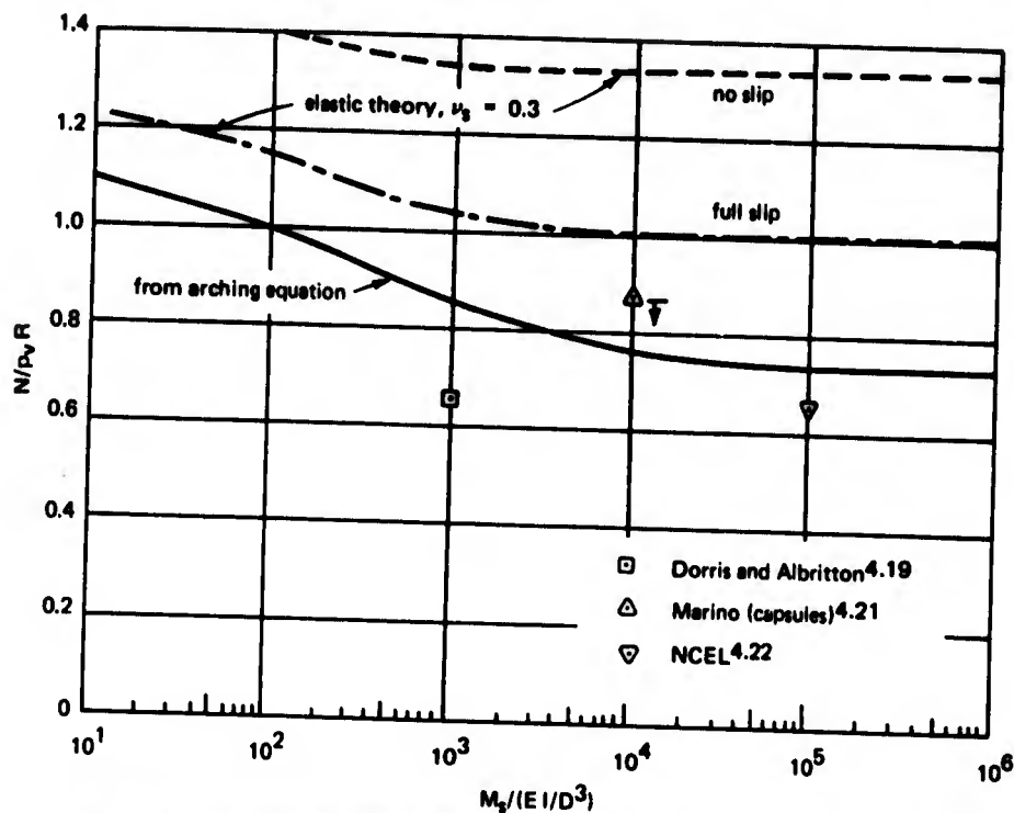
Figure 4.5. Comparative determination of thrust at springline under static loading.
