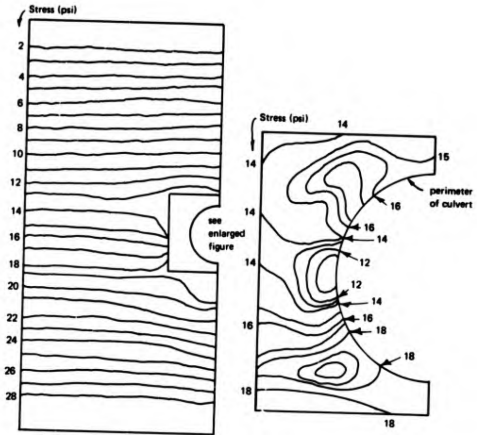
Figure 4.21. Vertical soil stress contours (Y-Z plane).
