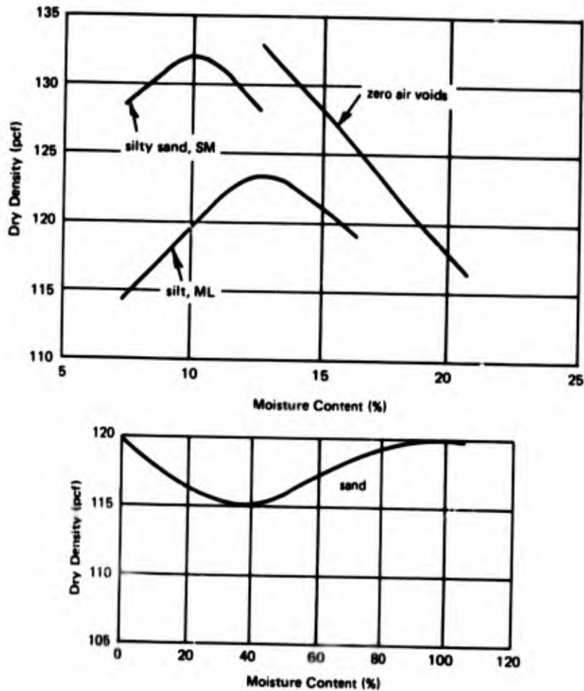
Figure 2.3. Modified AASHO compaction curves.
