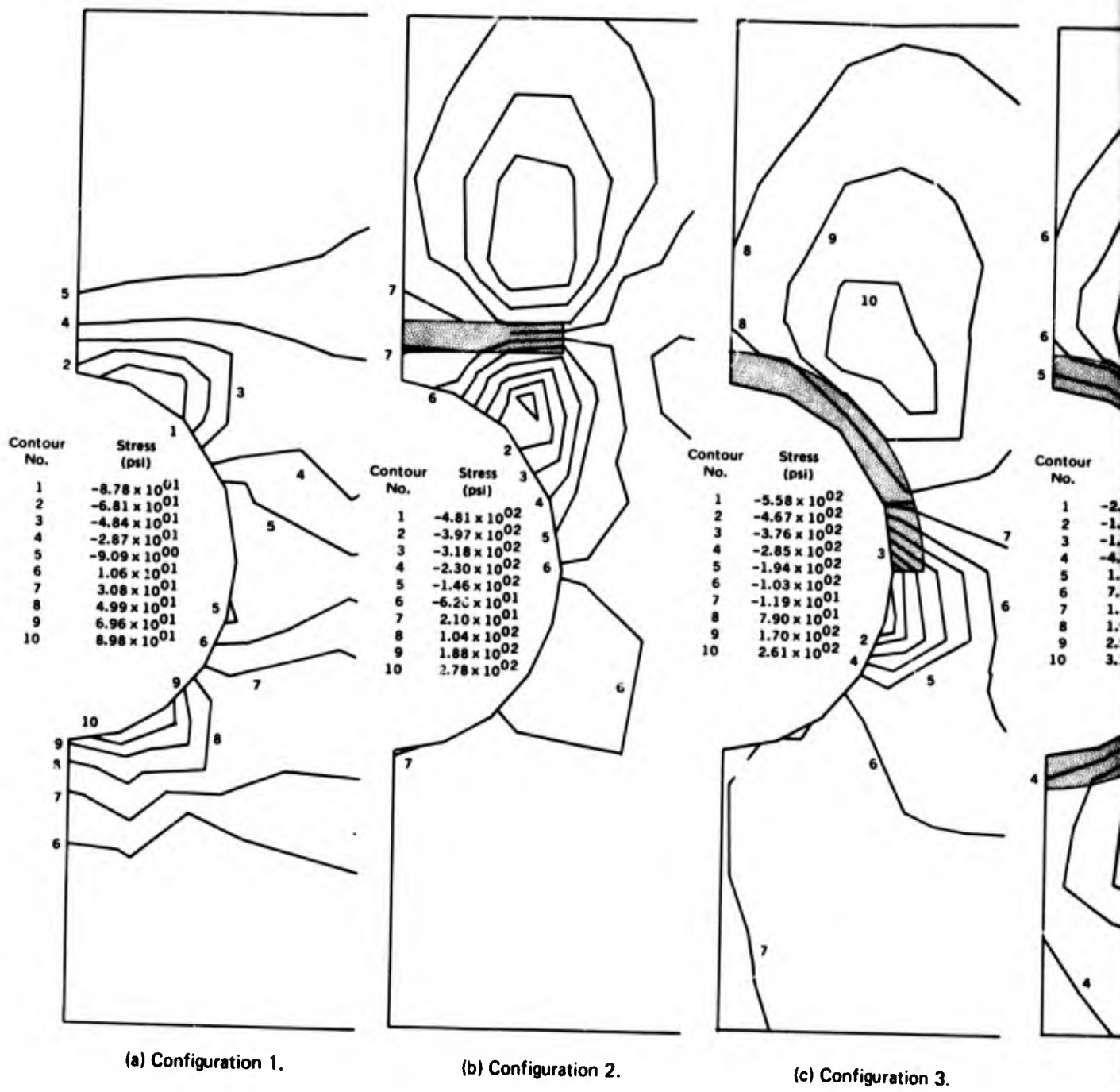
Figure 4.15. Comparison of static shear stress patterns.
