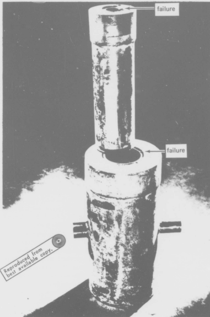
Figure 3.6. Stress wave fracture in model expansion chamber.
