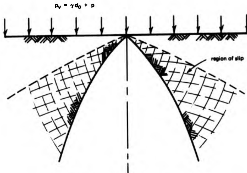
Figure 4.1. Typical stable arch form in cohesive soils.
