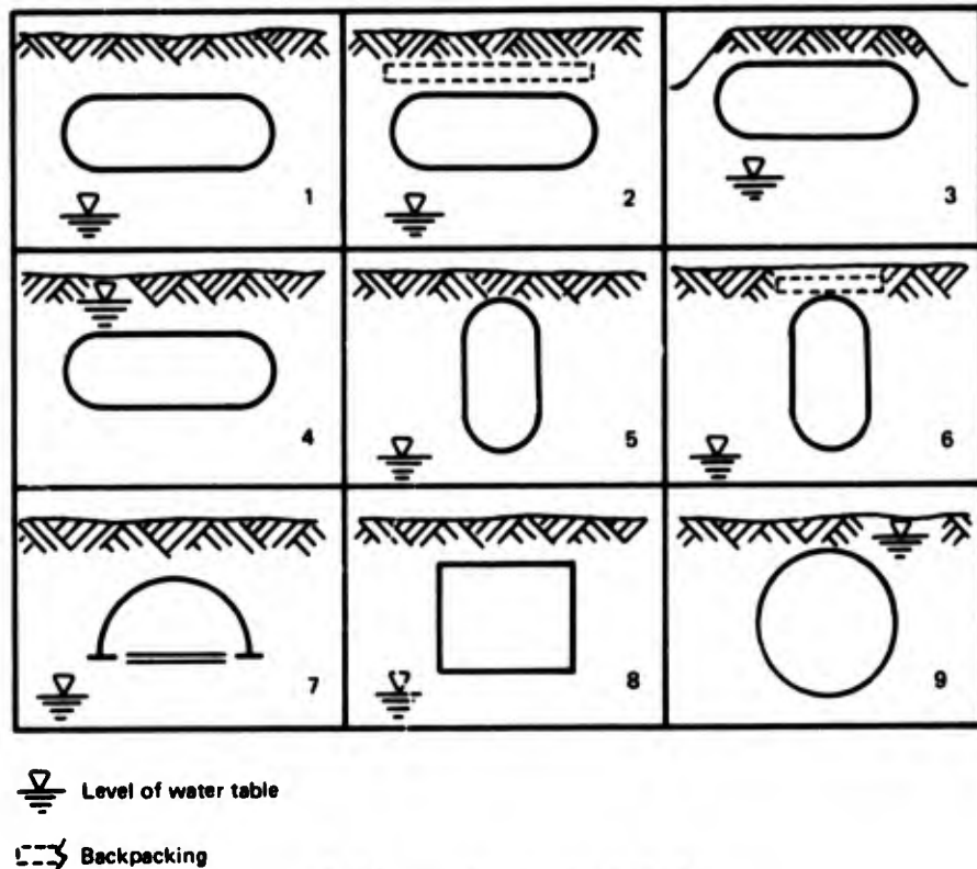
Figure 6.2. Structural configurations.
