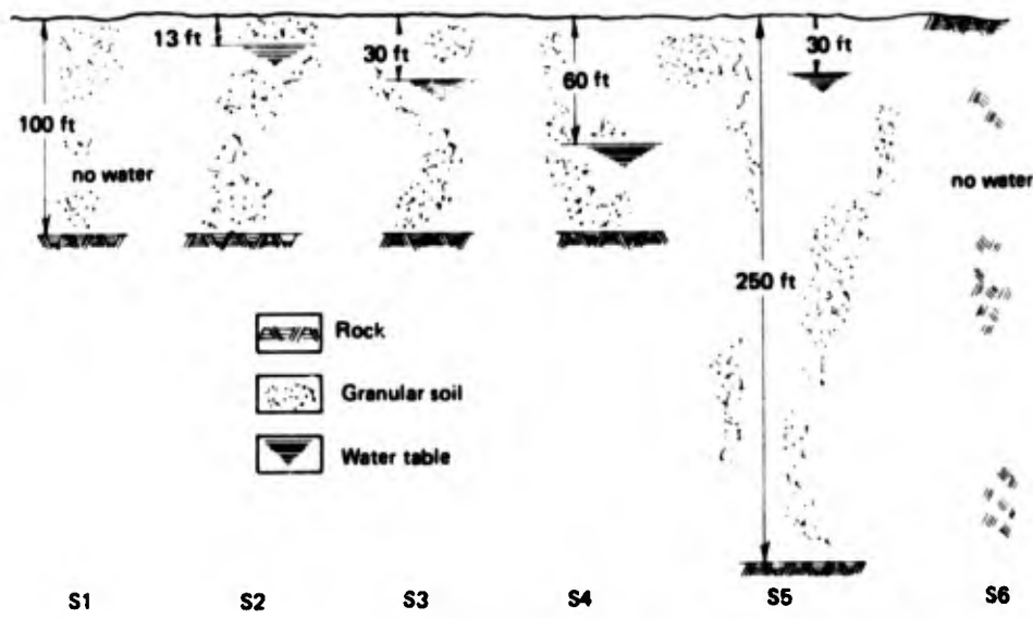
Figure 6.3. Site profiles.
