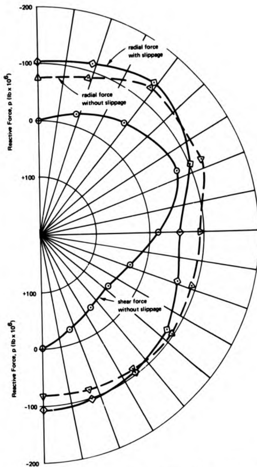
Figure 4.17. Reactive nodal point shear and radial forces on cylinder (configuration 0).
