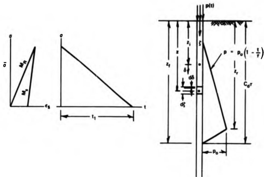
Figure 3.4. Stress—depth relationships.
