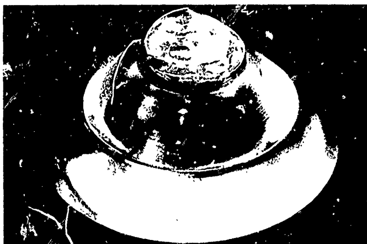
(c) Low-pressure face of fractured window.
