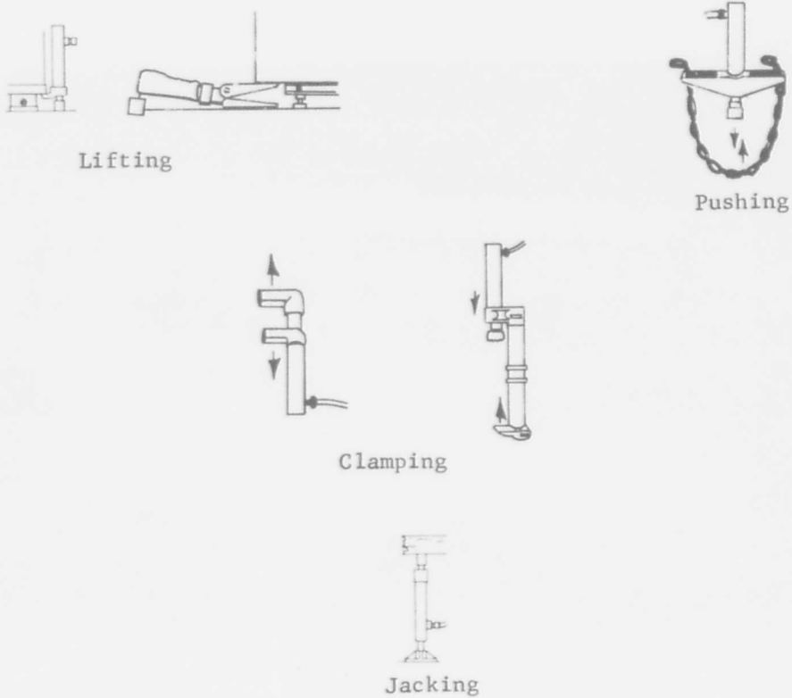
Figure 12. Typical Hydraulic Ram System
