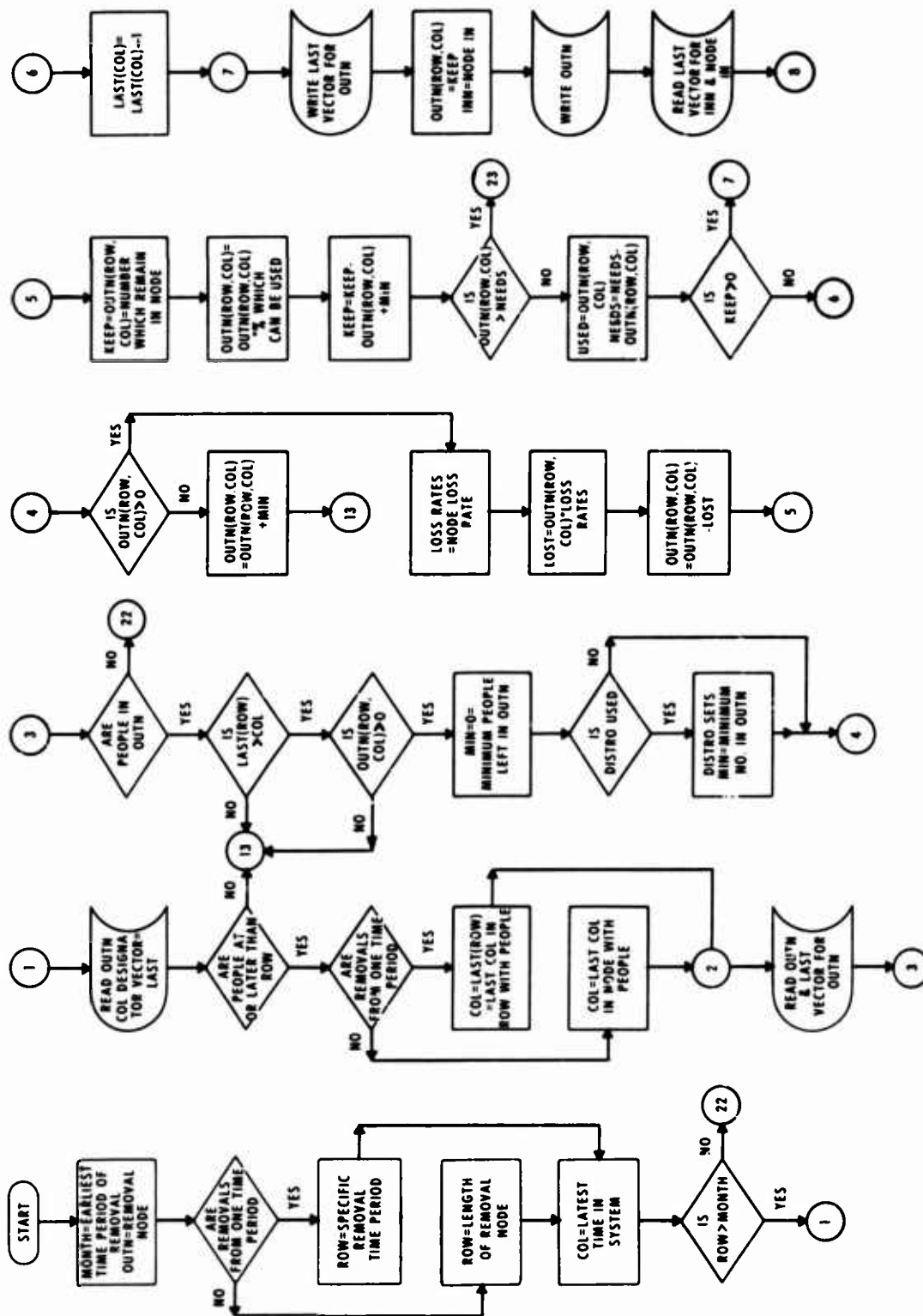
Figure 11. Subroutine LOCK
