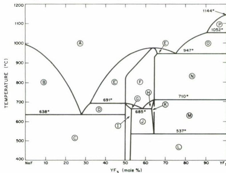
Fig. III-5. Pseudobinary phase diagram of the NaF- \text{YF}_3 system (Ref. 8).
