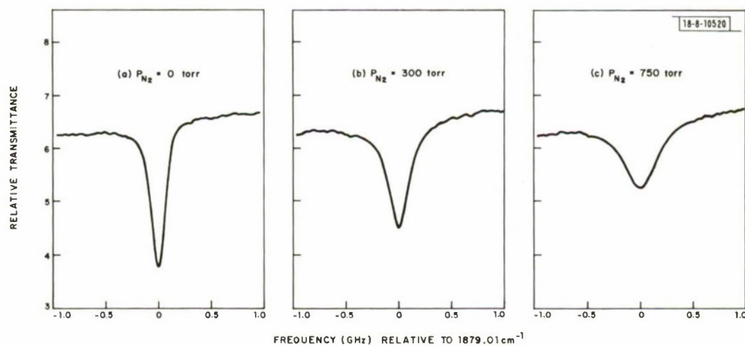
Fig. II-6. Water vapor-nitrogen pressure broadening ( P_{H_2O} = 1.95 torr).
