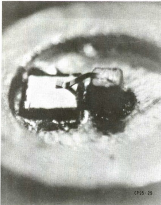
Fig.1-9. Photograph of a K a -bond GaAs IMPATT diode mounted on a copper heatsink and contacted with a 0.5 × 3-mil gold ribbon.
