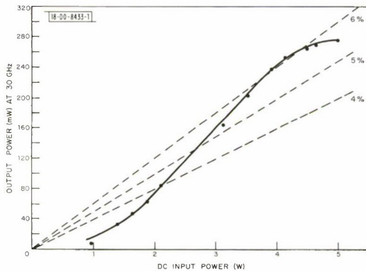
Fig. I-12. Oscillator output power plotted as a function of DC input power for a K_O -band GaAs IMPATT diode operating at 30 GHz. At each input power level, circuit tuning was adjusted for maximum oscillator power. Dashed lines shown are lines of constant power conversion efficiency.
