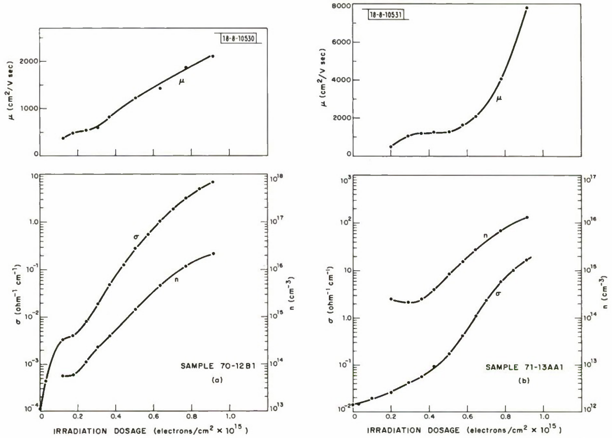
Fig. IV-7. Increase of conductivity, electron density and mobility as a function of electron irradiation (number of electrons per \text{cm}^2 ) for samples (a) 70-12B1 and (b) 71-13AA1. All measurements were made at 8°K.
