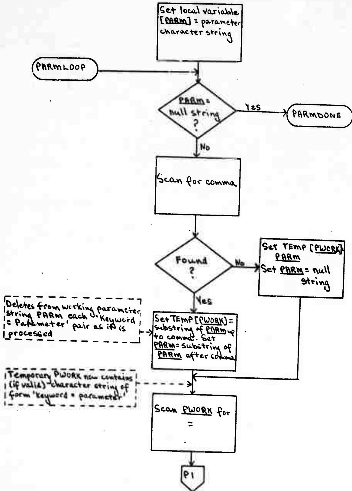
Figure C-1 : Parameter Processing (continued on next page)
