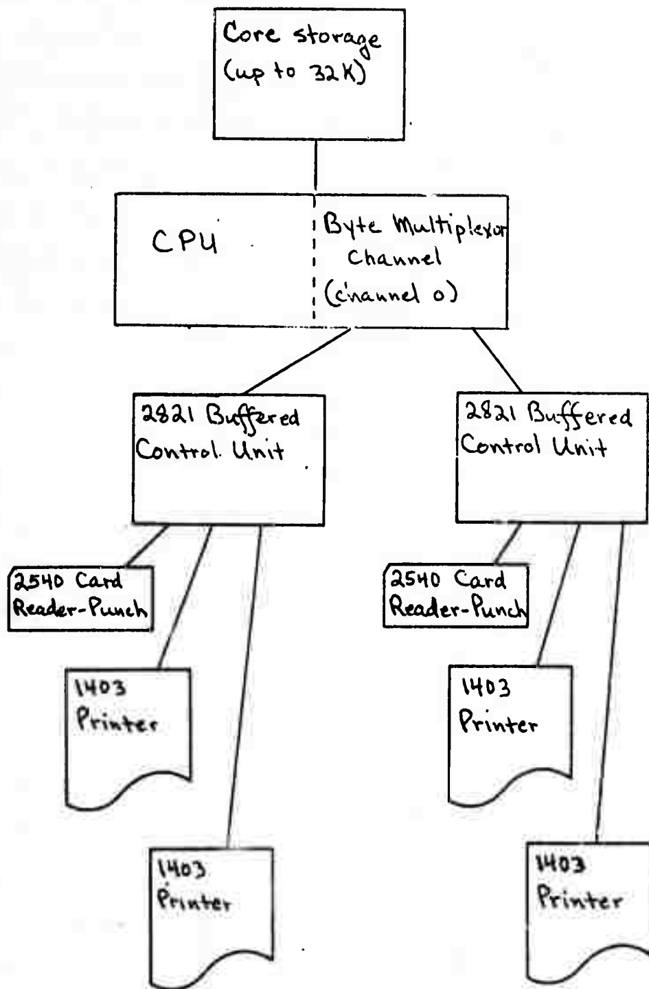
Figure 1 : Simulated Hardware Configuration
