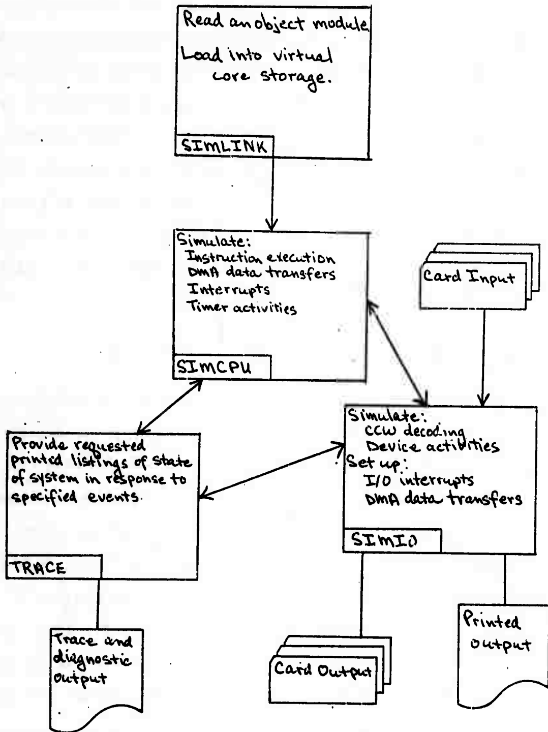
Figure 2 : Simulator Structure and Data Flow
