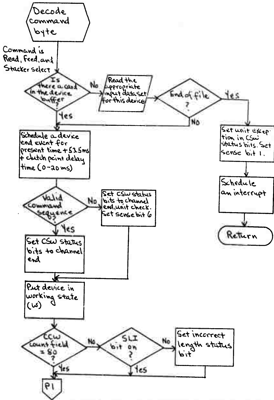
Figure C-12 : RFS Command to Card Reader (continued on next page)
