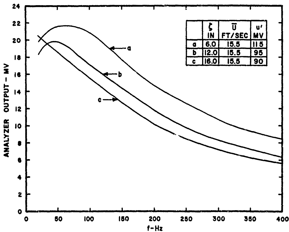
FIG. 10B. SPECTRA OF u AT DIFFERENT AXIAL LOCATIONS FOR TEST FLOW CONDITION "A".
