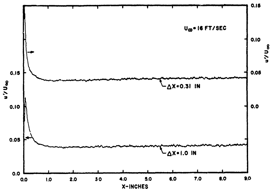
FIG. 46. AXIAL PROFILES OF u'/U_\infty FOR TWO SCREENS WITH X=0.31 AND 1.0 IN. IN TEST FLOW CONDITION "A".
