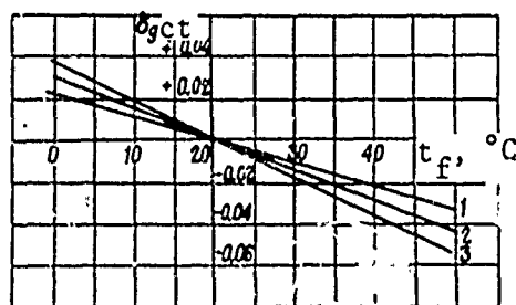
Figure 3. Relative Change in Fuel Feed \delta_{gct} as a Function of Temperature t_f with Fuel Pump Gear Against Stop and Full (maximum) Operating Speed: 1, type 61 diesel; 2, type M50F diesel; 3, type M503 diesel.
