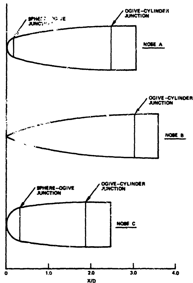
FIG. 3. Nose Configurations.
