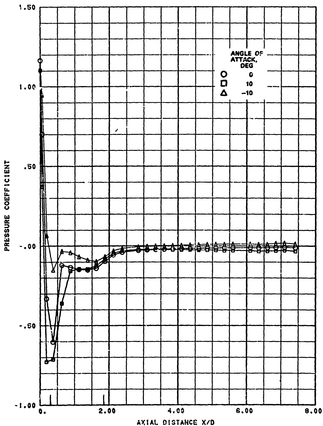
FIG. A-69. Longitudinal Pressure Distribution; Noose C, Mach 0.8, Roll Angle 15 Degrees.
