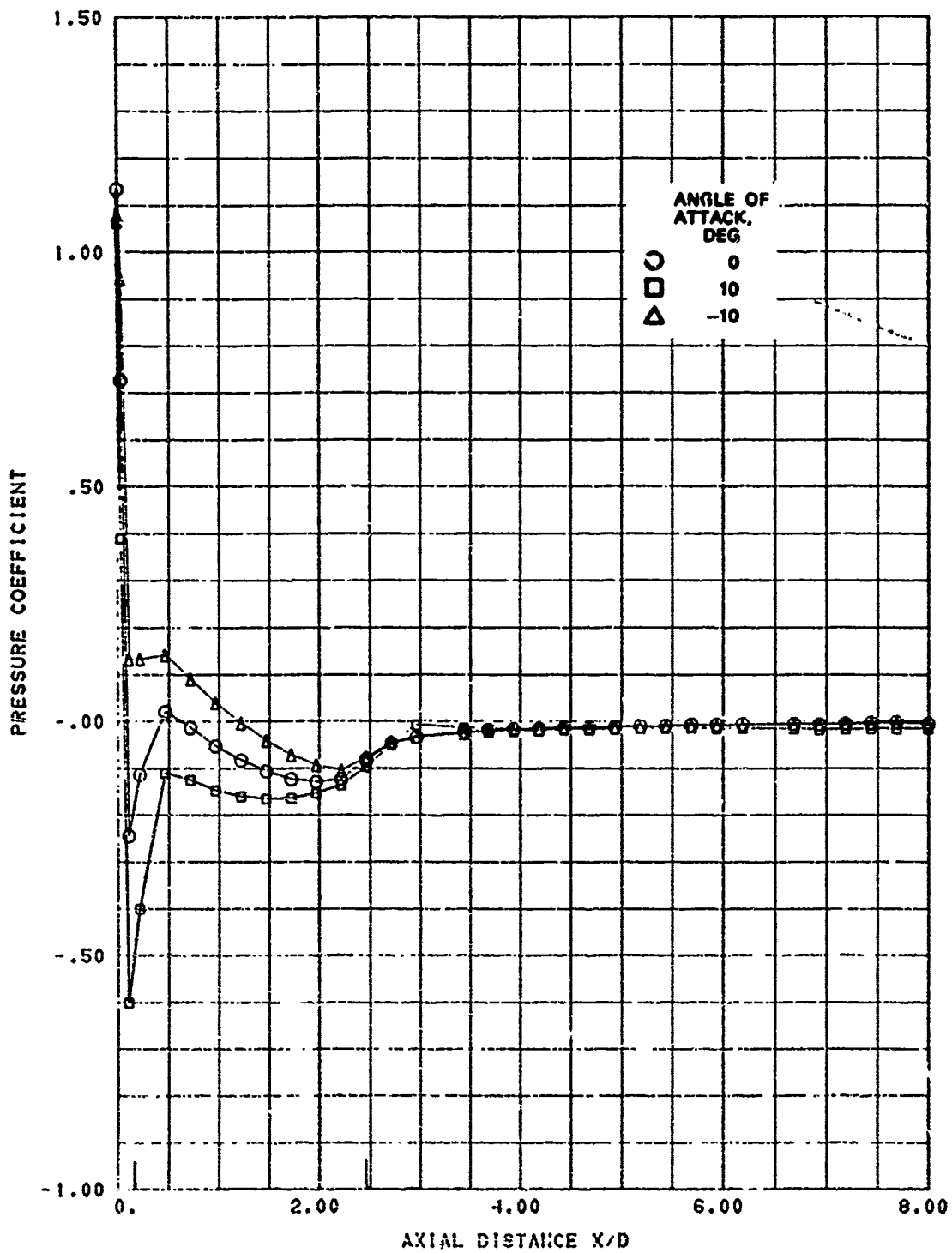
FIG. A-3. Longitudinal Pressure Distribution; Nose A, Mach 0.7, Roll Angle 30 Degrees.
