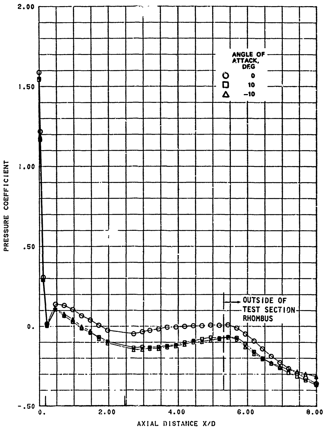
FIG. A-29. Longitudinal Pressure Distribution; No. A, Mach 1.52, Roll Angle 90 Degrees.
