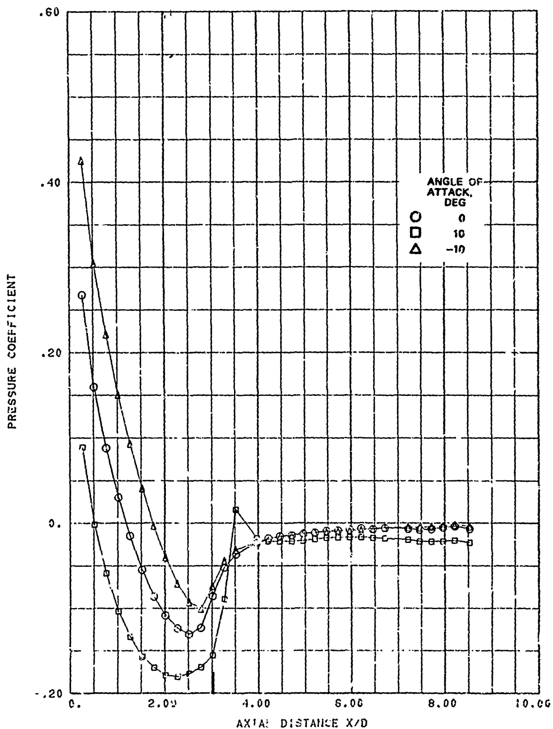
FIG. A-37 Longitudinal Pressure Distribution; N_{Re} B, Mach 0.7, Roll Angle 30 Degrees.
