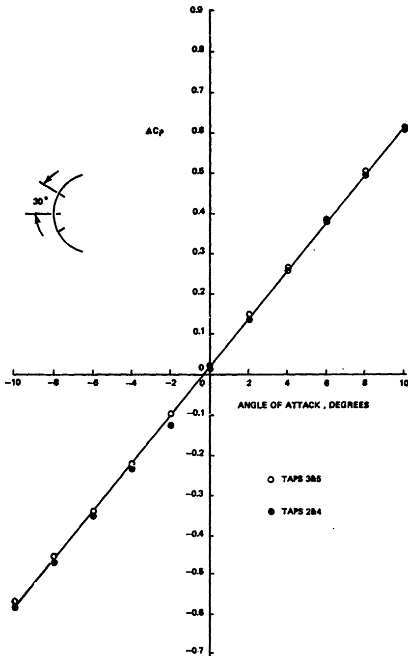
FIG. 31. Difference in Pressure Coefficient Across Nose Cap Versus Flow Angle; Nose C, Mach 0.8, 30 Degree Taps.
