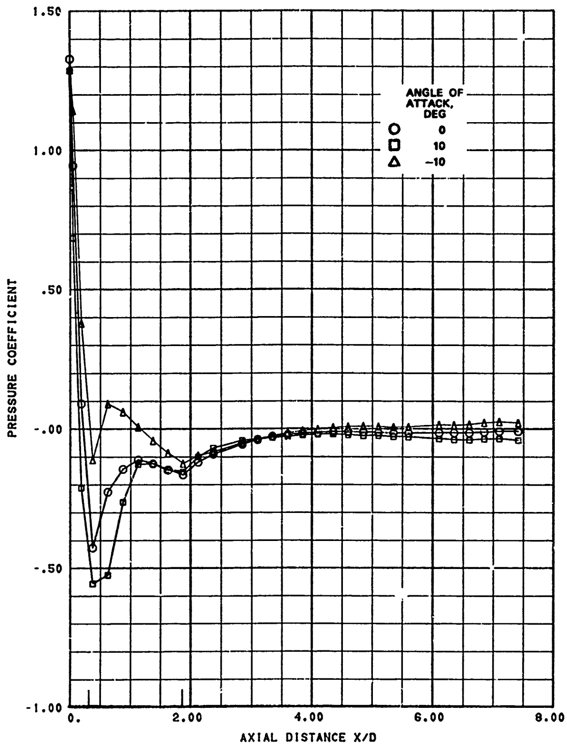
FIG. A-84. Longitudinal Pressure Distribution; Nose C, Mach 1.1, Roll Angle 15 Degrees.
