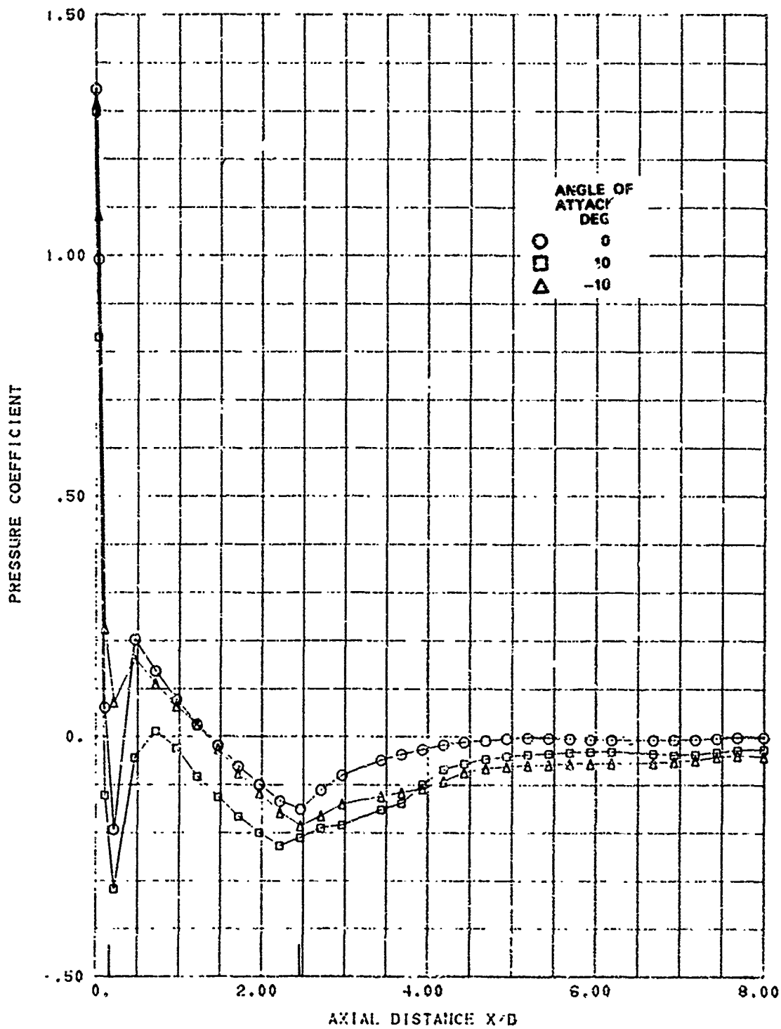
FIG. A-24. Longitudinal Pressure Distribution; Noce A, Mach 1.1, Roll Angle 60 Degrees.
