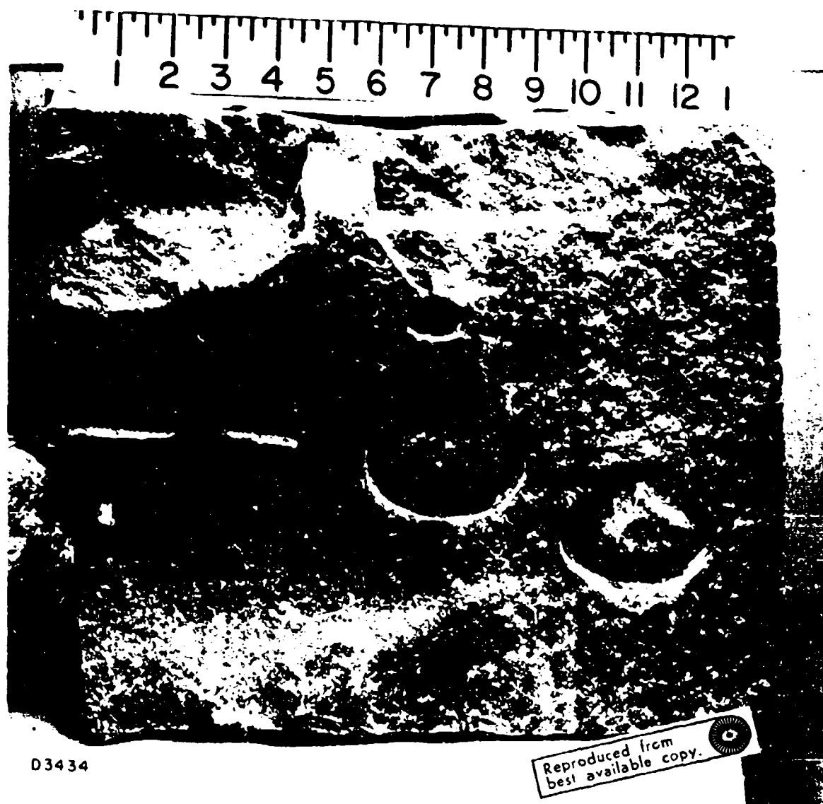
Figure 12 A 13 inch square block of quartzite exposed to rotating laser beams with power from .5 to 3 kilowatts.
