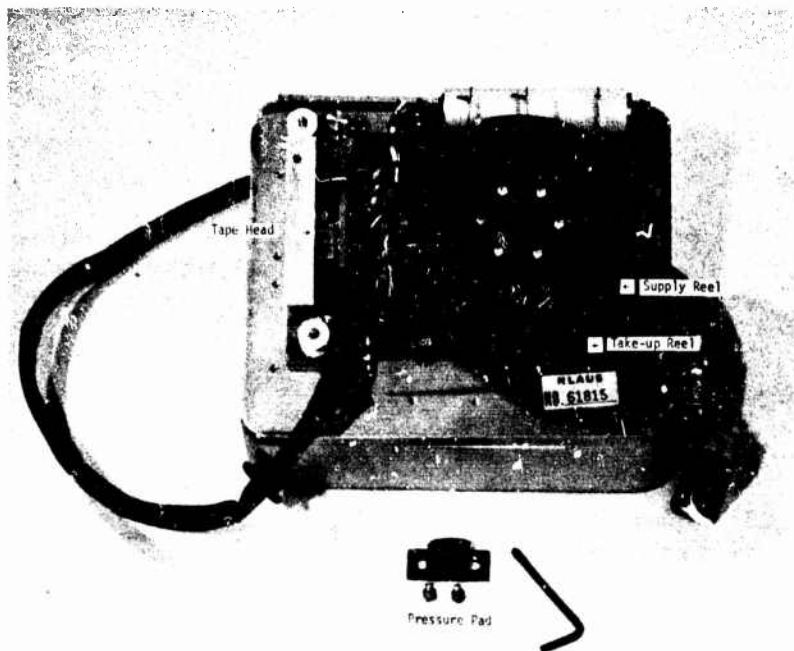
Figure 7a. Tape Loading (Front View).
