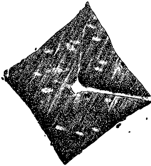
FIGURE 7 DPH indentation made at 2200F in unalloyed tantalum. 300X
