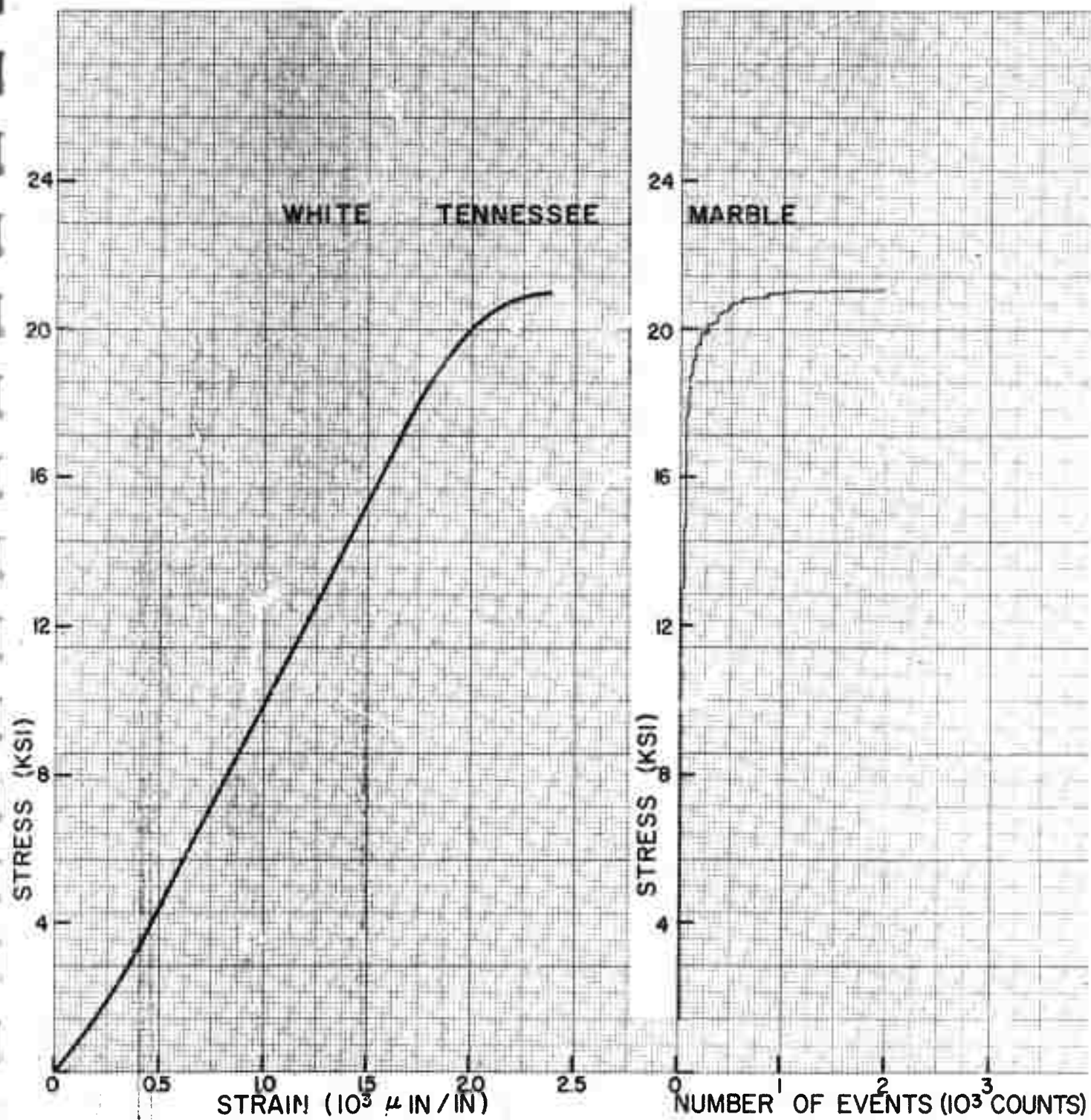
Figure 12 - Stress-strain curve and acoustic emission in monotonic compression (White Tennessee marble).
