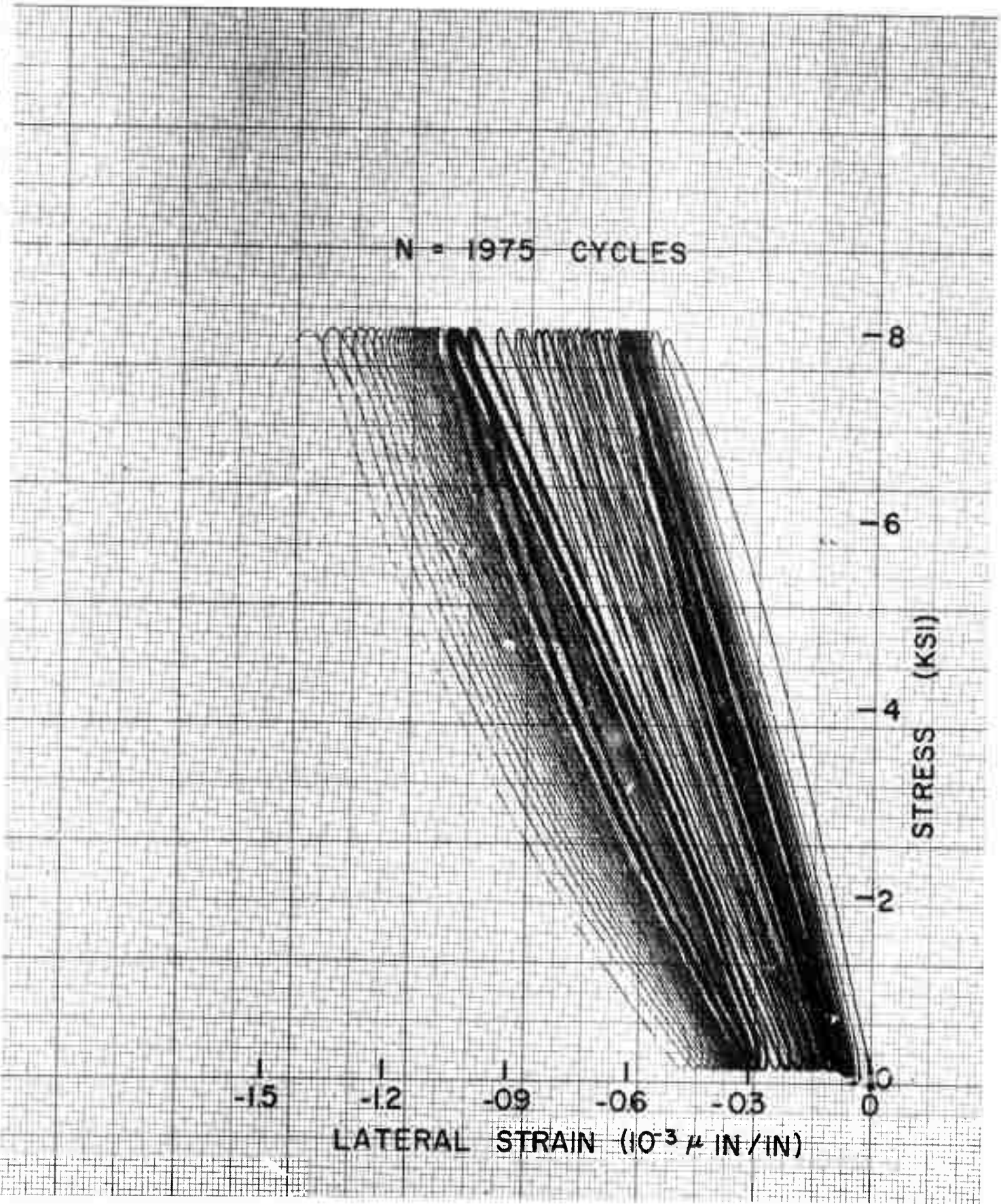
Figure 17 - Typical stress-lateral strain recording in cyclic loading of Indiana limestone.
