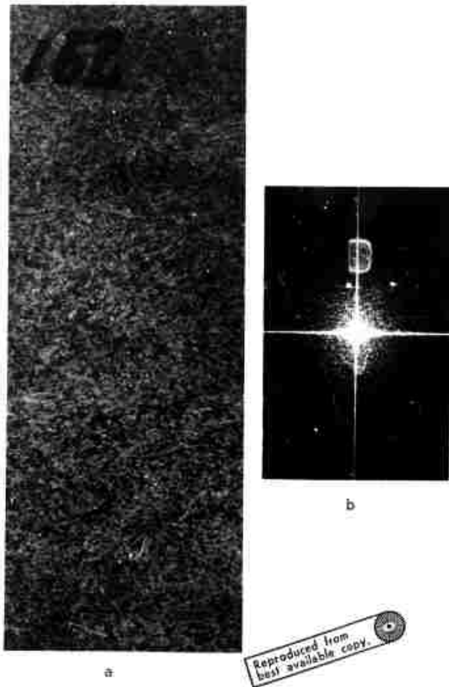
Figure 29. Indiana limestone - Optical analysis of a specimen after being cyclicly loaded to the accelerated tertiary stage, just before failure (upper peak stress = 75%).
