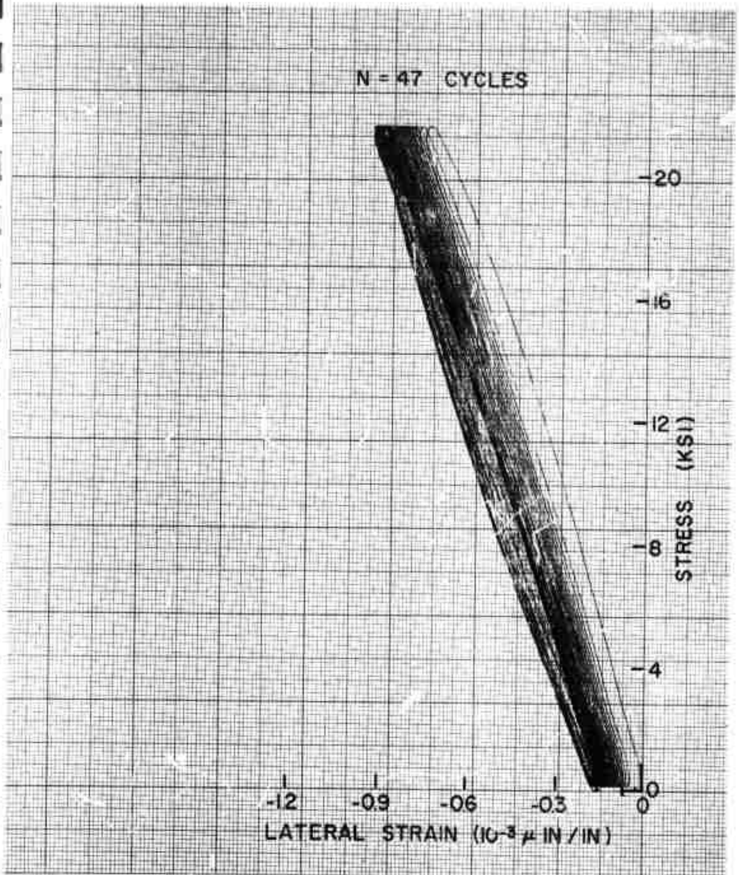
Figure 16 - Typical stress-lateral strain recording in cyclic loading of White Tennessee marble.
