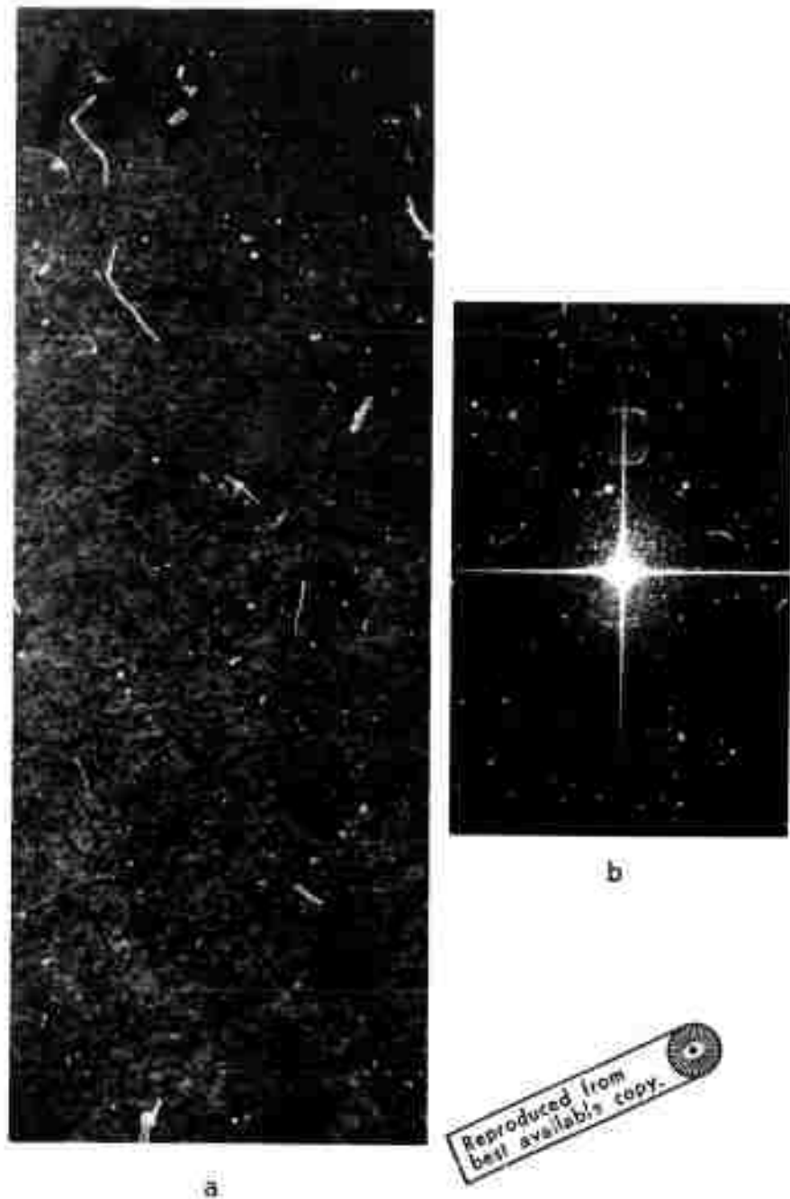
Figure 28. Indiana limestone - Optical analysis of a specimen after being cyclicly loaded to well within the steady state stage (upper peak stress = 75%).
