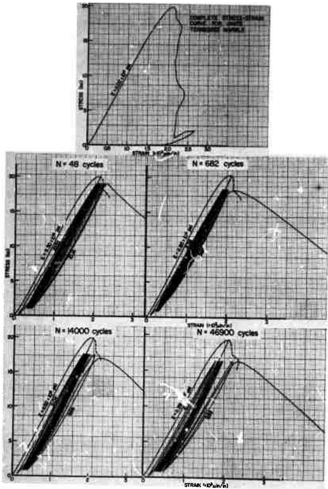
Figure 33 - Stress-strain curves for failed White Tennessee marble under cyclic loading (Broker line depicts the expected descending complete stress-strain curve).
