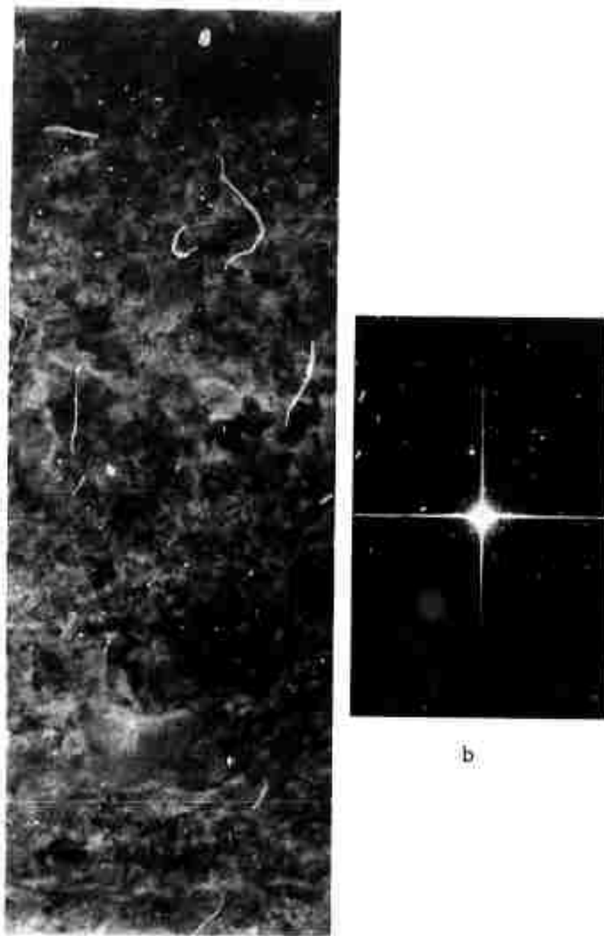
Figure 25 - White Tennessee marble - optical analysis of a specimen after 3,700 cycles of loading (See Figure 20).
