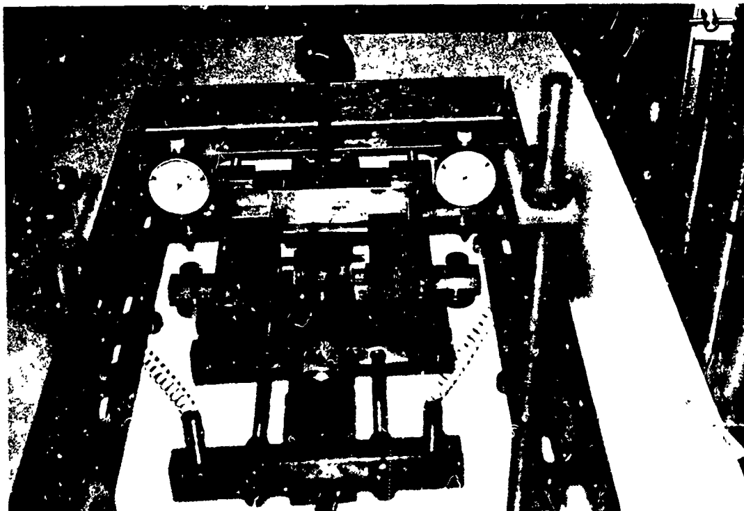
FIGURE 47. General view of the apparatus and one complete tensile rig
