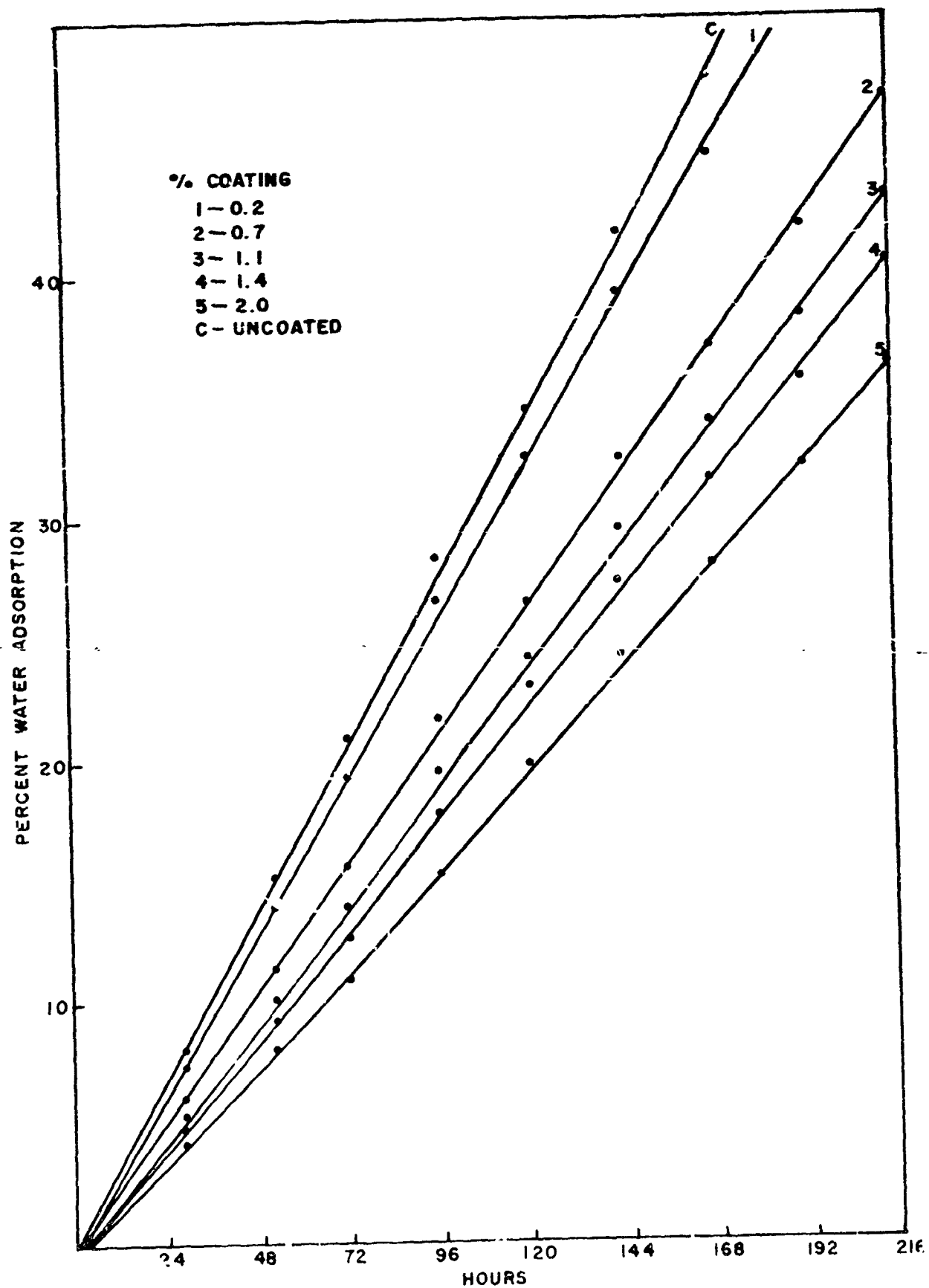
Fig 8 Rate of water absorption of Parylene-coated AN granules; at 100 °F (23 °C)
