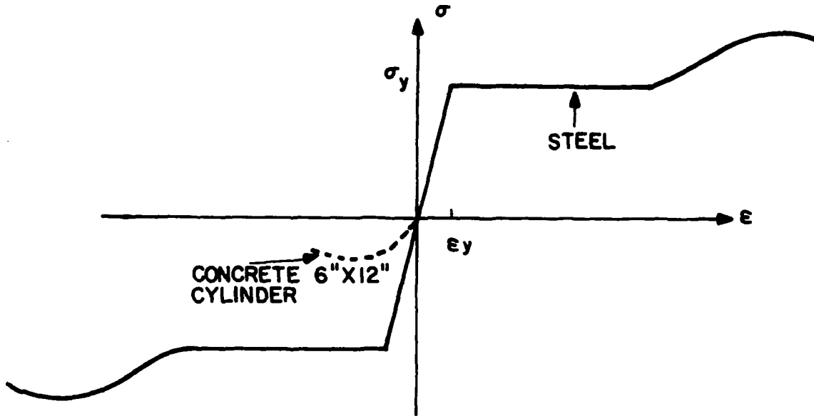
Figure 20. Stress-Strain Relations
