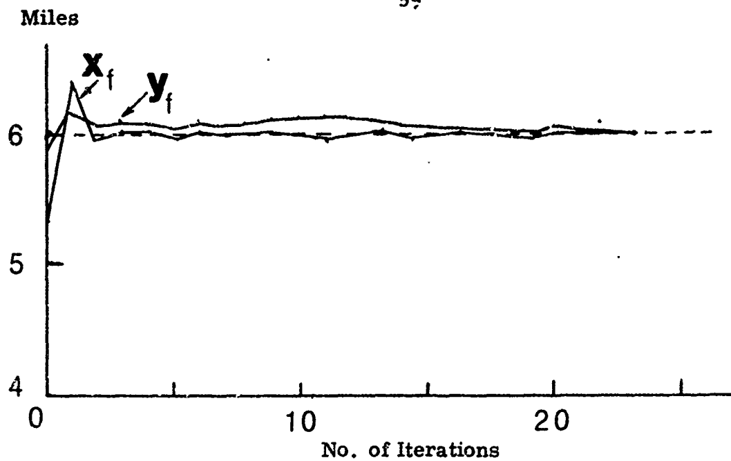
Fig.IV.1 Convergence of the Final Coordinates (Problem 4)
