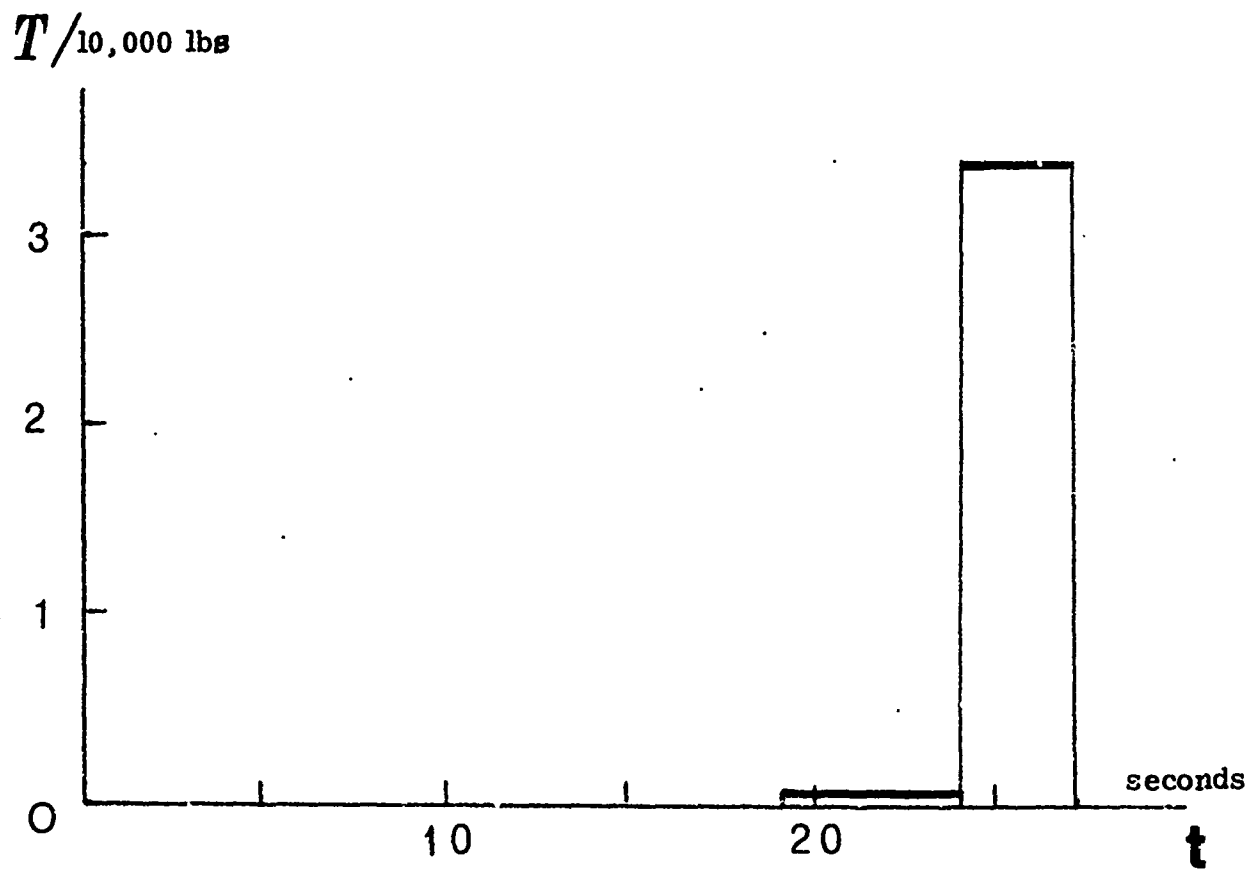
Fig.IV.3 Optimal Thrust Profile (Problem 4)
