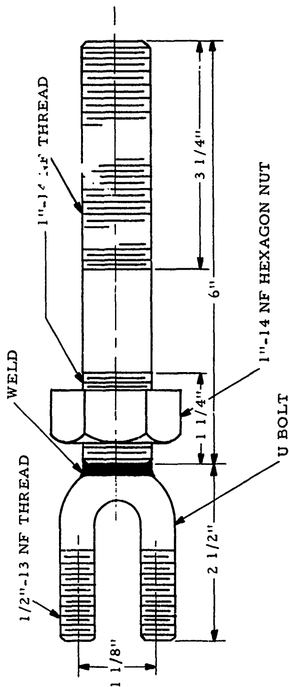
STUD & U BOLT ASSEMBLY - STEEL - 2 REQUIRED
