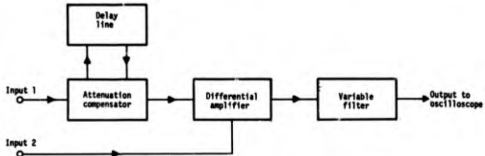
Fig. 14. Delay line instrumentation.
