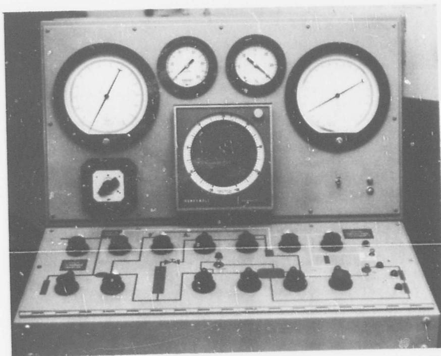
Fig. 6. Control console.
