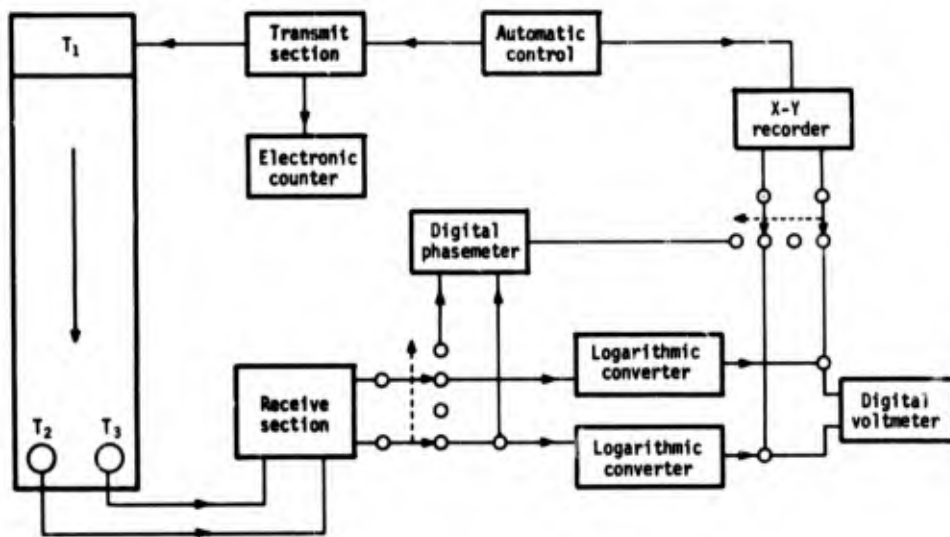
Fig. 1. Physical arrangement of sound source and transducers in the calibration chamber and block diagram of the measuring system for comparison calibrations in a standing-wave field. T_1 is the source, T_2 is the standard hydrophone, and T_3 is the unknown.
