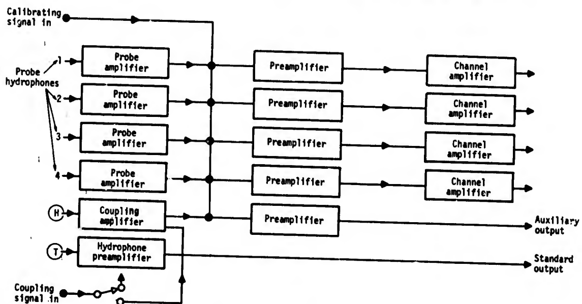
Fig. 13. Receiving section: H is the hydrophone being calibrated and T is the standard hydrophone.
