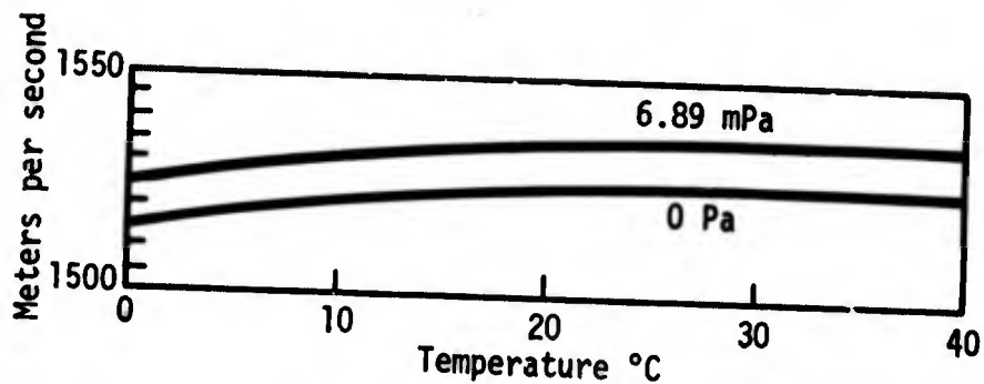
Fig. 10. Sound speed as a function of pressure and temperature in 33% ethylene glycol solution in System K.
