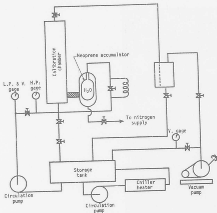
Fig. 5. Diagram of the external piping system.
