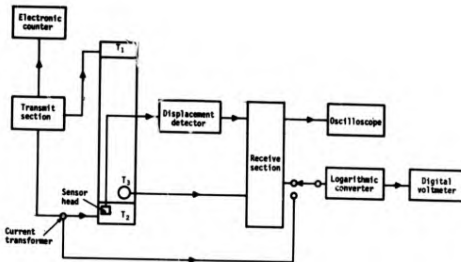
Fig. 3. Arrangement of instrumentation in the calibration chamber for the Two-Projector Null calibration, and block diagram of the electronic equipment. T_1 is the source, T_2 is the null projector, and T_3 is the hydrophone being calibrated.
