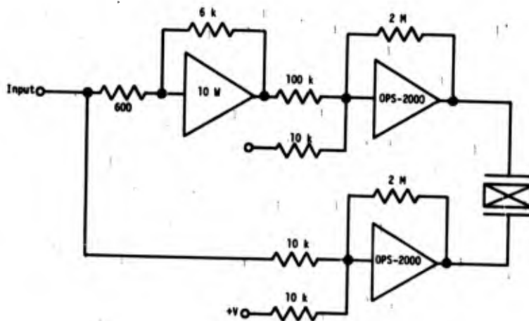
Fig. 12. High-voltage drive schematic.
