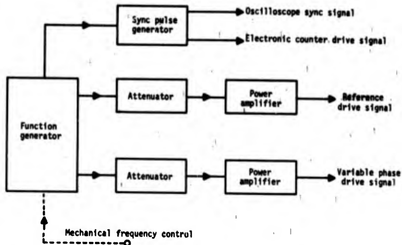
Fig. 11. Transmitting section.
