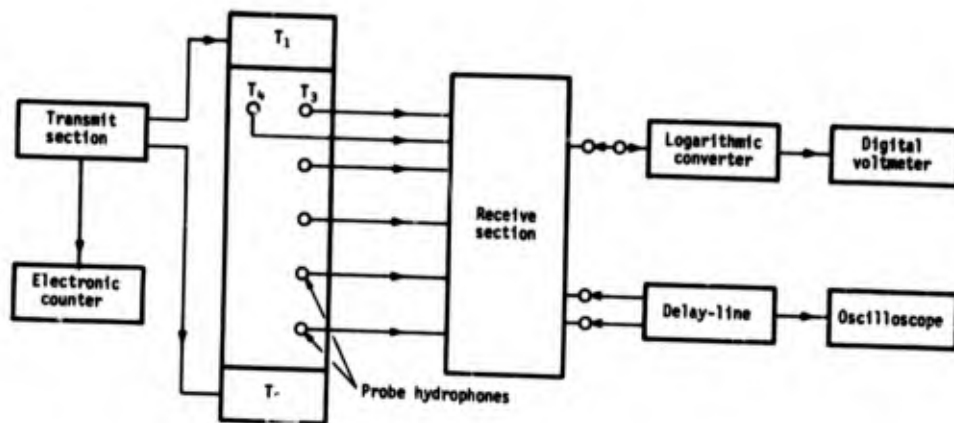
Fig. 2. Arrangement of instrumentation in the calibration chamber and block diagram of the electronic equipment for comparison calibration in a plane-wave field. T_1 is the active impedance transducer, T_2 is the source, T_3 is the standard hydrophone, and T_4 is the unknown.
