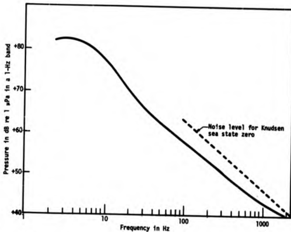
Fig. 9. Equivalent noise pressure level in water-filled System K.
