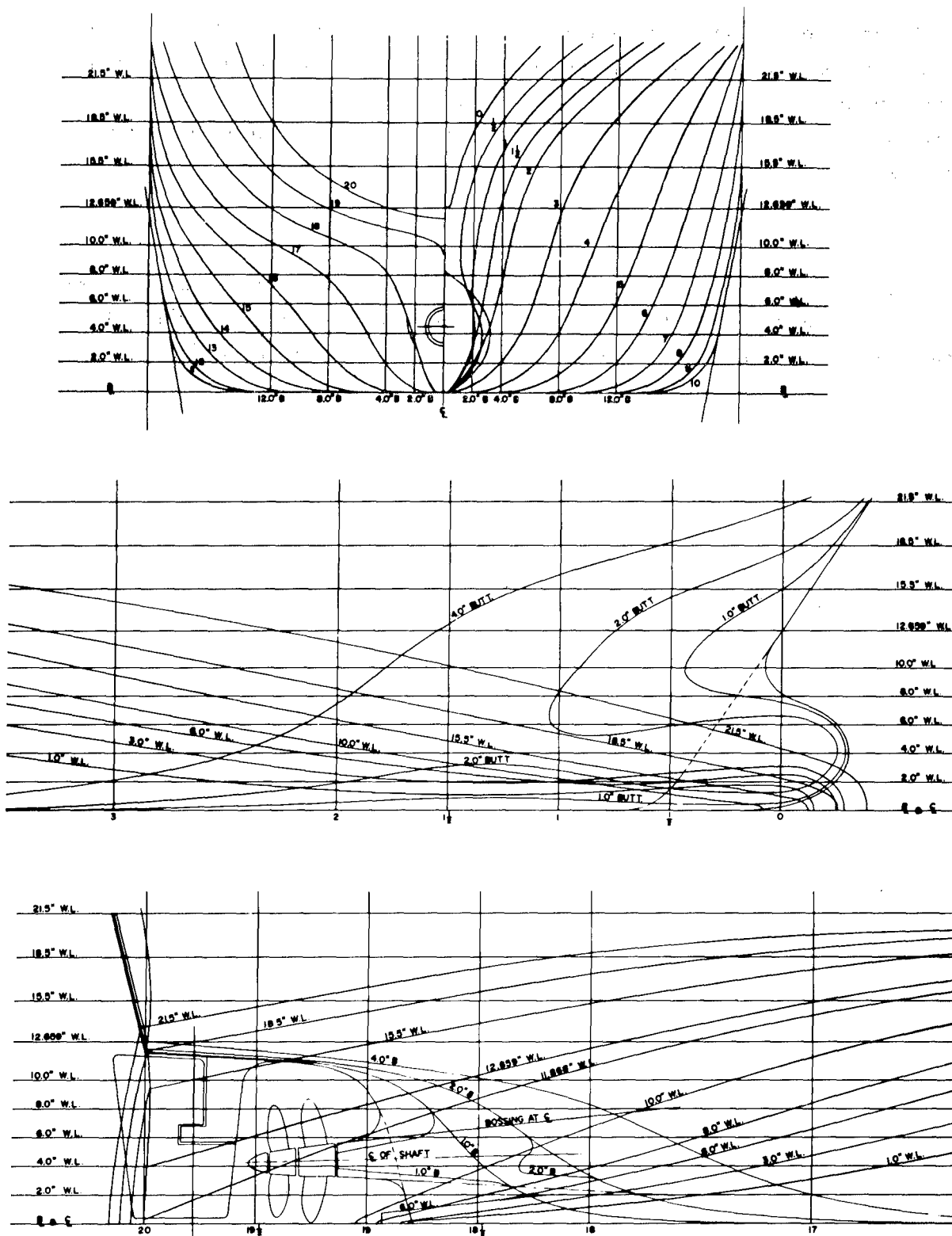
Figure 1 - Lines Drawing for Model 5218, Representing Contrarotating Single Rudder Containership Design
