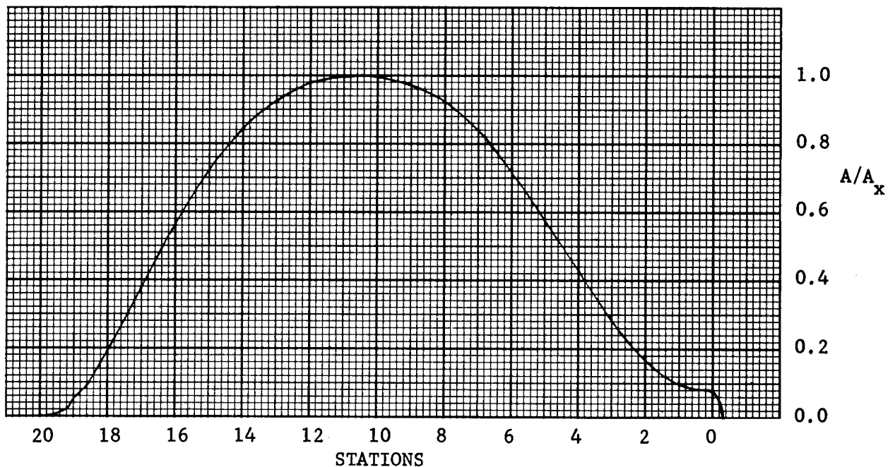
Sectional Area Curve
