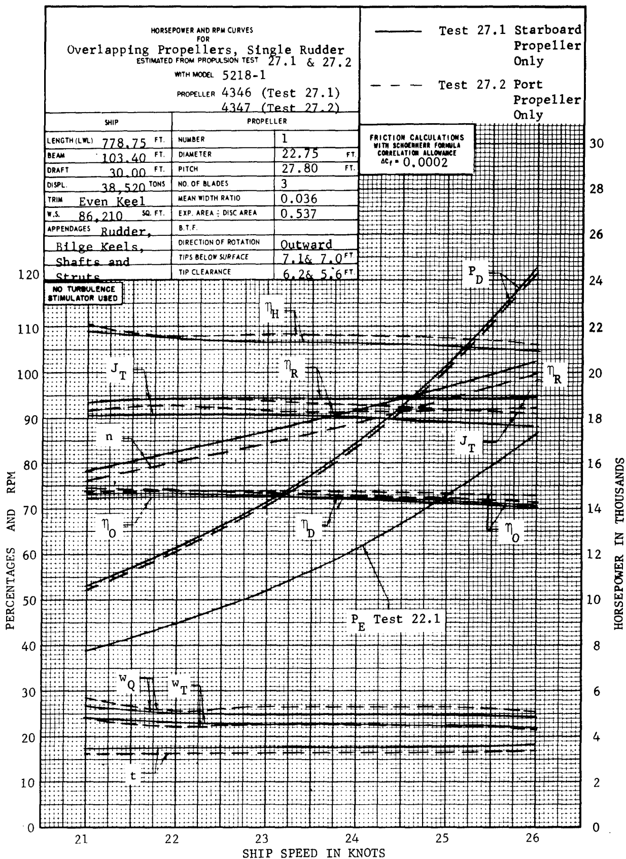
Figure 9 – Results from Propulsion Tests 27.1 and 27.2 with Overlapping Propeller, Single Rudder Arrangement—Starboard Propeller Only (Test 27.1) and Port Propeller Only (Test 27.2)—Stock Propellers 4346 (Starboard) and 4347 (Port) Outward Rotating
