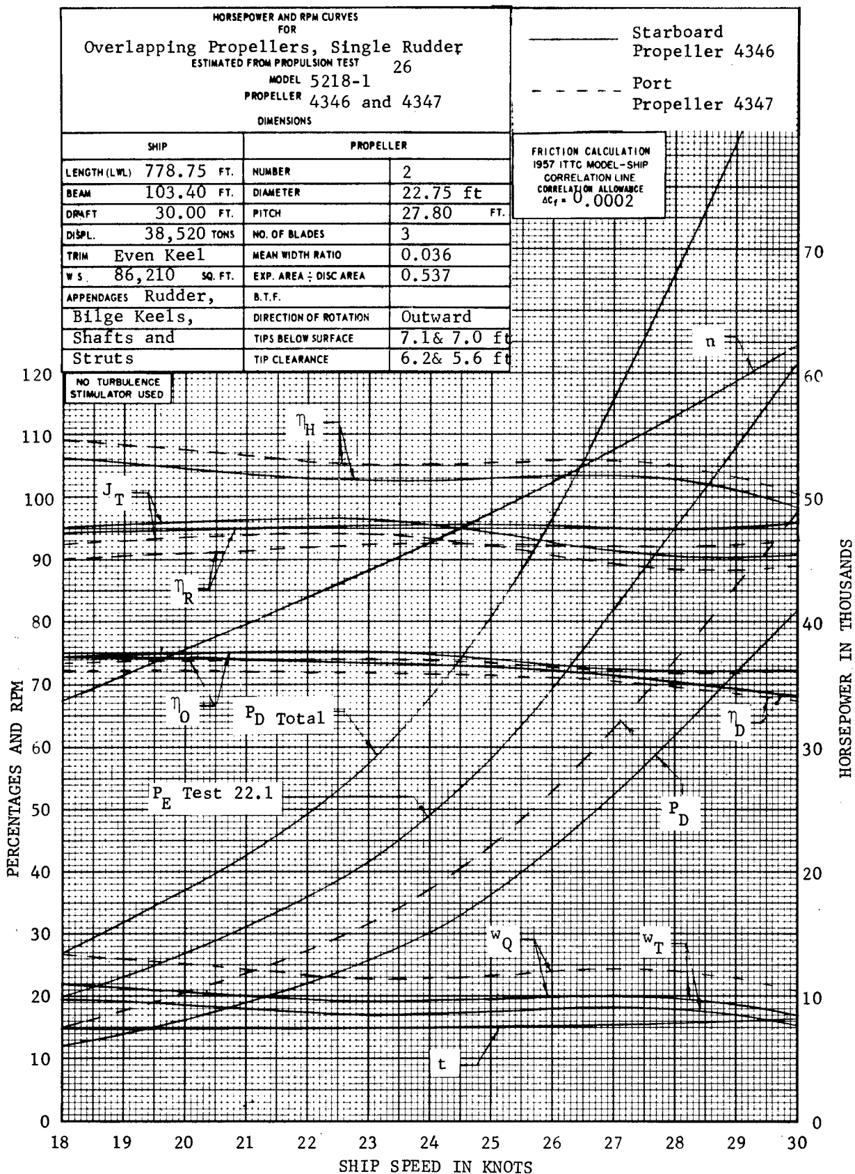
Figure 8 – Results from Propulsion Test 26 with Overlapping Propellers, Single Rudder Arrangement—Stock Propellers 4346 (Starboard) and 4347 (Port) Outward Rotating
