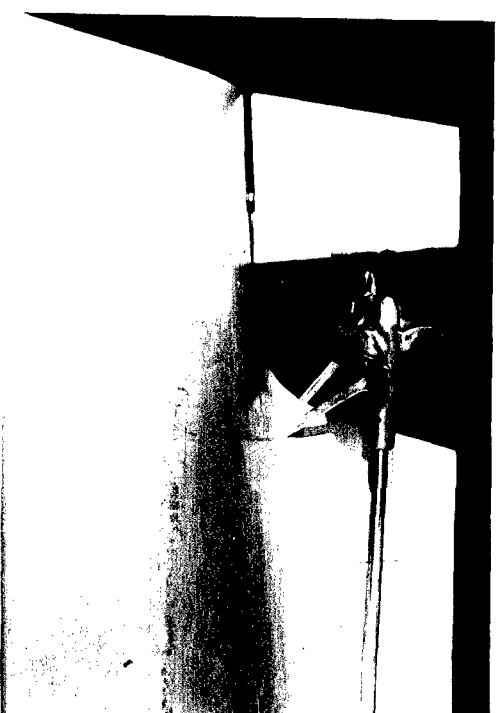
Figure 3 - Fitting Room Photographs of Overlapping Propeller Arrangement Model 5218-1, with Single Rudder (Stock Propellers 4346 and 4347)
