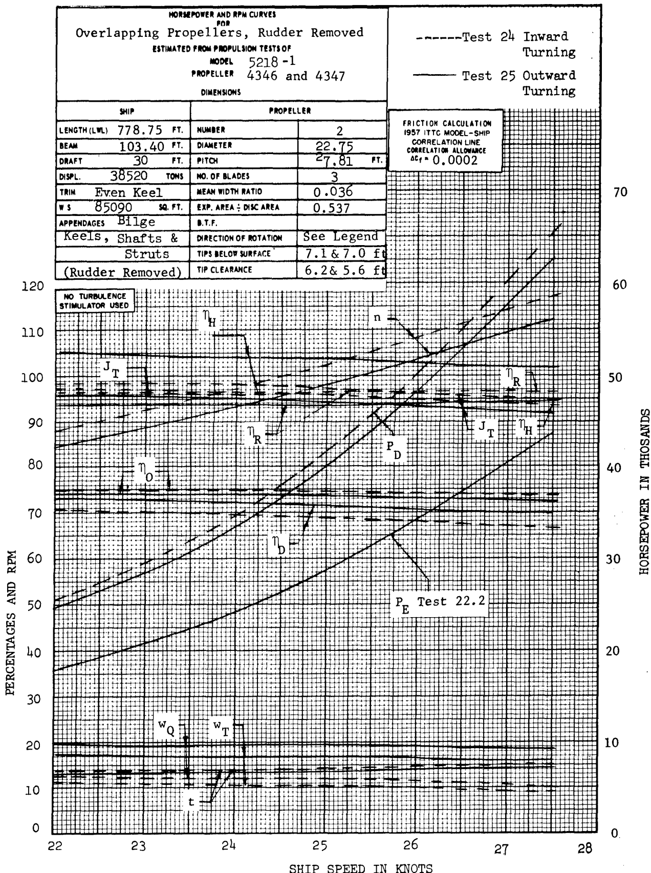
Figure 7 – Results from Propulsion Tests 24 and 25 with Overlapping Propeller Arrangement, Single Rudder Removed—Stock Propellers 4346 and 4347 Rotating Inward (Test 24) and Outward (Test 25)
