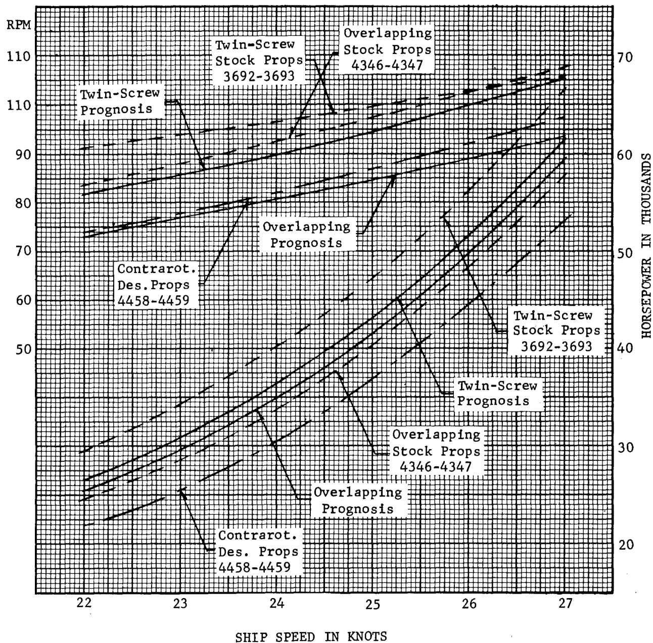
Figure 10 – Comparison of Performance of Overlapping Propeller Arrangement with Single Rudder (Model 5218-1), Contrarotating Design with Single Rudder (Model 5218), and Twin-Screw Arrangement (Model 5209)
