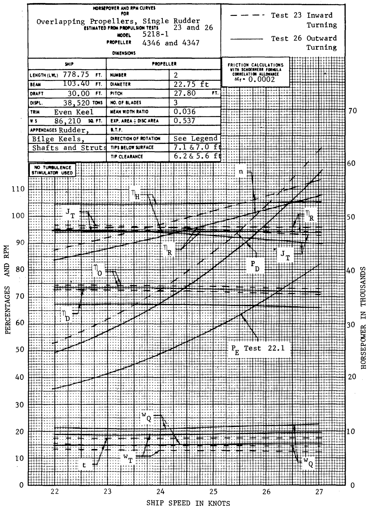
Figure 6 – Results from Propulsion Tests 23 and 26 with Overlapping Propellers, Single Rudder Arrangement—Stock Propellers 4346 and 4347 Rotating Inward (Test 23) and Outward (Test 26)
