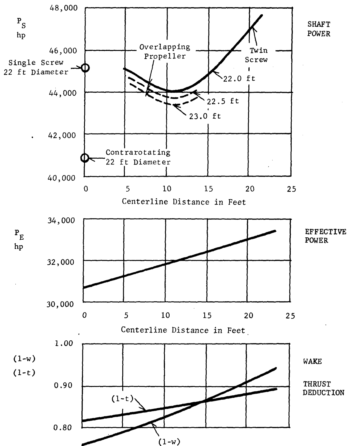
Figure 11 – Predicted Performance of Twin-Screw Propulsion Arrangement as a Function of Propeller Shaft Distance from Centerline
