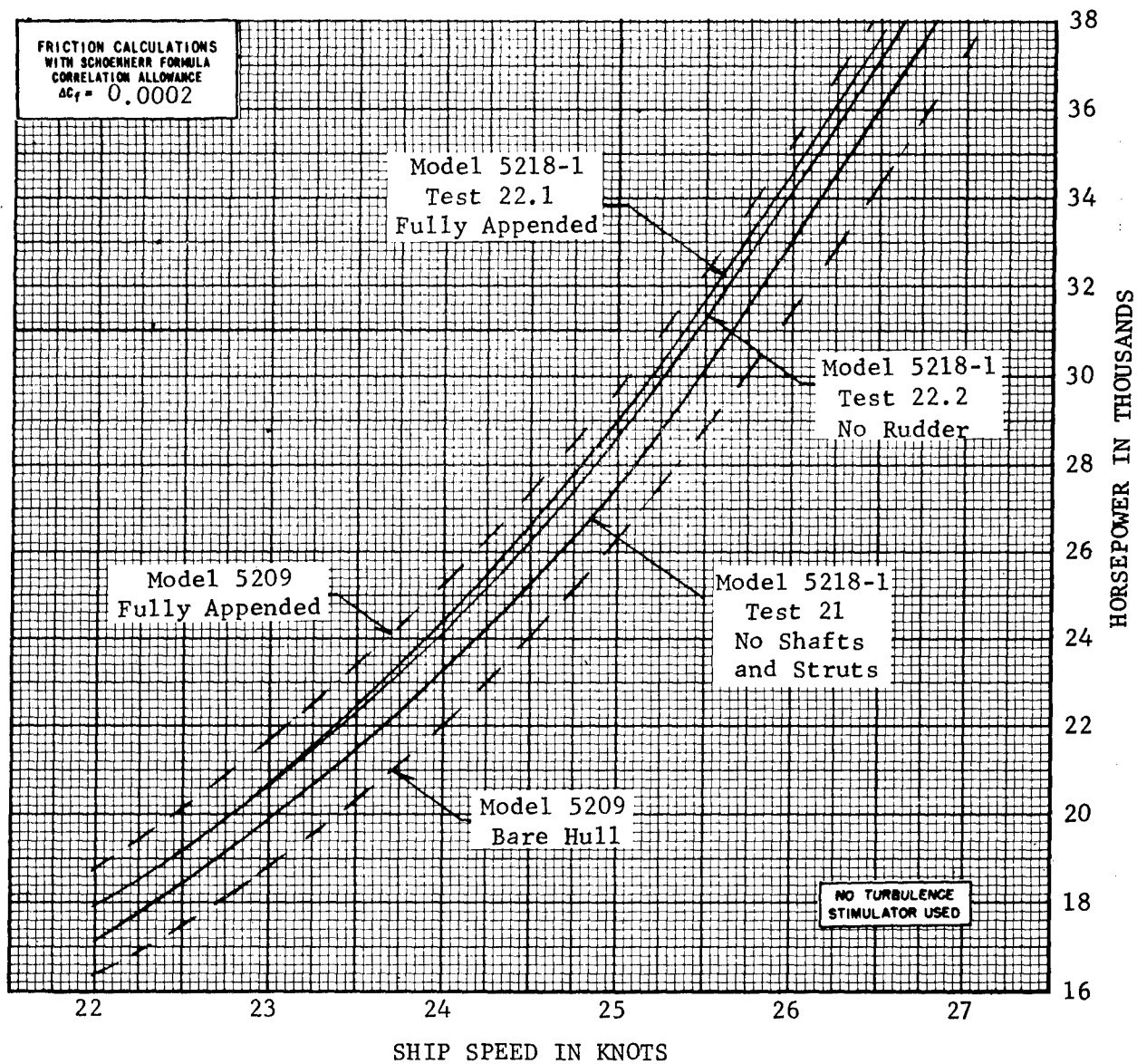
Figure 5 - Comparison of Effective Horsepower Curves for Overlapping Propeller Design Model 5218-1 and Twin-Screw Design Model 5209
