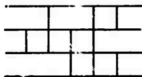
Figure 1.3.1 Sorting network.
