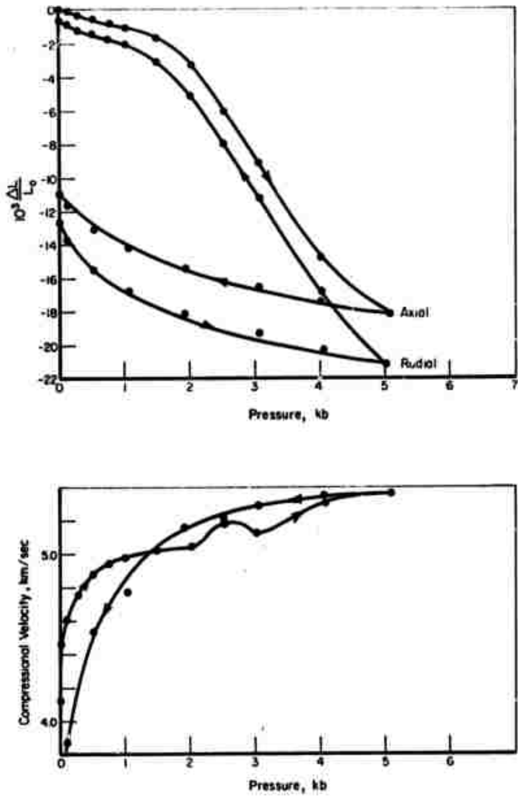
FIGURE 8. SALEM LIMESTONE, DRY (5-KBAR CYCLE)
