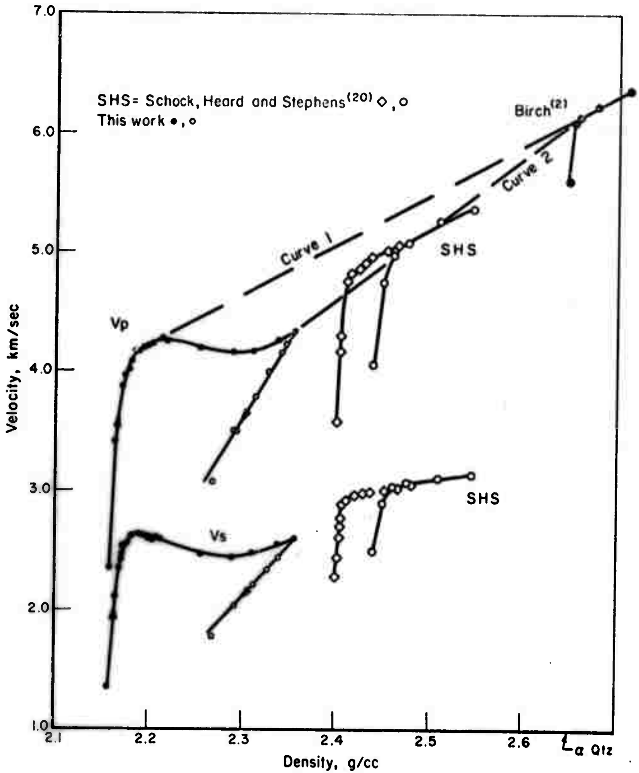
FIGURE 31. VELOCITY-DENSITY PLOTS FOR SANDSTONE
