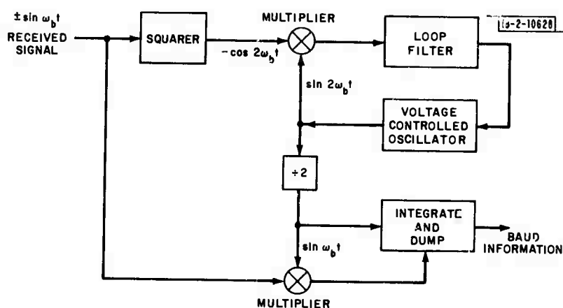
Fig. 5. PSK demodulator.
