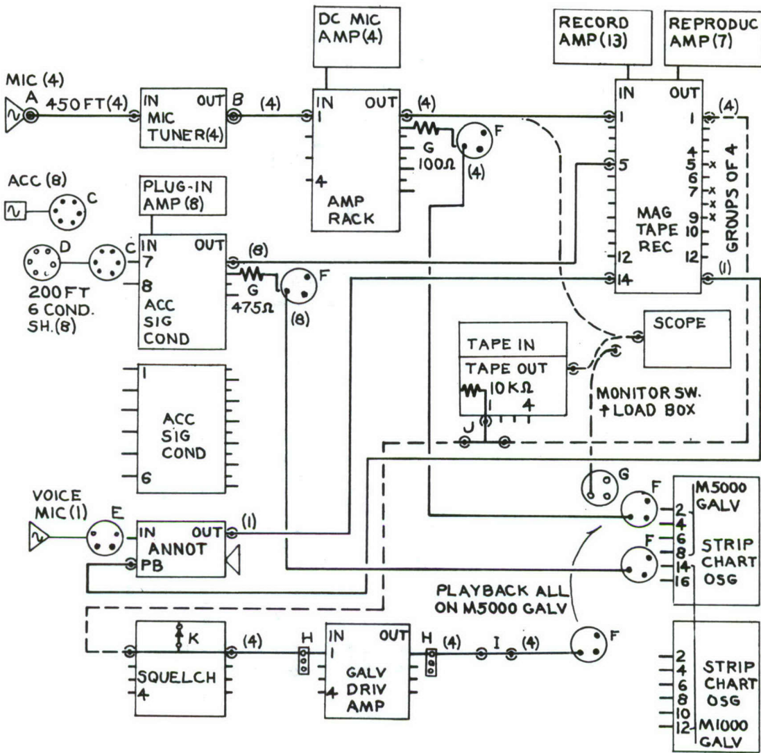
APPENDIX I, FIG. 22 SIGNAL CONNECTIONS NASA-USDA INSTRUMENT SYSTEM FOR SONIC BOOM OVERPRESSURE + STRUCTURAL ACCELERATION. J.R. MENEAR - AERD, ARS, USDA AT SMIS, EMIB, IRD, NASA-LANGLEY RES. CTR. JA70
