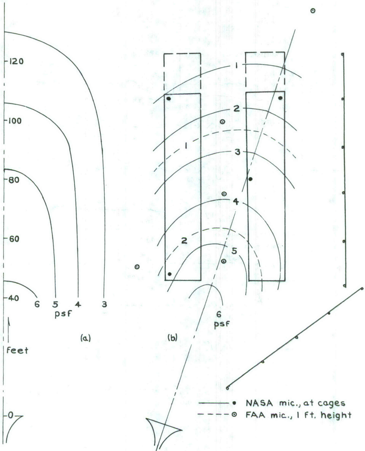
Figure 13.--Peak overpressure field of sonic boom simulator, in pounds per square foot. (a) Clear field calibration, 4 feet above level gravel; (b) Simulated Boom 1, 12 May 70.
