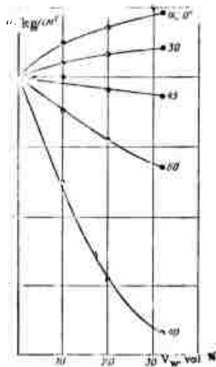
Fig. 4. Titanium impact viscosity as a function of molybdenum volumetric wire content, E_v .
