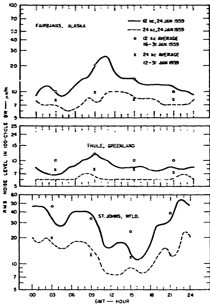
FIG. V-1 DIURNAL RMS NOISE LEVEL VARIATION, JANUARY 1959
