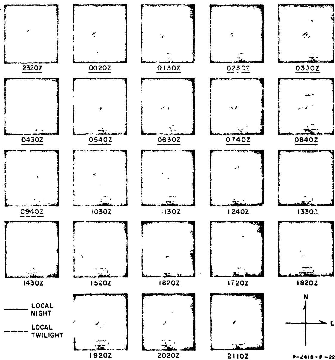
FIG. G-12 TEN MINUTES INTEGRATED DF AT ST. JOHNS, NEWFOUNDLAND—14-15 MARCH 1959—10 mv/m
