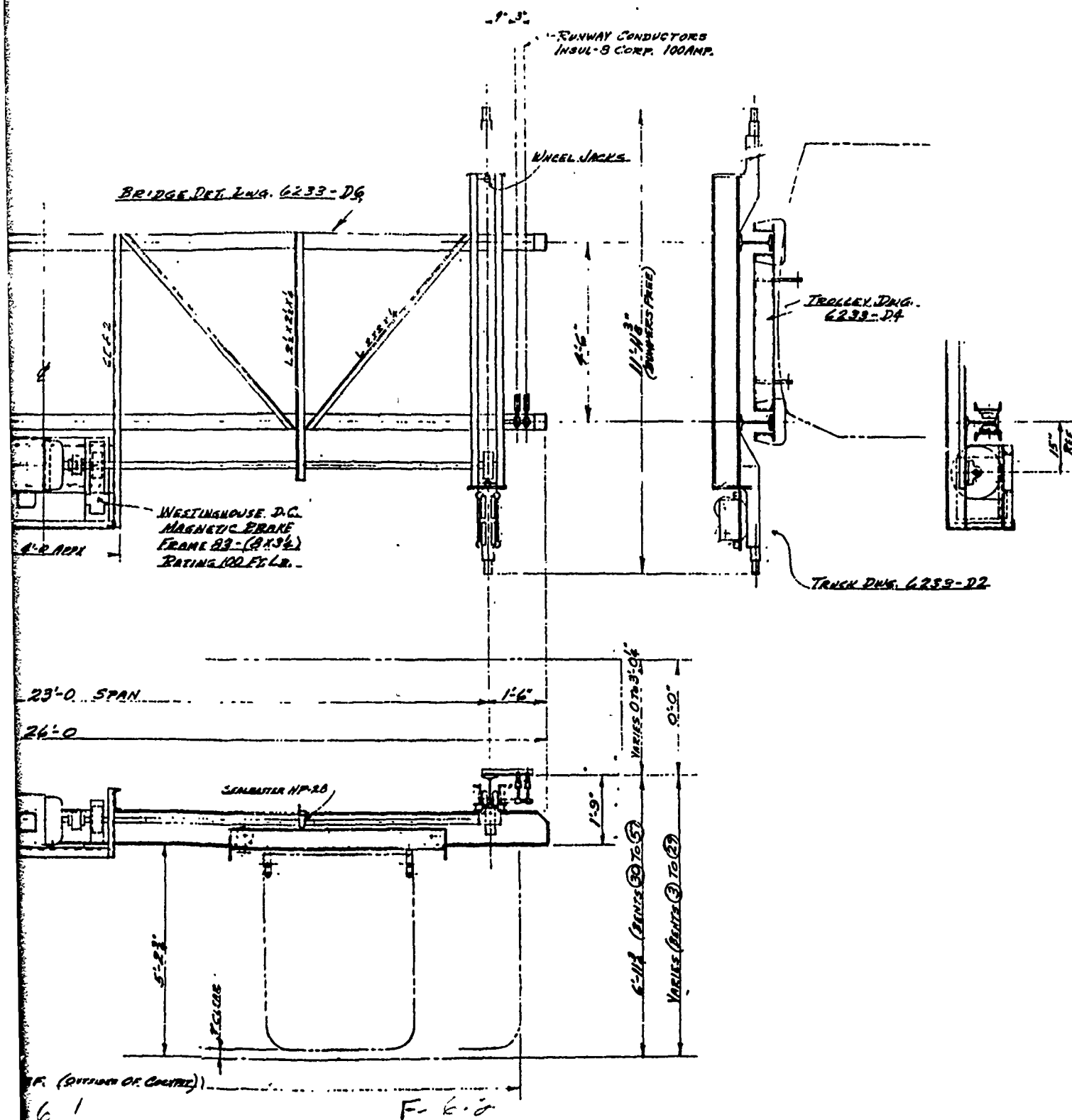
Fig. 6 - Tramway carriage structural features.
