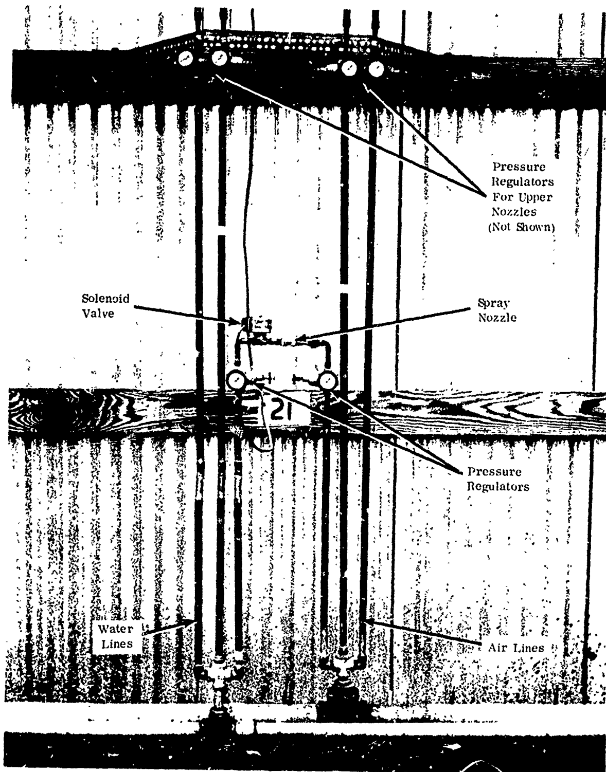
Fig. 14 - Typical nozzle manifold assembly.
