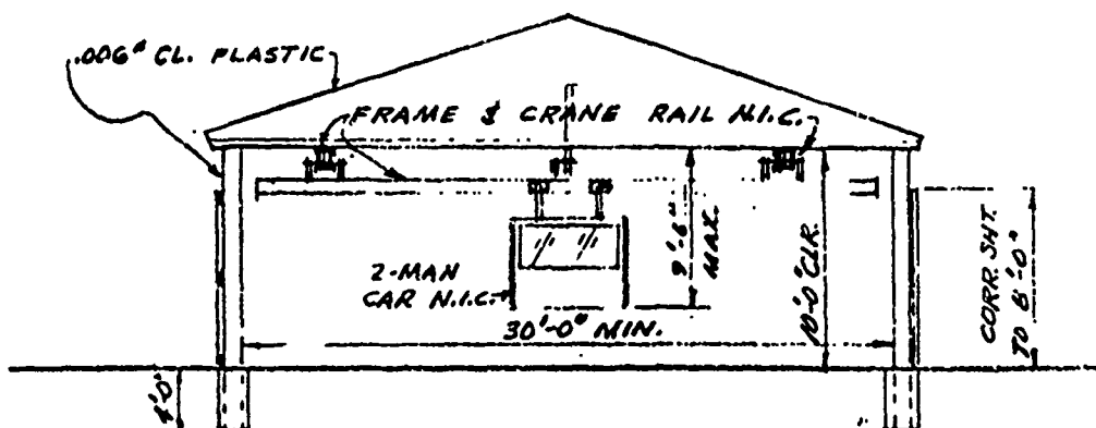
SECTION C-C SCALE : \frac{1}{8}" = 1'-0"
