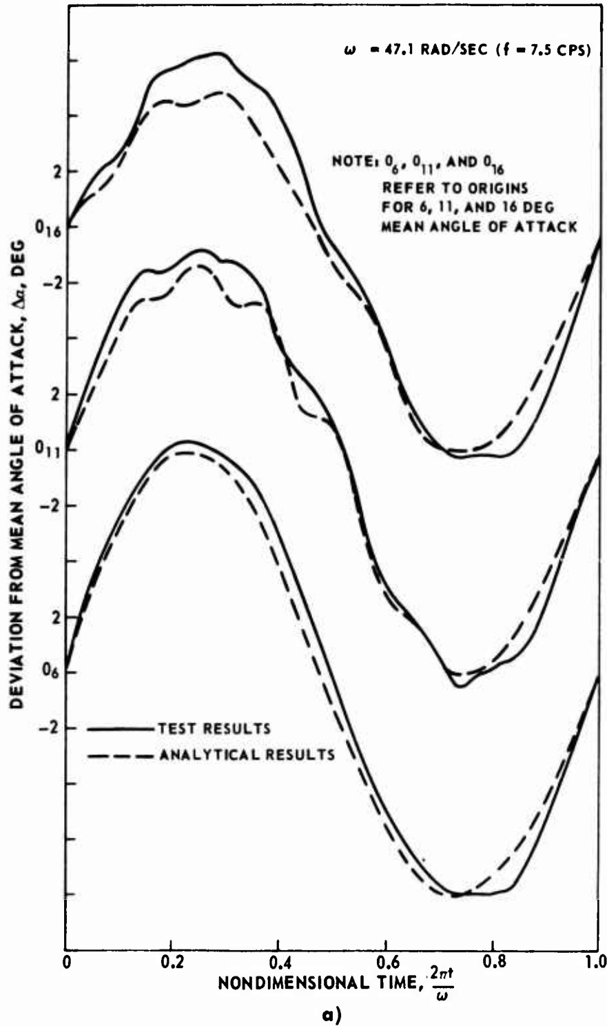
Figure 40. Comparison of Experimental and Analytical Time Histories for Flexible Airfoil With f_{\alpha} = 52 \text{ CPS} .
