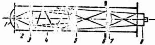
Fig. 40. Optical diagram of the variospectrometric underwater irradiance-meter (VARIPO): 1 - port; 2 - receiving slot; 3 - lens system; 4 - Amici prism; 5 - objective; 6 - normalizing diaphragm; 7 - lens, 8 - photoelectron multiplier (PEM).
