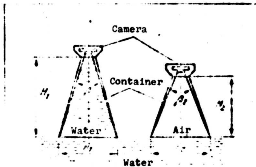
Fig. 62. Adapters for photography in turbid water: a - water filler container; b - air filler container A_1 = A_2 , but \beta_1 < \beta_2 and thus H_1 > H_2 .
