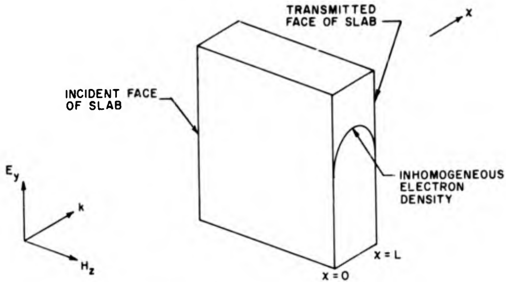
Figure 1. Plane Wave Incident on Inhomogeneous Reentry Plasma Sheath
