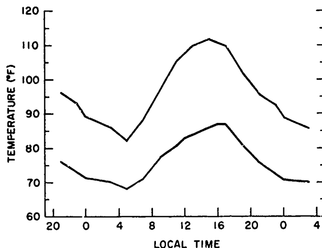
Figure 4. Composite of Five Daily Cycles of High Temperature and Dew Point for Abadan, Iran. An example of a high, fluctuating dew-point cycle and its associated very hot temperature cycle
