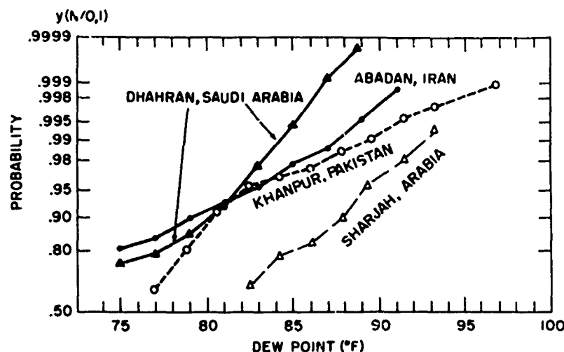
Figure 6. Cumulative Frequency Distributions (Upper Portions) for Dhahran, Abadan, Khanpur and Sharjah
