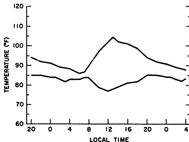
Figure 1. Composite of Five Daily Cycles of High Temperature and Dew Point for Dhahran, Iran. An example of a high, relatively steady dew point
