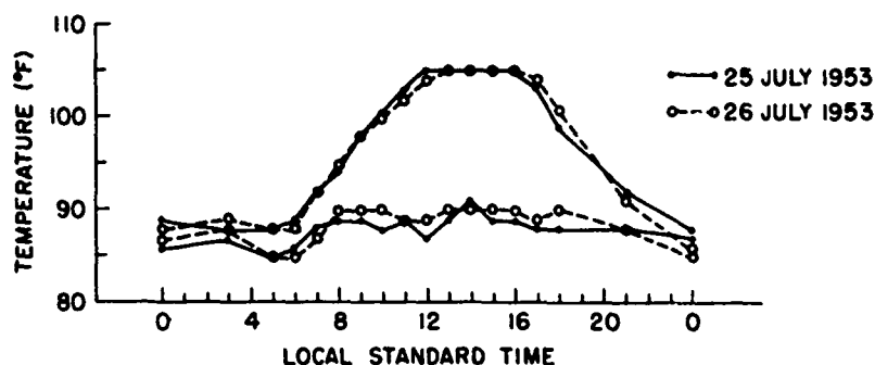
Figure 7. Hourly Temperatures and Dew Points for Two Consecutive Days of Very High Humidities at Abadan, Iran
