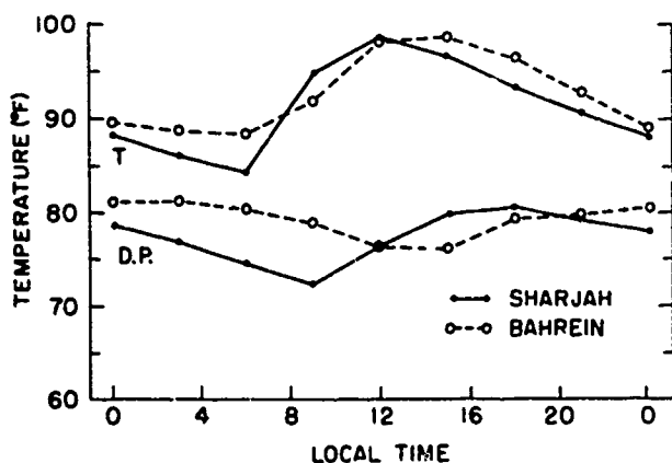
Figure 5. August Mean Monthly Dry-Bulb and Dew-Point Temperature Cycles for Sharjah and Bahrein, Arabia, Based on 1962-1966 Date (After Watt, 1968)
