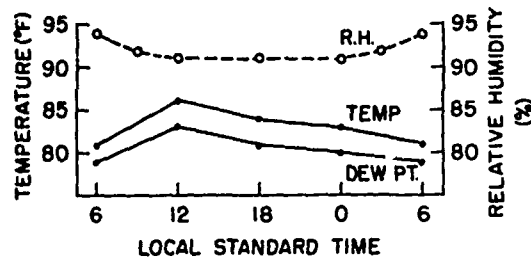
Figure 10. Withstanding High Absolute Humidity (Dew Point) With Associated Temperature, Resulting Relative Humidity and Insolation. Such conditions are found in coastal, moist tropical locations and are approximately duplicated for a month. Adjacent months will experience slightly less humid extremes
