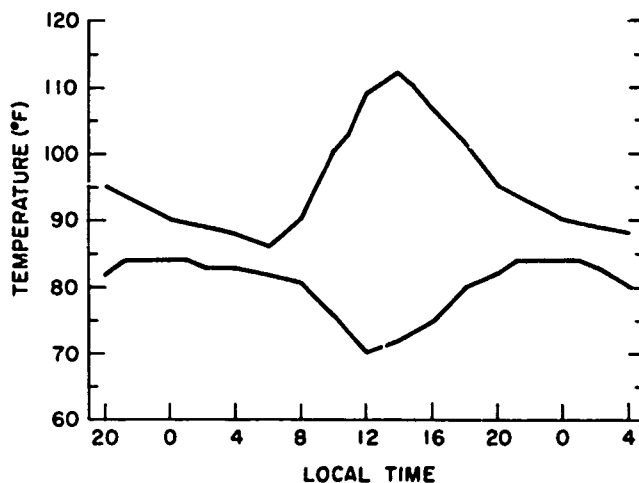
Figure 2. Composite of Five Daily Cycles of High Temperature and Dew Point for Dhahran, Iran. An example of a high, fluctuating dew-point cycle and its associated very hot temperature cycle
