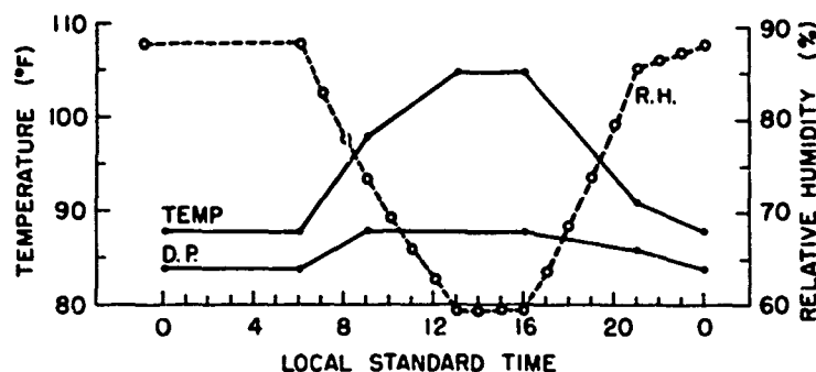
Figure 8. Diurnal Cycle of Dew Point, Temperature and Relative Humidity Associated With the 1 Percent High Absolute Humidity Operational Extreme (which is a dew point of 88° in a coastal desert location, Abadan, Iran)
