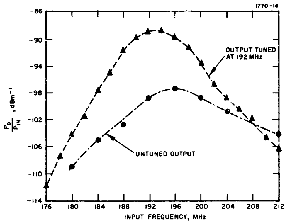
Fig. 50. Narrow Band Convolver: Convolution Efficiency for 5 \mu\text{sec} Pulses, 195 MHz Design.
