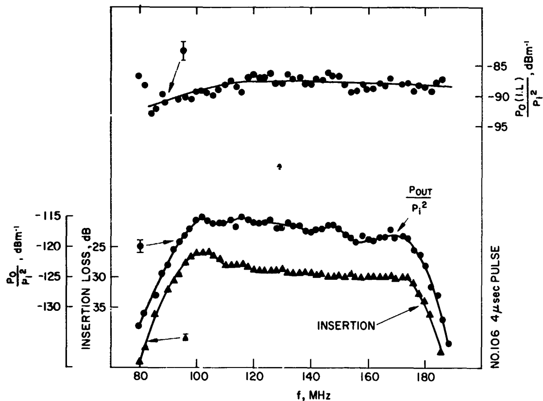
Fig. 28. Measured Performance of 95 to 180 MHz Broadband Convolver.
