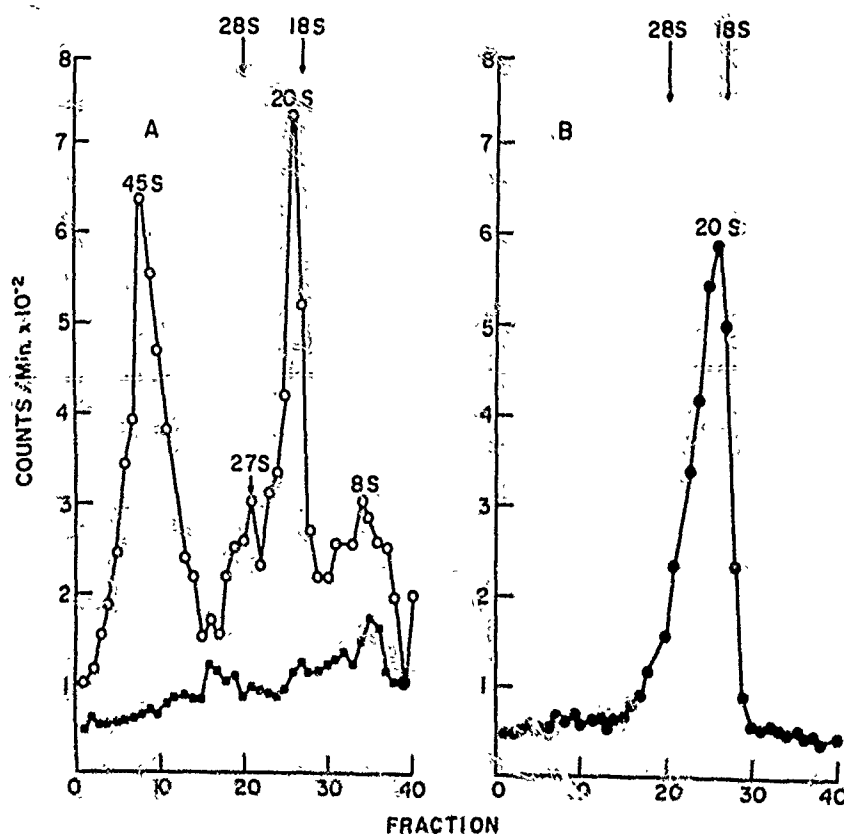
Fig. 4. Sedimentation profile of RNA extracted from CMC fraction derived from PS(X-15) cells infected with JEV. JEV infected and control uninfected cells pretreated with 1 \mu g/ml AD were incubated at 35 °C for 2 days. Cells were pulse labeled with 5 \mu Ci 3 H-5-uridine for 2 hours. CMC fraction RNA isolated and analyzed as described in Materials and Methods.
