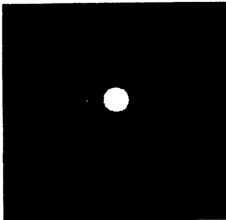
Fig. 3 1 \times 10^{14} N^+ Ions/cm 2 . Diffraction pattern shows some randomly oriented quartz due to recrystallization of amorphous material at 578°C.
