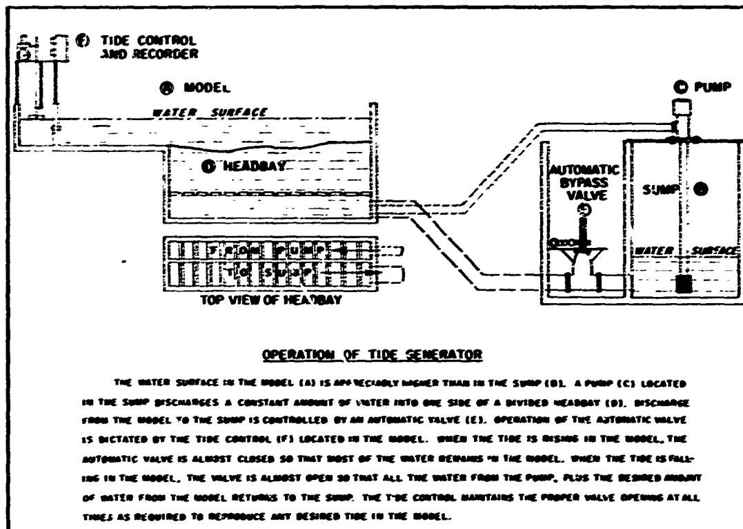
Fig. 5. Schematic diagram of tide generation system
