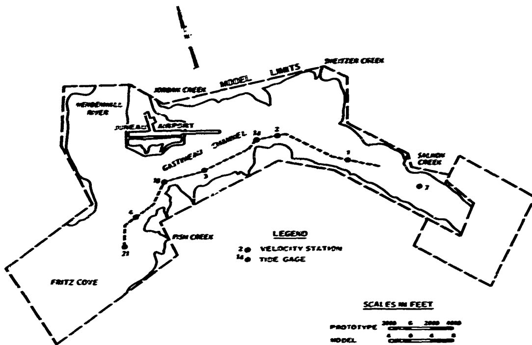
Fig. 3. Model layout
