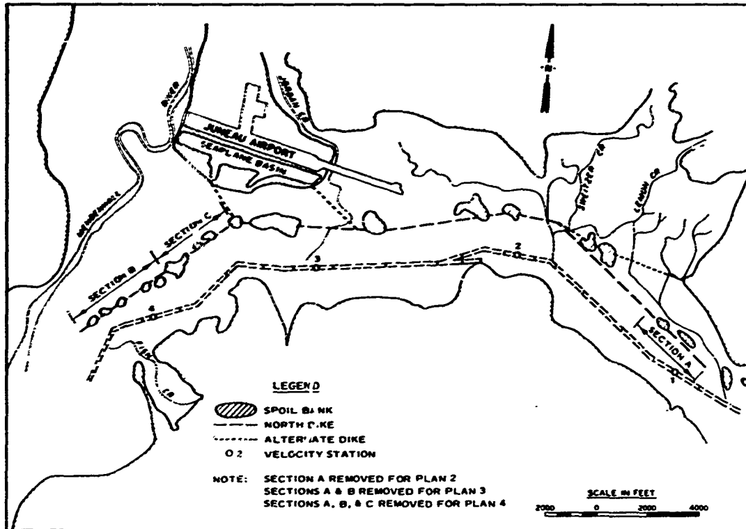
Fig. 12. Elements of proposed north dike plans 1-4
