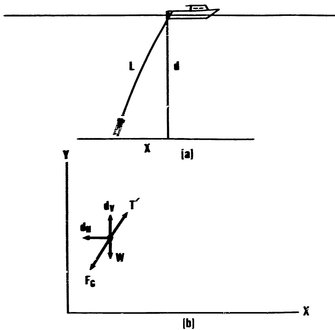
Fig. 63. Forces on unit element of EEA wire rope.
