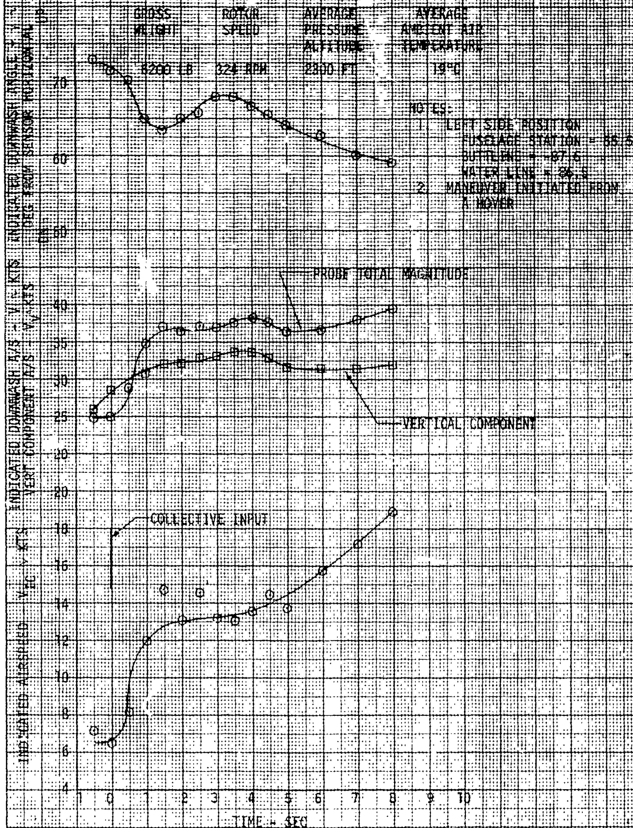
FIGURE 11 AIRSPEED SYSTEM PERFORMANCE DURING A VERTICAL CLIMB EVALUATE LOW AIRSPEED SENSING AND INDICATING EQUIPMENT ON-10
